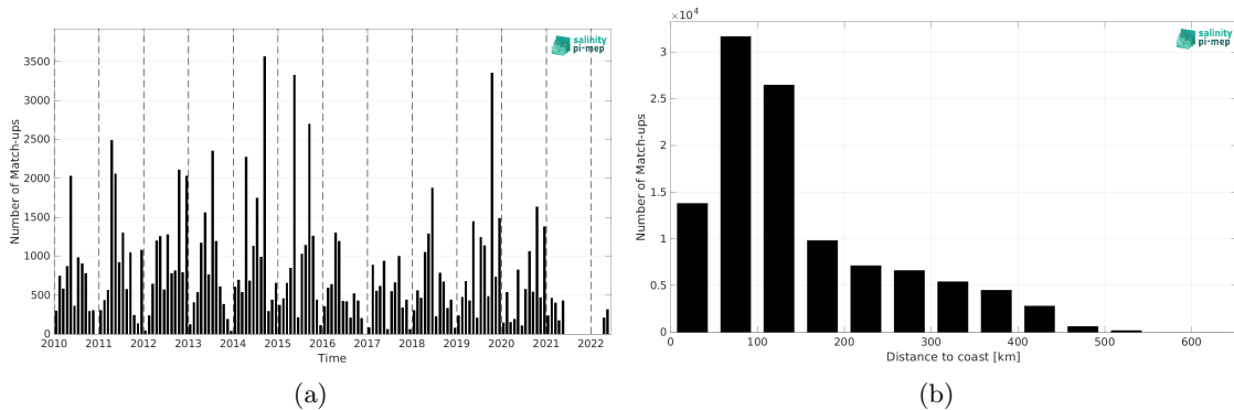
Figure 1: Number of match-ups between ICES and SMOS SSS L3 v9 - 9 Days (CATDS-CEC-LOCEAN) SSS as a function of time (a) and as function of the distance to coast (b) over the Arctic Ocean Pi-MEP region and for the full satellite product period.
