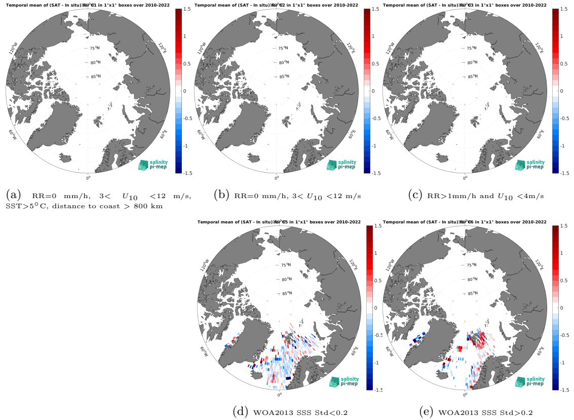
Figure 12: Temporal mean gridded over spatial boxes of size 1^{\circ}\times 1^{\circ} of \Delta\text{SSS} (SMOS SSS L3 v9 - 9 Days (CATDS-CEC-LOCEAN) - ICES) for 5 different subdatasets corresponding to:RR=0 mm/h, 3 < U_{10} < 12 m/s, SST > 5^{\circ}\text{C} , distance to coast > 800 km (a), RR=0 mm/h, 3 < U_{10} < 12 m/s (b), RR > 1 mm/h and U_{10} < 4 m/s (c), WOA2013 SSS Std < 0.2 (d), WOA2013 SSS Std > 0.2 (e).
