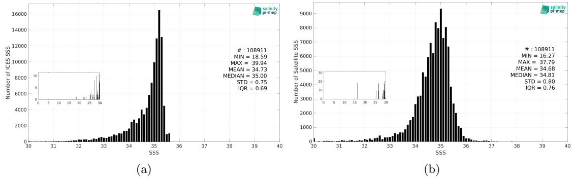
Figure 2: Histograms of SSS from ICES (a) and SMOS SSS L3 v9 - 9 Days (CATDS-CEC-LOCEAN) (b) considering all match-up pairs per bins of 0.1 over the Arctic Ocean Pi-MEP region and for the full satellite product period.
