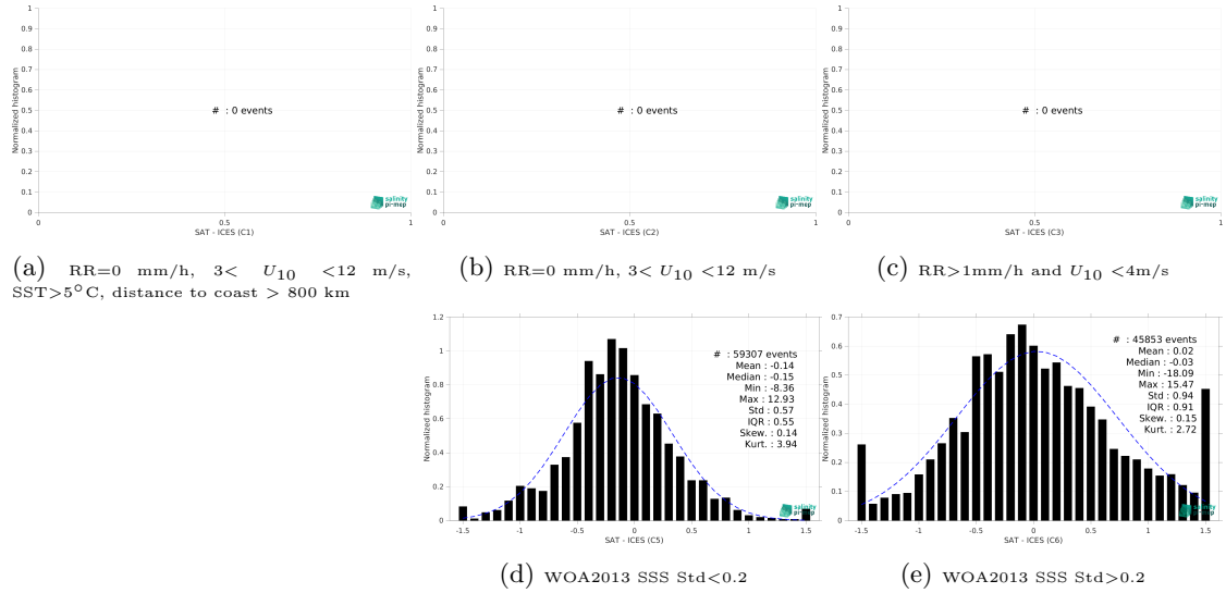
Figure 13: Normalized histogram of \Delta SSS (SMOS SSS L3 v9 - 9 Days (CATDS-CEC-LOCEAN) - ICES) for 5 different subdatasets corresponding to: RR=0 mm/h, 3 < U_{10} < 12 m/s, SST > 5°C, distance to coast > 800 km (a), RR=0 mm/h, 3 < U_{10} < 12 m/s (b), RR > 1mm/h and U_{10} < 4 m/s (c), WOA2013 SSS Std < 0.2 (d), WOA2013 SSS Std > 0.2 (e).
