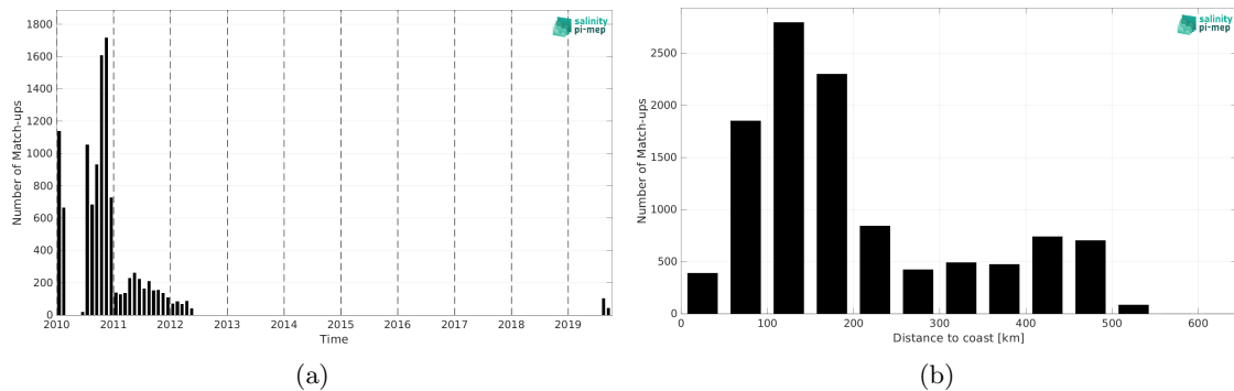
Figure 1: Number of match-ups between Surface drifters and SMOS SSS L3 v9 - 9 Days (CATDS-CEC-LOCEAN) SSS as a function of time (a) and as function of the distance to coast (b) over the Arctic Ocean Pi-MEP region and for the full satellite product period.
