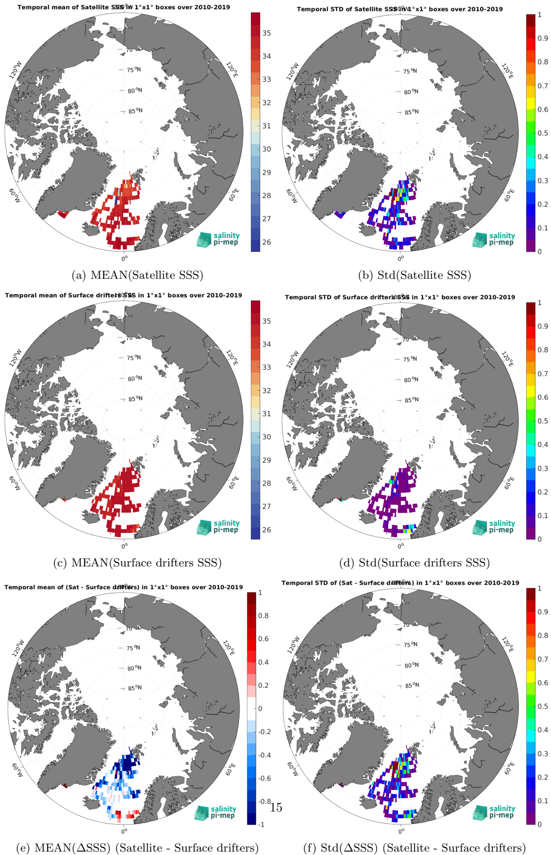
Figure 5: Temporal mean (left) and Std (right) of SSS from SMOS SSS L3 v9 - 9 Days (CATDS-CEC-LOCEAN) (top), Surface drifters (middle), and of \Delta SSS (Satellite - Surface drifters). Only match-up pairs are used to generate these maps.
