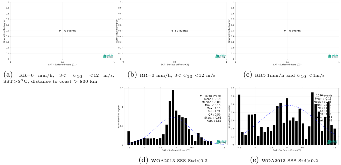
Figure 12: Normalized histogram of \Delta SSS (SMOS SSS L3 v9 - 9 Days (CATDS-CEC-LOCEAN) - Surface drifters) for 5 different subdatasets corresponding to: RR=0 mm/h, 3 < U_{10} < 12 m/s, SST>5°C, distance to coast > 800 km (a), RR=0 mm/h, 3 < U_{10} < 12 m/s (b), RR>1mm/h and U_{10} < 4 m/s (c), WOA2013 SSS Std<0.2 (d), WOA2013 SSS Std>0.2 (e).
