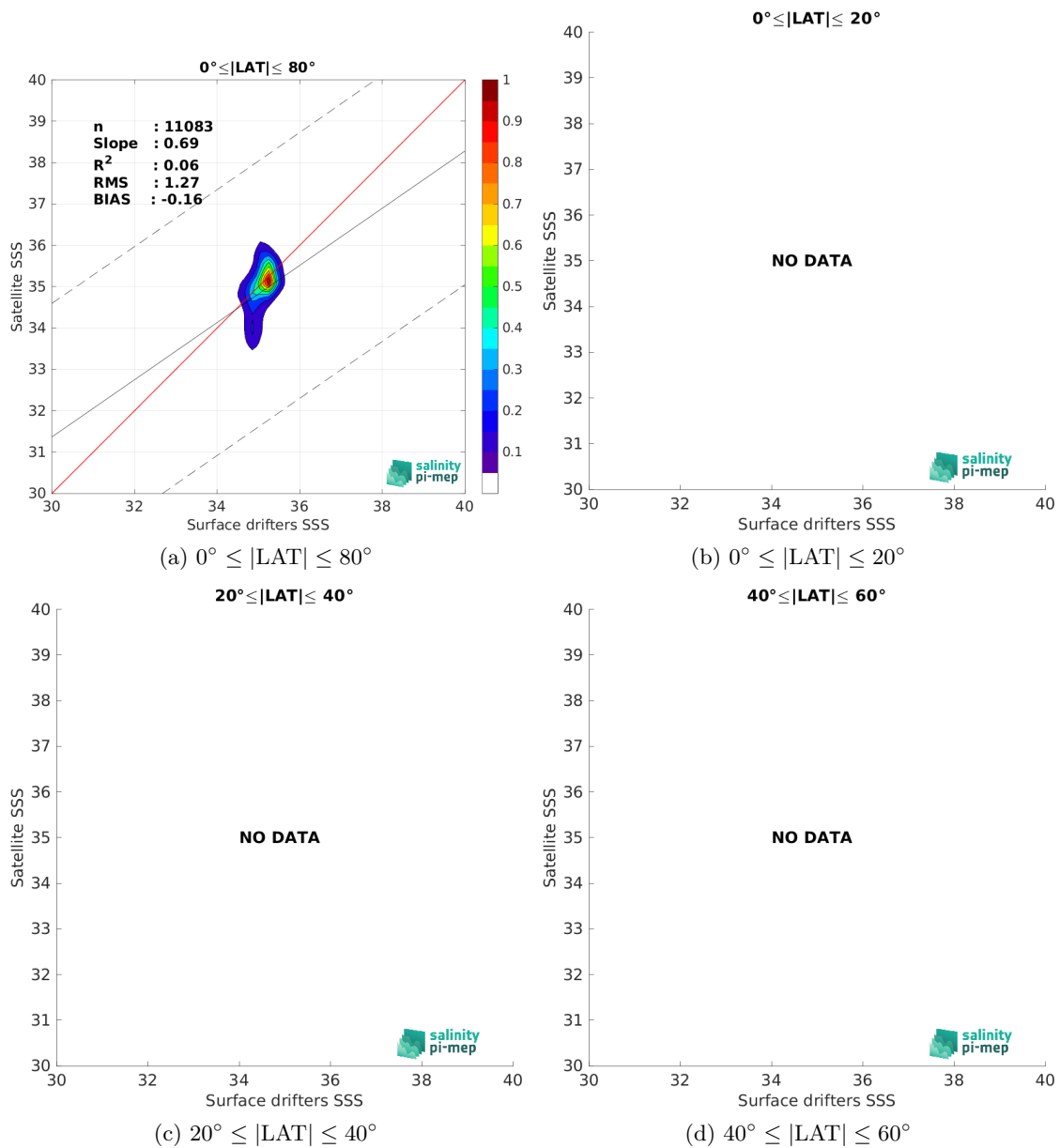
Figure 8: Contour maps of the concentration of SMOS SSS L3 v9 - 9 Days (CATDS-CEC-LOCEAN) SSS (y-axis) versus Surface drifters SSS (x-axis) at match-up pairs for different latitude bands. For each plot, the red line shows x=y . The black thin and dashed lines indicate a linear fit through the data cloud and the \pm 95\% confidence levels, respectively. The number match-up pairs n , the slope and R^2 coefficient of the linear fit, the root mean square (RMS) and the mean bias between satellite and in situ data are indicated for each latitude band in each plots.
