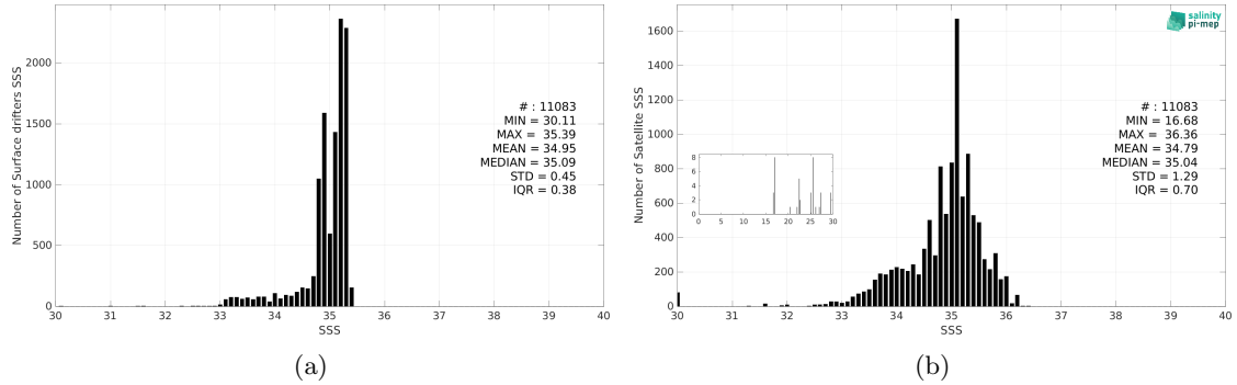
Figure 2: Histograms of SSS from Surface drifters (a) and SMOS SSS L3 v9 - 9 Days (CATDS-CEC-LOCEAN) (b) considering all match-up pairs per bins of 0.1 over the Arctic Ocean Pi-MEP region and for the full satellite product period.
