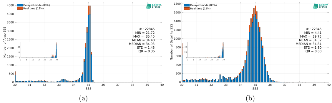
Figure 3: Histograms of SSS from Argo (a) and SMOS SSS L3 v9 - 9 Days (CATDS-CEC-LOCEAN) (b) considering all match-up pairs per bins of 0.1 over the Arctic Ocean Pi-MEP region and for the full satellite product period.
