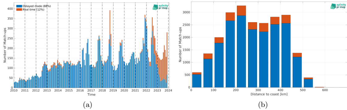
Figure 2: Number of match-ups between Argo and SMOS SSS L3 v9 - 9 Days (CATDS-CEC-LOCEAN) SSS as a function of time (a) and as function of the distance to coast (b) over the Arctic Ocean Pi-MEP region and for the full satellite product period.
