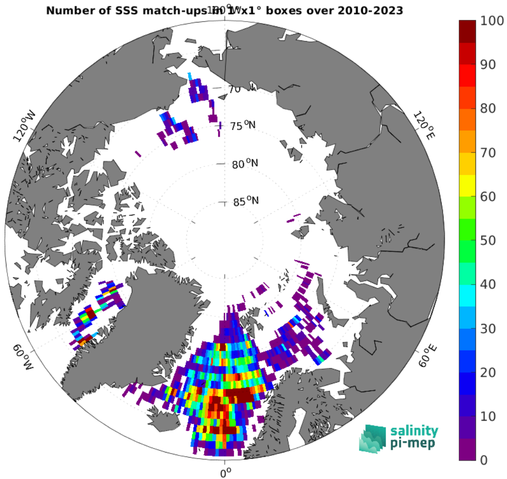
Figure 5: Number of SSS match-ups between Argo SSS and the SMOS SSS L3 v9 - 9 Days (CATDS-CEC-LOCEAN) SSS product for the Arctic Ocean Pi-MEP region over 1^\circ \times 1^\circ boxes and for the full satellite product period.
