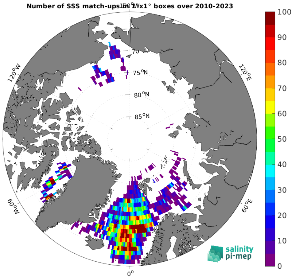
Figure 4: Number of SSS match-ups between Argo SSS and the SMOS SSS L3 v9 - 9 Days (CATDS-CEC-LOCEAN) SSS product for the Arctic Ocean Pi-MEP region over 1^\circ \times 1^\circ boxes and for the full satellite product period.
