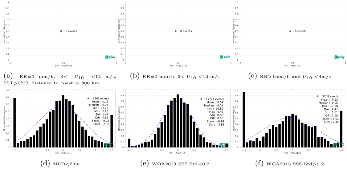
Figure 13: Normalized histogram of \Delta\text{SSS} (SMOS SSS L3 v9 - 9 Days (CATDS-CEC-LOCEAN) - Argo) for 6 different subdatasets corresponding to: RR=0 mm/h, 3 < U_{10} < 12 m/s, SST > 5^{\circ}\text{C} , distance to coast > 800 km (a), RR=0 mm/h, 3 < U_{10} < 12 m/s (b), RR > 1\text{mm/h} and U_{10} < 4\text{m/s} (c), MLD < 20\text{m} (d), WOA2013 SSS Std < 0.2 (e), WOA2013 SSS Std > 0.2 (f).
