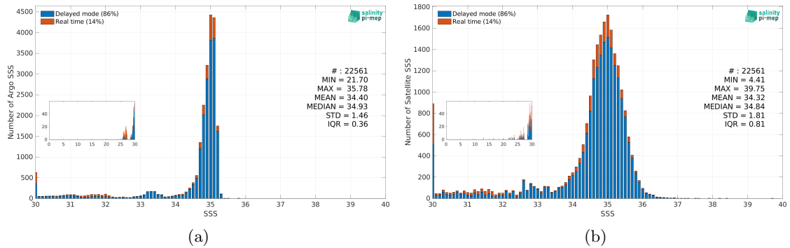
Figure 2: Histograms of SSS from Argo (a) and SMOS SSS L3 v9 - 9 Days (CATDS-CEC-LOCEAN) (b) considering all match-up pairs per bins of 0.1 over the Arctic Ocean Pi-MEP region and for the full satellite product period.
