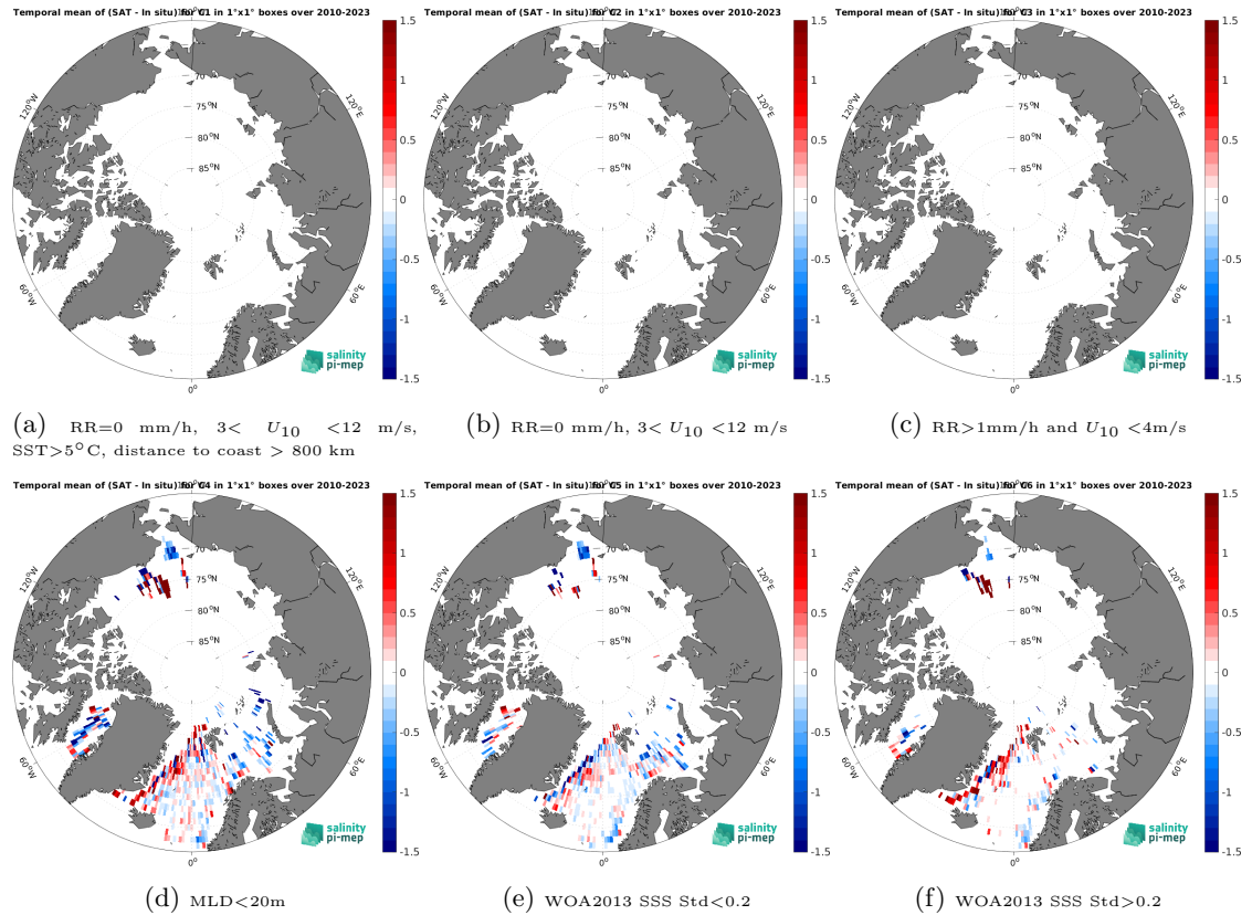
Figure 12: Temporal mean gridded over spatial boxes of size 1^{\circ}\times 1^{\circ} of \Delta\text{SSS} (SMOS SSS L3 v9 - 9 Days (CATDS-CEC-LOCEAN) - Argo) for 6 different subdatasets corresponding to:RR=0 mm/h, 3 < U_{10} < 12 m/s, SST >5^{\circ}\text{C} , distance to coast > 800 km (a), RR=0 mm/h, 3 < U_{10} < 12 m/s (b), RR >1\text{mm/h} and U_{10} < 4\text{m/s} (c),MLD <20\text{m} (d),WOA2013 SSS Std <0.2 (e),WOA2013 SSS Std >0.2 (f).
