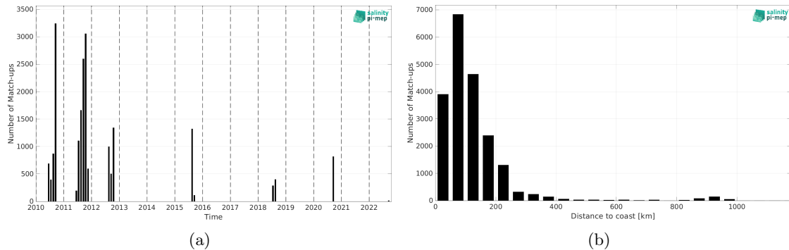
Figure 2: Number of match-ups between TSG (SAMOS) and SMOS SSS L3 v9 - 18 Days (CATDS-CEC-LOCEAN) SSS as a function of time (a) and as function of the distance to coast (b) over the Arctic Ocean Pi-MEP region and for the full satellite product period.
