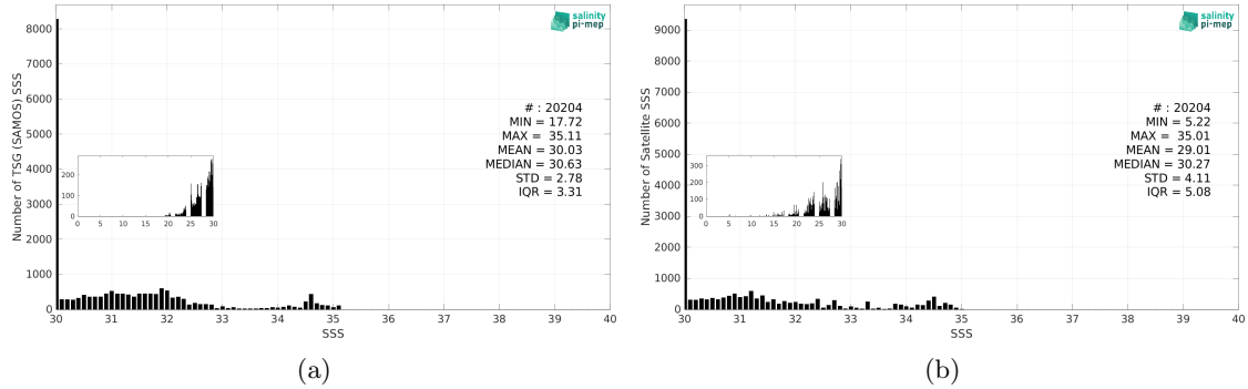
Figure 3: Histograms of SSS from TSG (SAMOS) (a) and SMOS SSS L3 v9 - 18 Days (CATDS-CEC-LOCEAN) (b) considering all match-up pairs per bins of 0.1 over the Arctic Ocean Pi-MEP region and for the full satellite product period.
