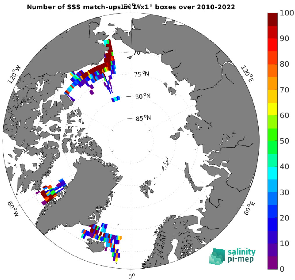
Figure 5: Number of SSS match-ups between TSG (SAMOS) SSS and the SMOS SSS L3 v9 - 18 Days (CATDS-CEC-LOCEAN) SSS product for the Arctic Ocean Pi-MEP region over 1^\circ \times 1^\circ boxes and for the full satellite product period.
