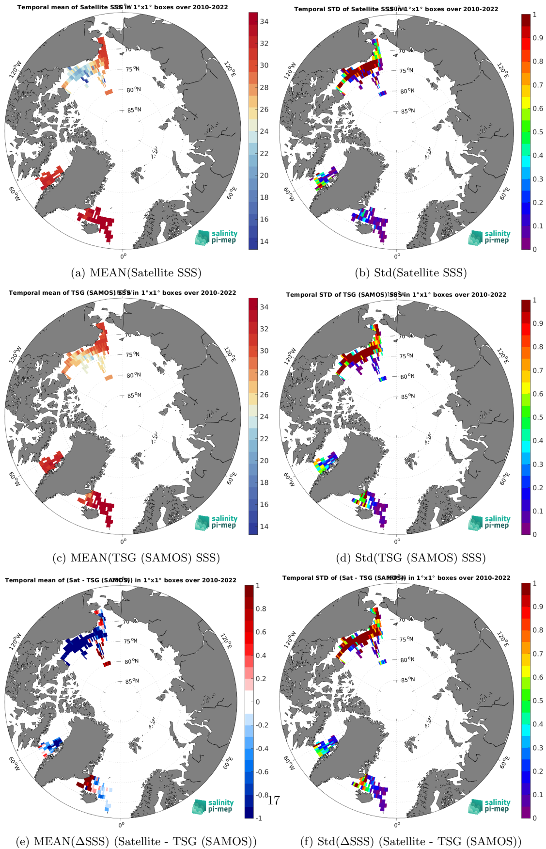
Figure 7: Temporal mean (left) and Std (right) of SSS from SMOS SSS L3 v9 - 18 Days (CATDS-CEC-LOCEAN) (top), TSG (SAMOS) (middle), and of \Delta SSS (Satellite - TSG (SAMOS)). Only match-up pairs are used to generate these maps.
