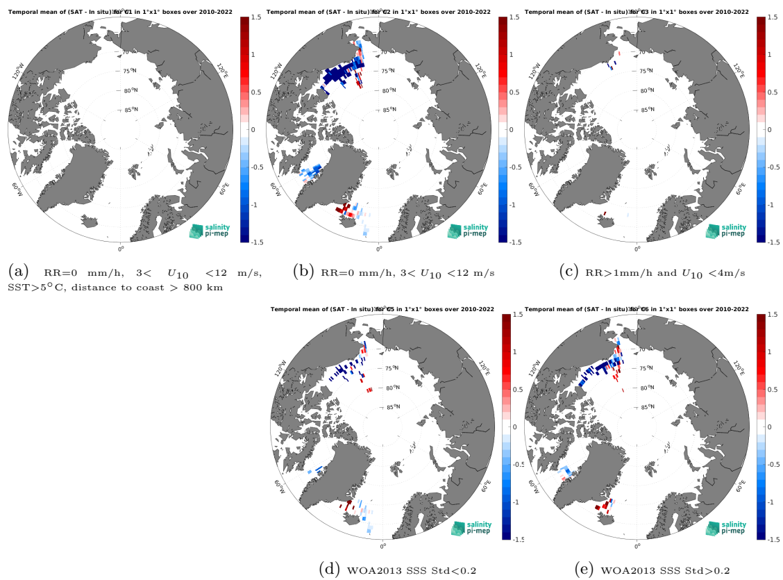
Figure 14: Temporal mean gridded over spatial boxes of size 1^\circ \times 1^\circ of \Delta\text{SSS} (SMOS SSS L3 v9 - 18 Days (CATDS-CEC-LOCEAN) - TSG (SAMOS)) for 5 different subdatasets corresponding to: RR=0 mm/h, 3 < U_{10} < 12 m/s, SST > 5^\circ\text{C} , distance to coast > 800 km (a), RR=0 mm/h, 3 < U_{10} < 12 m/s (b), RR > 1 mm/h and U_{10} < 4 m/s (c), WOA2013 SSS Std < 0.2 (d), WOA2013 SSS Std > 0.2 (e).
