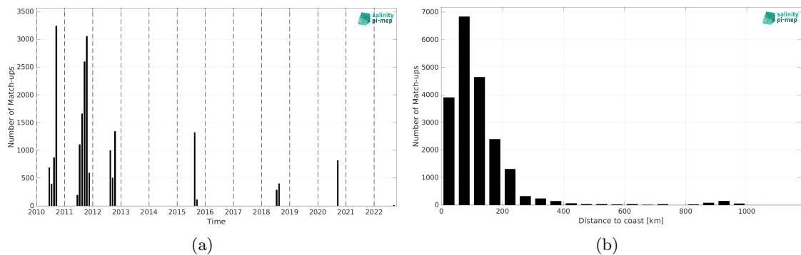
Figure 1: Number of match-ups between TSG (SAMOS) and SMOS SSS L3 v9 - 18 Days (CATDS-CEC-LOCEAN) SSS as a function of time (a) and as function of the distance to coast (b) over the Arctic Ocean Pi-MEP region and for the full satellite product period.
