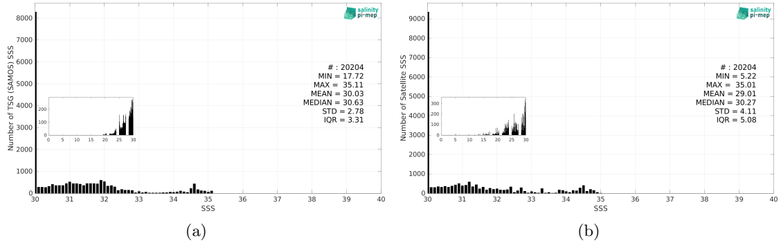
Figure 2: Histograms of SSS from TSG (SAMOS) (a) and SMOS SSS L3 v9 - 18 Days (CATDS-CEC-LOCEAN) (b) considering all match-up pairs per bins of 0.1 over the Arctic Ocean Pi-MEP region and for the full satellite product period.
