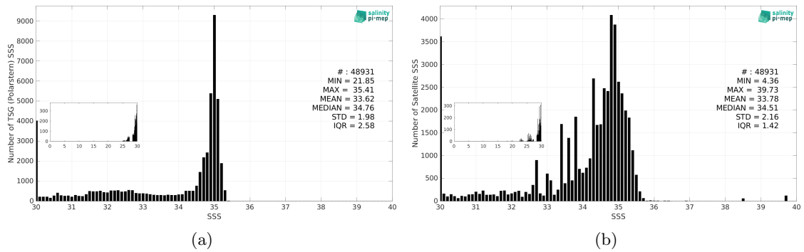
Figure 3: Histograms of SSS from TSG (Polarstern) (a) and SMOS SSS L3 v9 - 18 Days (CATDS-CEC-LOCEAN) (b) considering all match-up pairs per bins of 0.1 over the Arctic Ocean Pi-MEP region and for the full satellite product period.
