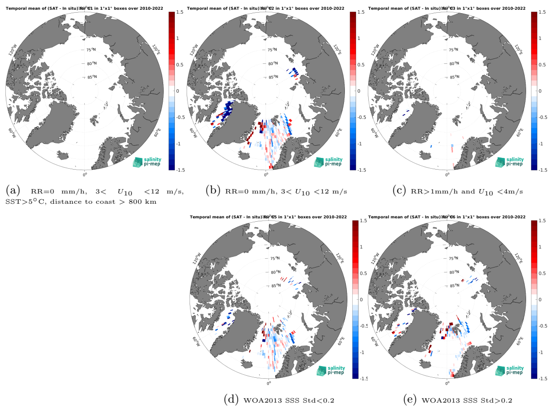
Figure 14: Temporal mean gridded over spatial boxes of size 1^\circ \times 1^\circ of \Delta SSS (SMOS SSS L3 v9 - 18 Days (CATDS-CEC-LOCEAN) - TSG (Polarstern)) for 5 different subdatasets corresponding to:RR=0 mm/h, 3 < U_{10} < 12 m/s, SST >5^\circ\text{C} , distance to coast > 800 km (a), RR=0 mm/h, 3 < U_{10} < 12 m/s (b), RR >1 mm/h and U_{10} < 4 m/s (c), WOA2013 SSS Std <0.2 (d), WOA2013 SSS Std >0.2 (e).
