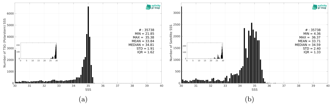
Figure 2: Histograms of SSS from TSG (Polarstern) (a) and SMOS SSS L3 v9 - 18 Days (CATDS-CEC-LOCEAN) (b) considering all match-up pairs per bins of 0.1 over the Arctic Ocean Pi-MEP region and for the full satellite product period.
