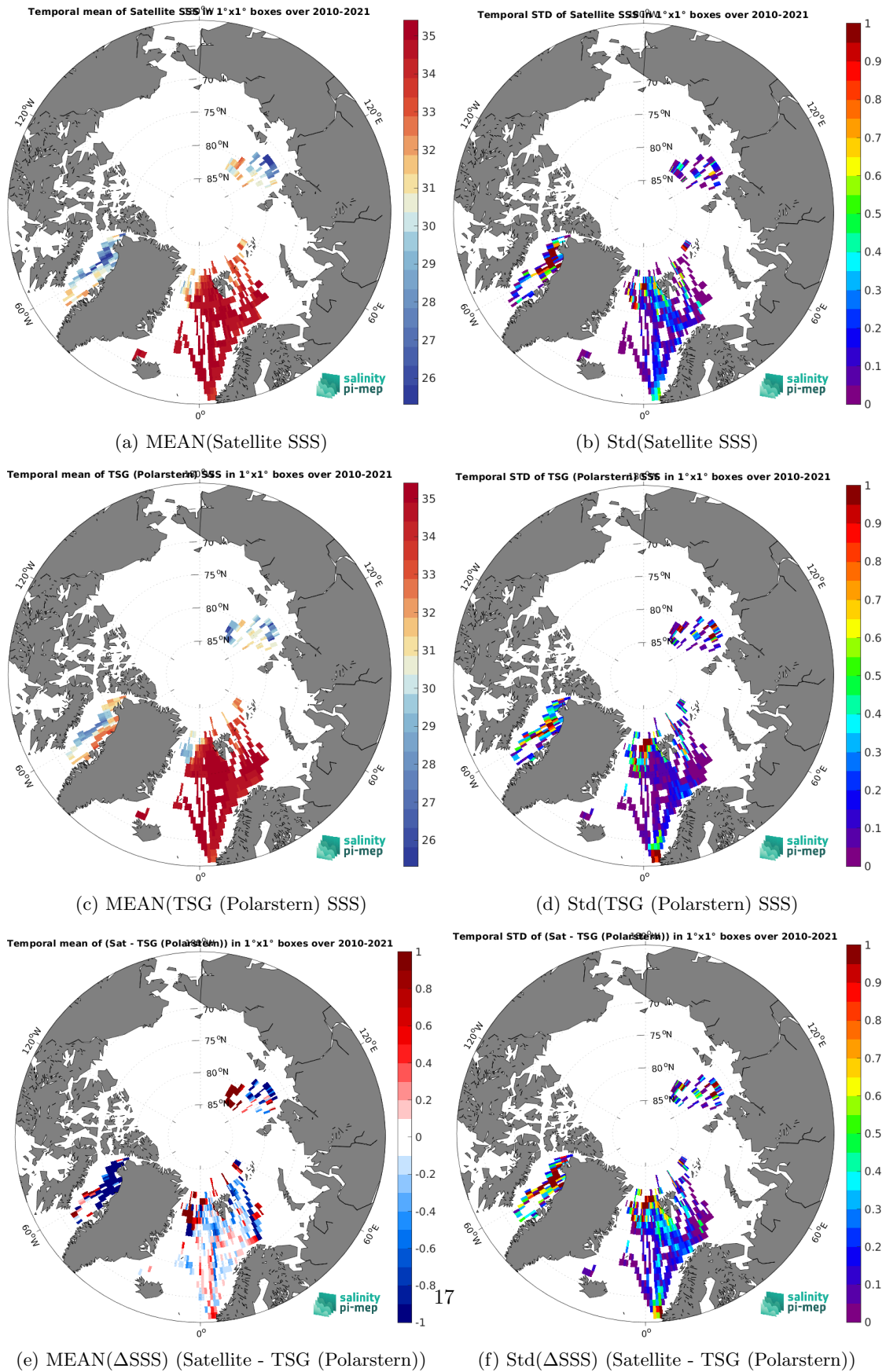
Figure 6: Temporal mean (left) and Std (right) of SSS from SMOS SSS L3 v9 - 18 Days (CATDS-CEC-LOCEAN) (top), TSG (Polarstern) (middle), and of \Delta SSS (Satellite - TSG (Polarstern)). Only match-up pairs are used to generate these maps.
