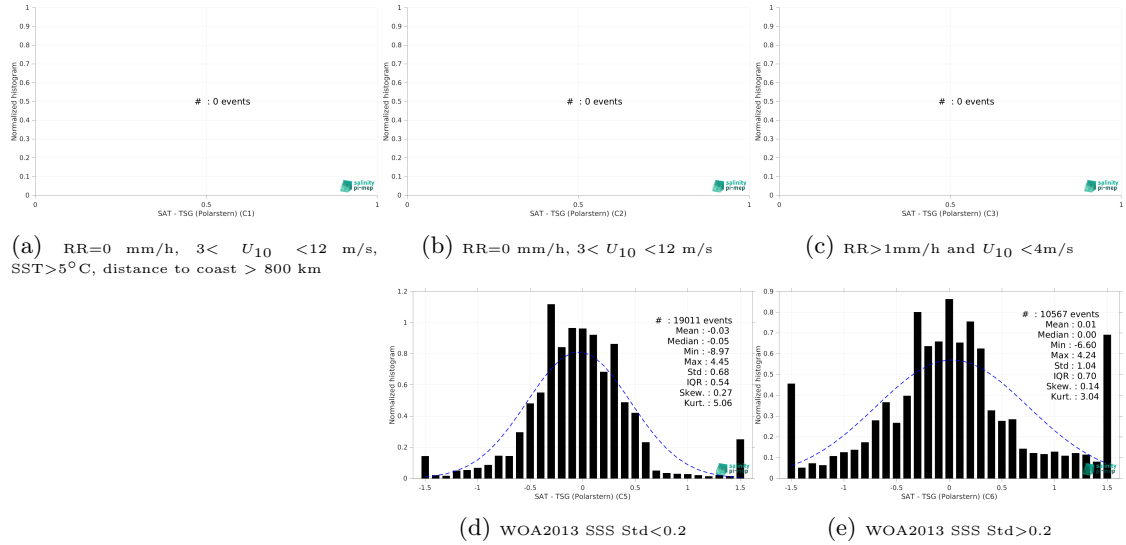
Figure 13: Normalized histogram of \Delta SSS (SMOS SSS L3 v9 - 18 Days (CATDS-CEC-LOCEAN) - TSG (Polarstern)) for 5 different subdatasets corresponding to: RR=0 mm/h, 3 < U_{10} < 12 m/s, SST>5°C, distance to coast > 800 km (a), RR=0 mm/h, 3 < U_{10} < 12 m/s (b), RR>1mm/h and U_{10} < 4 m/s (c), WOA2013 SSS Std<0.2 (d), WOA2013 SSS Std>0.2 (e).
