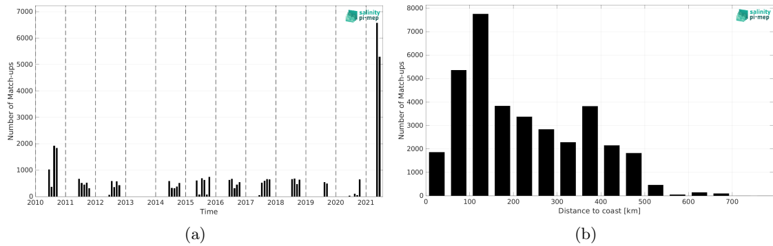
Figure 1: Number of match-ups between TSG (Polarstern) and SMOS SSS L3 v9 - 18 Days (CATDS-CEC-LOCEAN) SSS as a function of time (a) and as function of the distance to coast (b) over the Arctic Ocean Pi-MEP region and for the full satellite product period.
