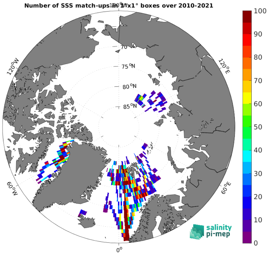
Figure 4: Number of SSS match-ups between TSG (Polarstern) SSS and the SMOS SSS L3 v9 - 18 Days (CATDS-CEC-LOCEAN) SSS product for the Arctic Ocean Pi-MEP region over 1^\circ \times 1^\circ boxes and for the full satellite product period.
