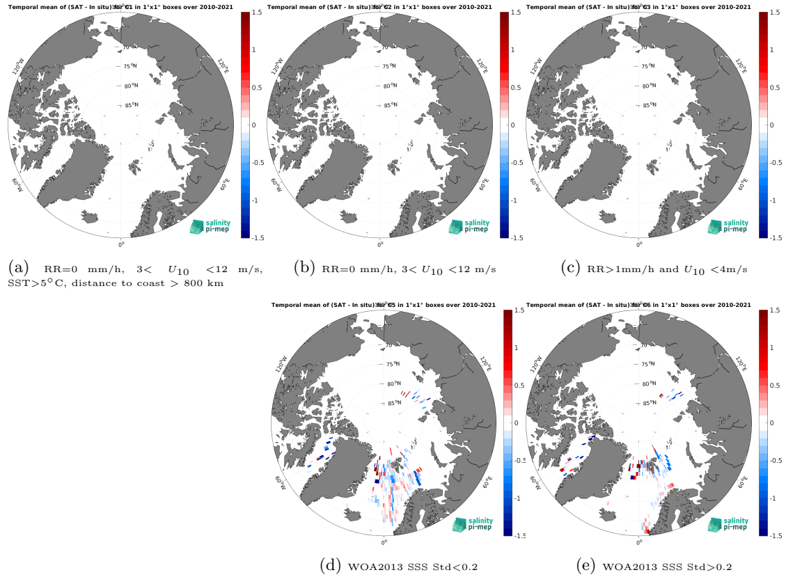
Figure 12: Temporal mean gridded over spatial boxes of size 1^{\circ}\times 1^{\circ} of \Delta\text{SSS} (SMOS SSS L3 v9 - 18 Days (CATDS-CEC-LOCEAN) - TSG (Polarstern)) for 5 different subdatasets corresponding to: RR=0 mm/h, 3 < U_{10} < 12 m/s, SST >5^{\circ}\text{C} , distance to coast > 800 km (a), RR=0 mm/h, 3 < U_{10} < 12 m/s (b), RR >1 mm/h and U_{10} < 4 m/s (c), WOA2013 SSS Std <0.2 (d), WOA2013 SSS Std >0.2 (e).
