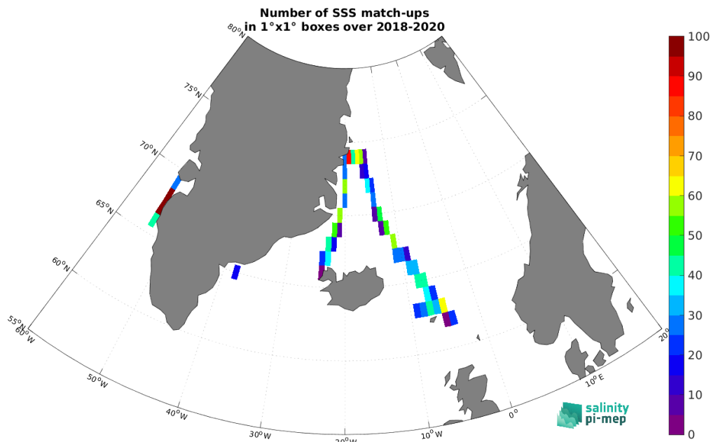
Figure 5: Number of SSS match-ups between TSG (Lauge-Koch) SSS and the SMOS SSS L3 v9 - 18 Days (CATDS-CEC-LOCEAN) SSS product for the Arctic Ocean Pi-MEP region over 1^\circ \times 1^\circ boxes and for the full satellite product period.
