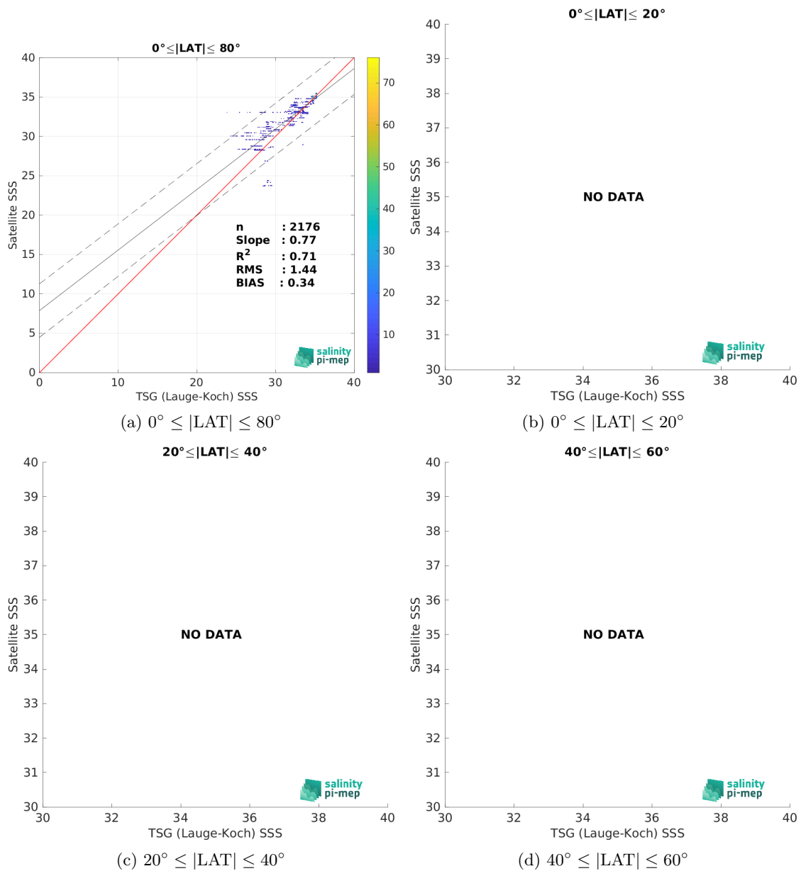
Figure 10: Contour maps of the concentration of SMOS SSS L3 v9 - 18 Days (CATDS-CEC-LOCEAN) SSS (y-axis) versus TSG (Lauge-Koch) SSS (x-axis) at match-up pairs for different latitude bands. For each plot, the red line shows x=y . The black thin and dashed lines indicate a linear fit through the data cloud and the \pm 95\% confidence levels, respectively. The number match-up pairs n , the slope and R^2 coefficient of the linear fit, the root mean square (RMS) and the mean bias between satellite and in situ data are indicated for each latitude band in each plots.
