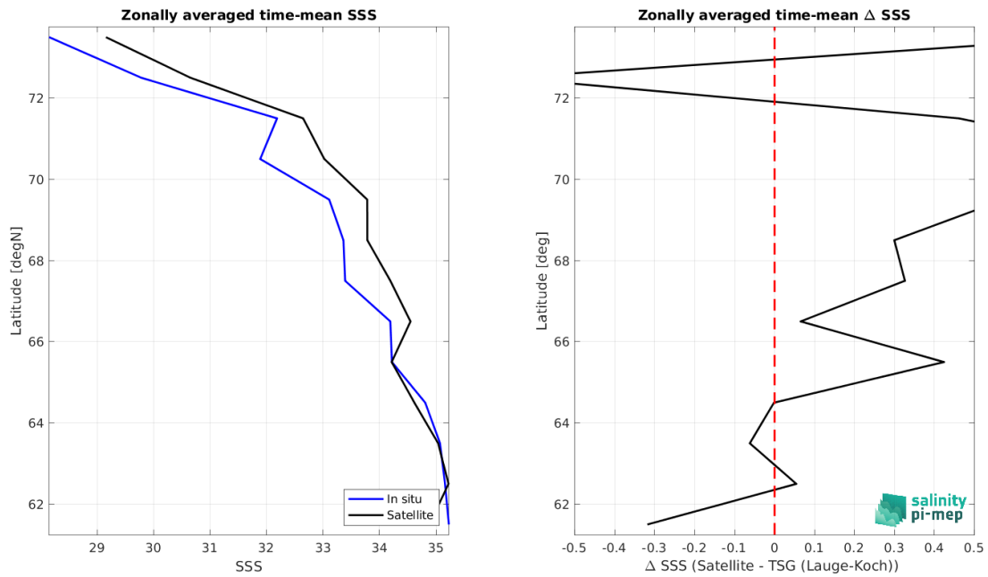
Figure 9: Left panel: Zonal mean SSS from SMOS SSS L3 v9 - 18 Days (CATDS-CEC-LOCEAN) satellite product (black) and from TSG (Lauge-Koch) (blue). Right panel: Zonal mean of \Delta SSS (Satellite - TSG (Lauge-Koch)) for all the collected Pi-MEP match-up pairs estimated over the full satellite product period.
