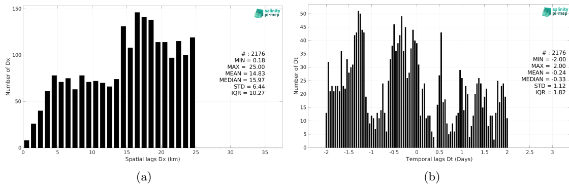
Figure 6: Histograms of the spatial (a) and temporal (b) lags between the location/time of the TSG (Lauge-Koch) measurement and the date of the corresponding SMOS SSS L3 v9 - 18 Days (CATDS-CEC-LOCEAN) SSS pixel.
