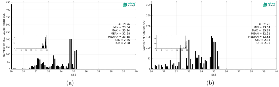
Figure 3: Histograms of SSS from TSG (Lauge-Koch) (a) and SMOS SSS L3 v9 - 18 Days (CATDS-CEC-LOCEAN) (b) considering all match-up pairs per bins of 0.1 over the Arctic Ocean Pi-MEP region and for the full satellite product period.
