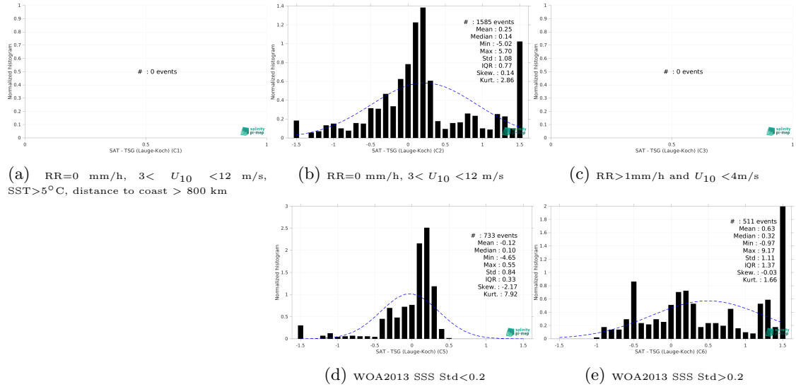
Figure 15: Normalized histogram of \Delta SSS (SMOS SSS L3 v9 - 18 Days (CATDS-CEC-LOCEAN) - TSG (Lauge-Koch)) for 5 different subdatasets corresponding to: RR=0 mm/h, 3 < U_{10} < 12 m/s, SST > 5°C, distance to coast > 800 km (a), RR=0 mm/h, 3 < U_{10} < 12 m/s (b), RR > 1mm/h and U_{10} < 4 m/s (c), WOA2013 SSS Std < 0.2 (d), WOA2013 SSS Std > 0.2 (e).
