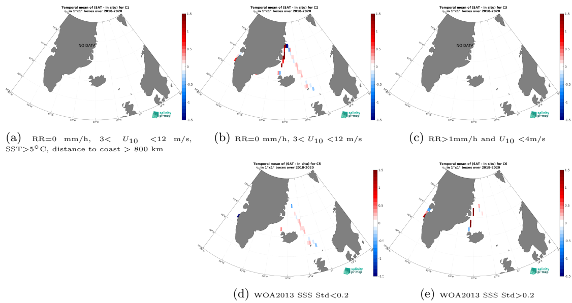
Figure 14: Temporal mean gridded over spatial boxes of size 1^\circ \times 1^\circ of \Delta SSS (SMOS SSS L3 v9 - 18 Days (CATDS-CEC-LOCEAN) - TSG (Lauge-Koch)) for 5 different subdatasets corresponding to:RR=0 mm/h, 3 < U_{10} < 12 m/s, SST > 5^\circ\text{C} , distance to coast > 800 km (a), RR=0 mm/h, 3 < U_{10} < 12 m/s (b), RR > 1 mm/h and U_{10} < 4 m/s (c), WOA2013 SSS Std < 0.2 (d), WOA2013 SSS Std > 0.2 (e).
