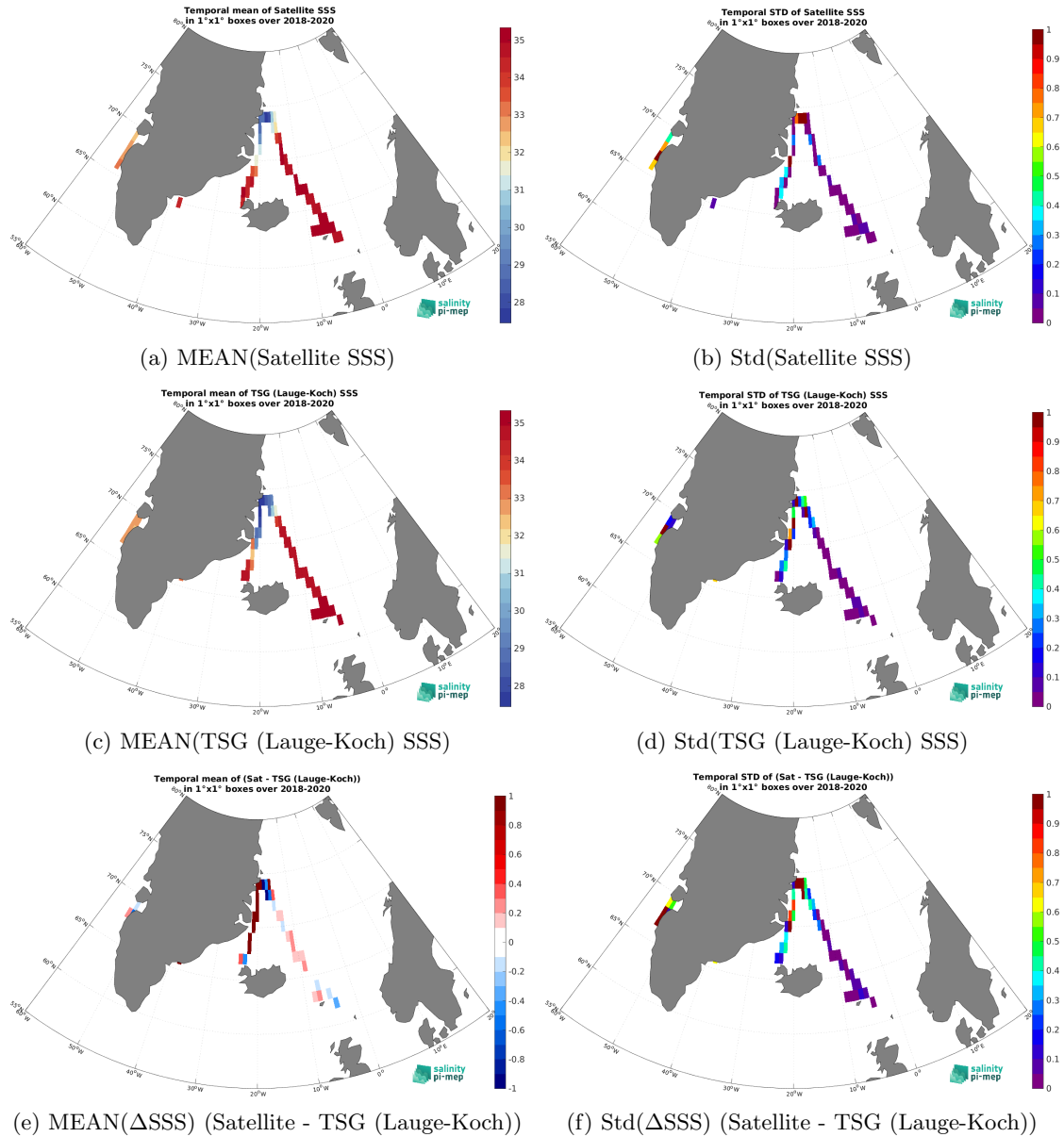
Figure 7: Temporal mean (left) and Std (right) of SSS from SMOS SSS L3 v9 - 18 Days (CATDS-CEC-LOCEAN) (top), TSG (Lauge-Koch) (middle), and of \Delta SSS (Satellite - TSG (Lauge-Koch)). Only match-up pairs are used to generate these maps.
