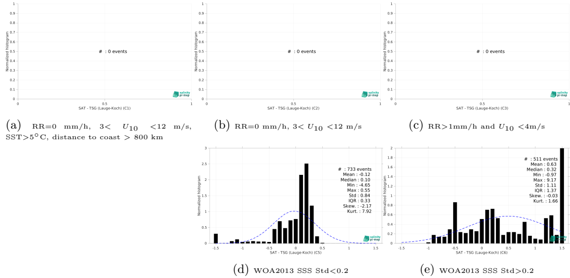
Figure 13: Normalized histogram of \Delta SSS (SMOS SSS L3 v9 - 18 Days (CATDS-CEC-LOCEAN) - TSG (Lauge-Koch)) for 5 different subdatasets corresponding to: RR=0 mm/h, 3 < U_{10} < 12 m/s, SST > 5°C, distance to coast > 800 km (a), RR=0 mm/h, 3 < U_{10} < 12 m/s (b), RR > 1mm/h and U_{10} < 4 m/s (c), WOA2013 SSS Std < 0.2 (d), WOA2013 SSS Std > 0.2 (e).
