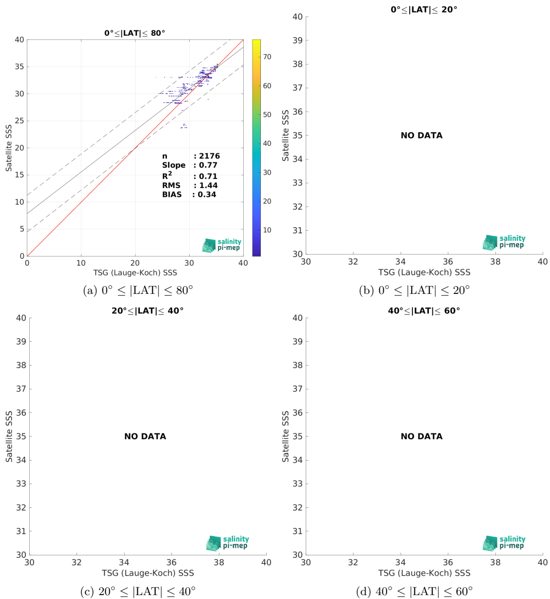
Figure 9: Contour maps of the concentration of SMOS SSS L3 v9 - 18 Days (CATDS-CEC-LOCEAN) SSS (y-axis) versus TSG (Lauge-Koch) SSS (x-axis) at match-up pairs for different latitude bands. For each plot, the red line shows x=y . The black thin and dashed lines indicate a linear fit through the data cloud and the \pm 95\% confidence levels, respectively. The number match-up pairs n , the slope and R^2 coefficient of the linear fit, the root mean square (RMS) and the mean bias between satellite and in situ data are indicated for each latitude band in each plots.
