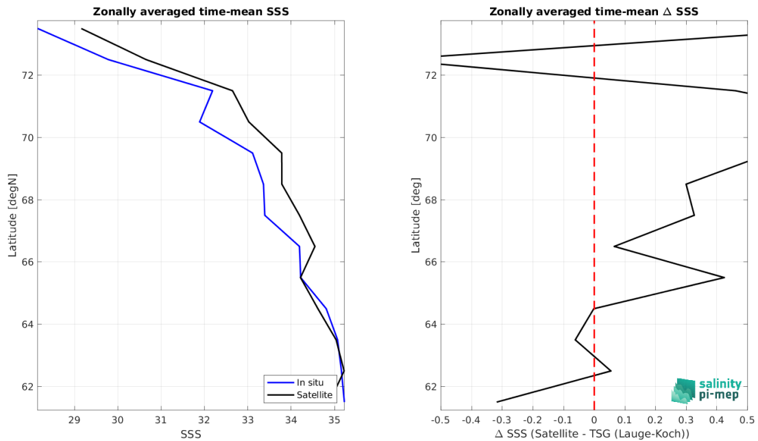
Figure 8: Left panel: Zonal mean SSS from SMOS SSS L3 v9 - 18 Days (CATDS-CEC-LOCEAN) satellite product (black) and from TSG (Lauge-Koch) (blue). Right panel: Zonal mean of \Delta SSS (Satellite - TSG (Lauge-Koch)) for all the collected Pi-MEP match-up pairs estimated over the full satellite product period.
