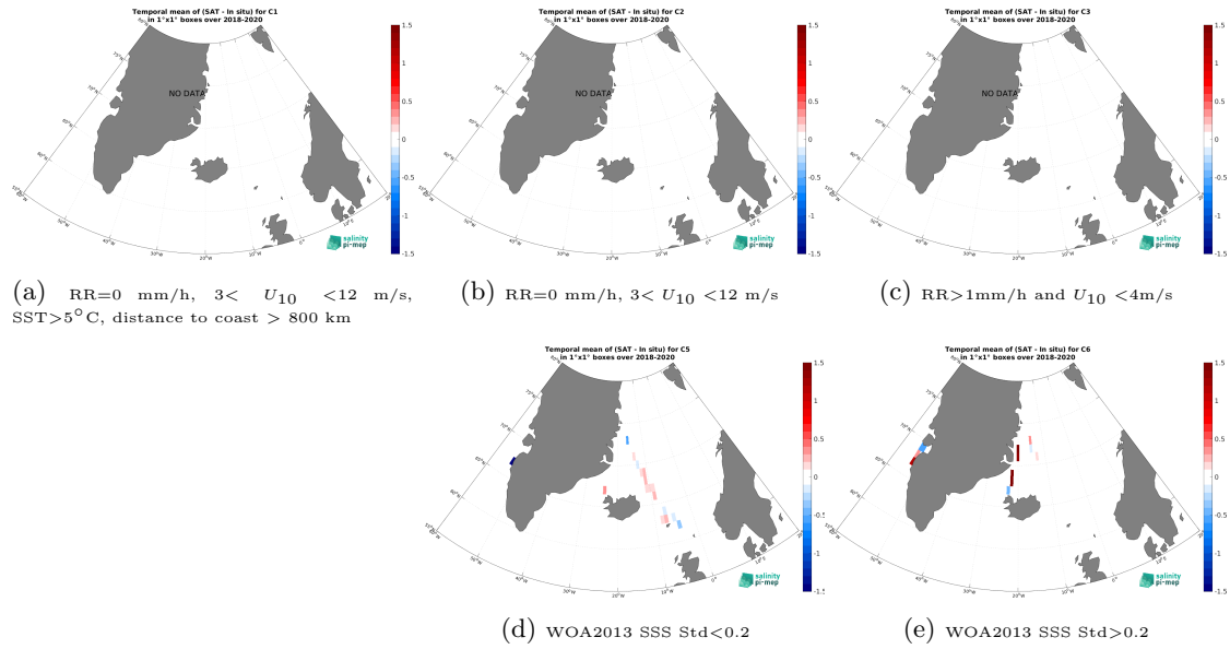
Figure 12: Temporal mean gridded over spatial boxes of size 1^{\circ}\times 1^{\circ} of \Delta\text{SSS} (SMOS SSS L3 v9 - 18 Days (CATDS-CEC-LOCEAN) - TSG (Lauge-Koch)) for 5 different subdatasets corresponding to:RR=0 mm/h, 3 < U_{10} < 12 m/s, SST >5^{\circ}\text{C} , distance to coast > 800 km (a), RR=0 mm/h, 3 < U_{10} < 12 m/s (b), RR >1 mm/h and U_{10} < 4 m/s (c), WOA2013 SSS Std <0.2 (d), WOA2013 SSS Std >0.2 (e).
