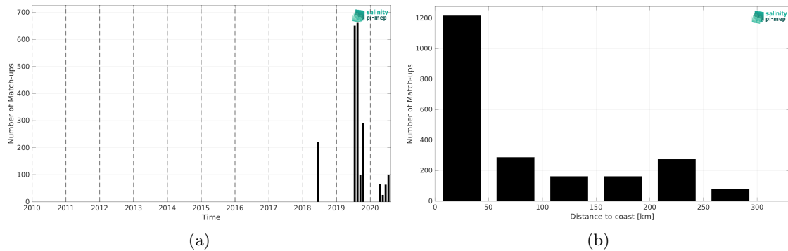
Figure 1: Number of match-ups between TSG (Lauge-Koch) and SMOS SSS L3 v9 - 18 Days (CATDS-CEC-LOCEAN) SSS as a function of time (a) and as function of the distance to coast (b) over the Arctic Ocean Pi-MEP region and for the full satellite product period.
