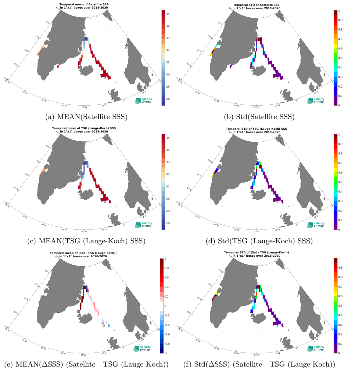
Figure 6: Temporal mean (left) and Std (right) of SSS from SMOS SSS L3 v9 - 18 Days (CATDS-CEC-LOCEAN) (top), TSG (Lauge-Koch) (middle), and of \Delta SSS (Satellite - TSG (Lauge-Koch)). Only match-up pairs are used to generate these maps.
