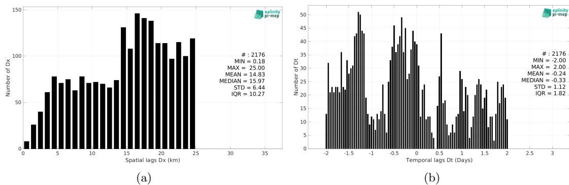
Figure 5: Histograms of the spatial (a) and temporal (b) lags between the location/time of the TSG (Lauge-Koch) measurement and the date of the corresponding SMOS SSS L3 v9 - 18 Days (CATDS-CEC-LOCEAN) SSS pixel.
