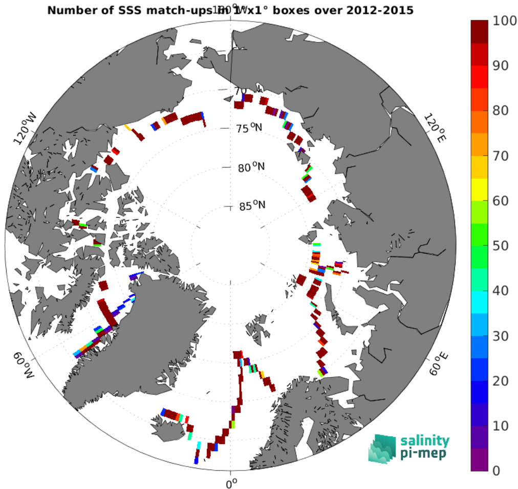
Figure 4: Number of SSS match-ups between TSG (GOSUD-Sailing-ship) SSS and the SMOS SSS L3 v9 - 18 Days (CATDS-CEC-LOCEAN) SSS product for the Arctic Ocean Pi-MEP region over 1^\circ \times 1^\circ boxes and for the full satellite product period.
