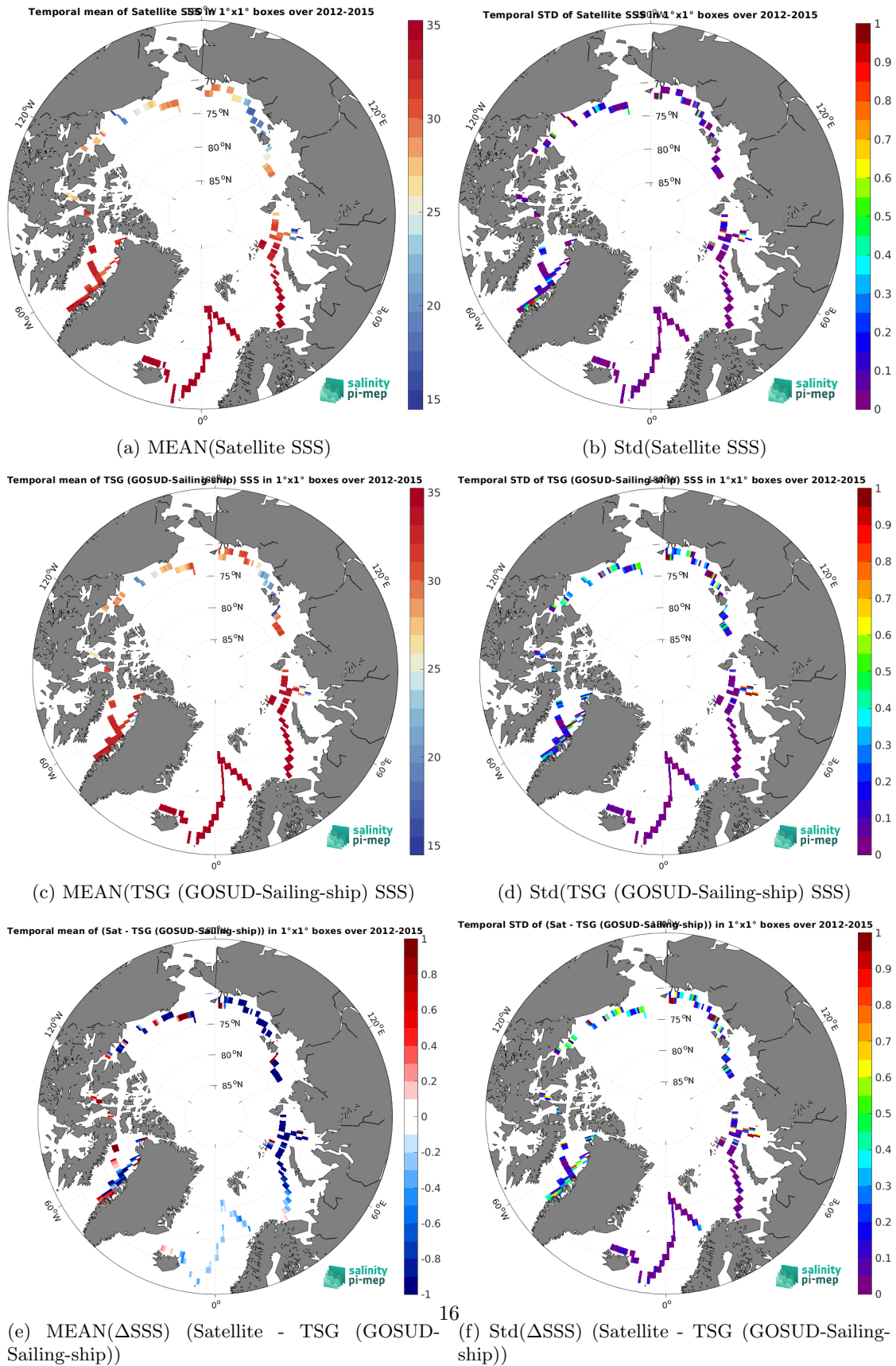
Figure 6: Temporal mean (left) and Std (right) of SSS from SMOS SSS L3 v9 - 18 Days (CATDS-CEC-LOCEAN) (top), TSG (GOSUD-Sailing-ship) (middle), and of \Delta SSS (Satellite - TSG (GOSUD-Sailing-ship)). Only match-up pairs are used to generate these maps.
