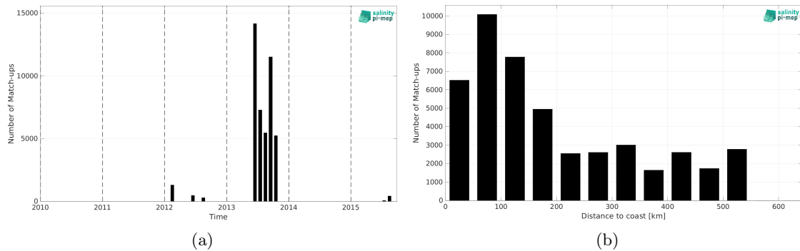
Figure 1: Number of match-ups between TSG (GOSUD-Sailing-ship) and SMOS SSS L3 v9 - 18 Days (CATDS-CEC-LOCEAN) SSS as a function of time (a) and as function of the distance to coast (b) over the Arctic Ocean Pi-MEP region and for the full satellite product period.
