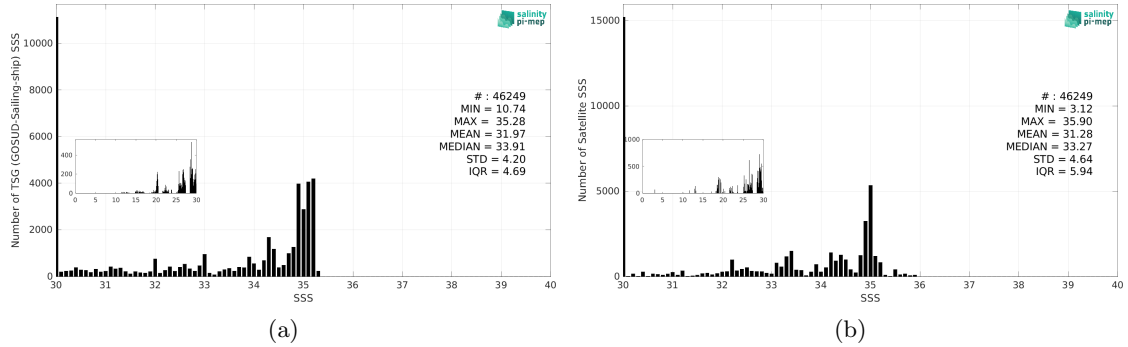
Figure 2: Histograms of SSS from TSG (GOSUD-Sailing-ship) (a) and SMOS SSS L3 v9 - 18 Days (CATDS-CEC-LOCEAN) (b) considering all match-up pairs per bins of 0.1 over the Arctic Ocean Pi-MEP region and for the full satellite product period.
