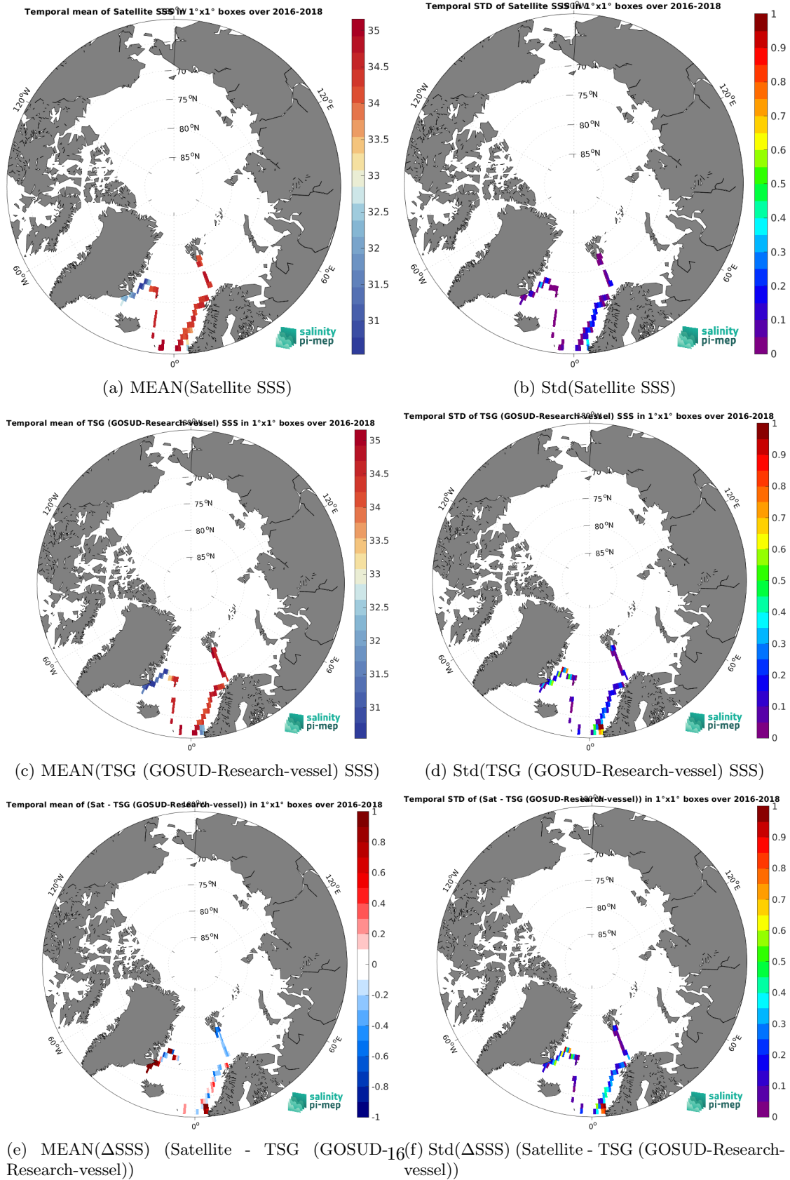
Figure 7: Temporal mean (left) and Std (right) of SSS from SMOS SSS L3 v9 - 18 Days (CATDS-CEC-LOCEAN) (top), TSG (GOSUD-Research-vessel) (middle), and of \Delta SSS (Satellite - TSG (GOSUD-Research-vessel)). Only match-up pairs are used to generate these maps.
