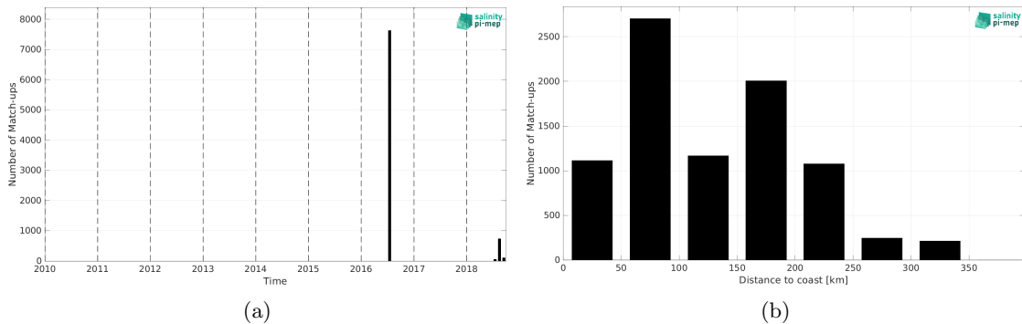
Figure 2: Number of match-ups between TSG (GOSUD-Research-vessel) and SMOS SSS L3 v9 - 18 Days (CATDS-CEC-LOCEAN) SSS as a function of time (a) and as function of the distance to coast (b) over the Arctic Ocean Pi-MEP region and for the full satellite product period.
