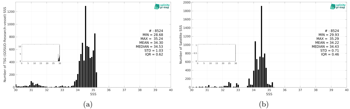
Figure 2: Histograms of SSS from TSG (GOSUD-Research-vessel) (a) and SMOS SSS L3 v9 - 18 Days (CATDS-CEC-LOCEAN) (b) considering all match-up pairs per bins of 0.1 over the Arctic Ocean Pi-MEP region and for the full satellite product period.
