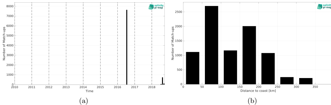
Figure 1: Number of match-ups between TSG (GOSUD-Research-vessel) and SMOS SSS L3 v9 - 18 Days (CATDS-CEC-LOCEAN) SSS as a function of time (a) and as function of the distance to coast (b) over the Arctic Ocean Pi-MEP region and for the full satellite product period.
