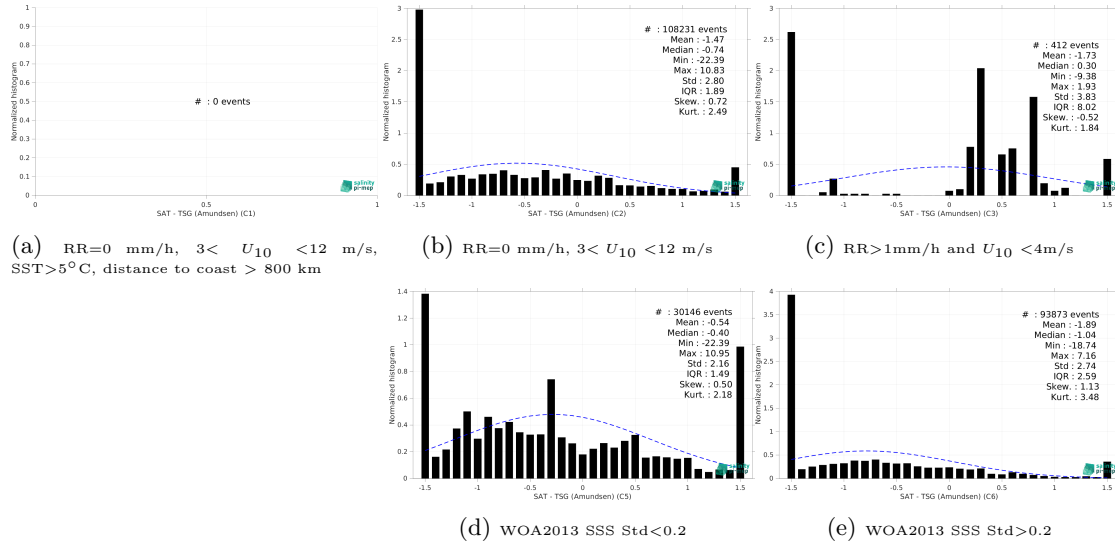
Figure 15: Normalized histogram of \Delta SSS (SMOS SSS L3 v9 - 18 Days (CATDS-CEC-LOCEAN) - TSG (Amundsen)) for 5 different subdatasets corresponding to: RR=0 mm/h, 3 < U_{10} < 12 m/s, SST>5°C, distance to coast > 800 km (a), RR=0 mm/h, 3 < U_{10} < 12 m/s (b), RR>1mm/h and U_{10} < 4 m/s (c), WOA2013 SSS Std<0.2 (d), WOA2013 SSS Std>0.2 (e).
