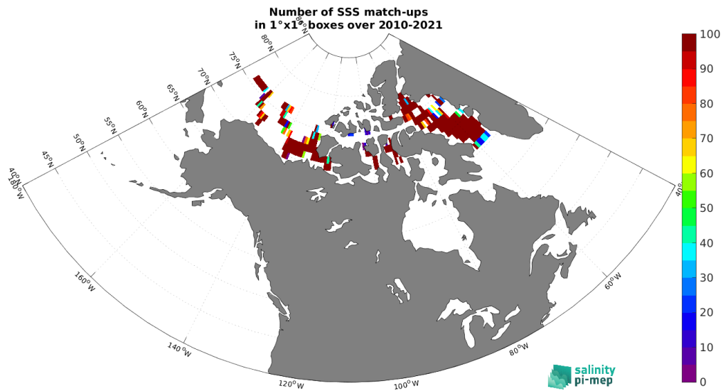
Figure 5: Number of SSS match-ups between TSG (Amundsen) SSS and the SMOS SSS L3 v9 - 18 Days (CATDS-CEC-LOCEAN) SSS product for the Arctic Ocean Pi-MEP region over 1^\circ \times 1^\circ boxes and for the full satellite product period.
