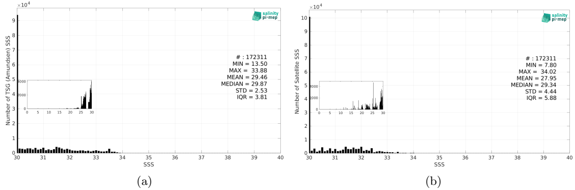
Figure 3: Histograms of SSS from TSG (Amundsen) (a) and SMOS SSS L3 v9 - 18 Days (CATDS-CEC-LOCEAN) (b) considering all match-up pairs per bins of 0.1 over the Arctic Ocean Pi-MEP region and for the full satellite product period.
