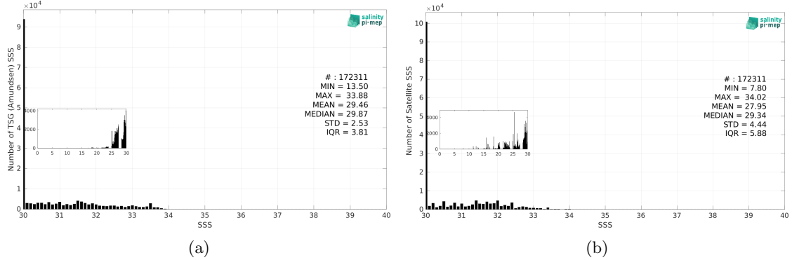
Figure 2: Histograms of SSS from TSG (Amundsen) (a) and SMOS SSS L3 v9 - 18 Days (CATDS-CEC-LOCEAN) (b) considering all match-up pairs per bins of 0.1 over the Arctic Ocean Pi-MEP region and for the full satellite product period.
