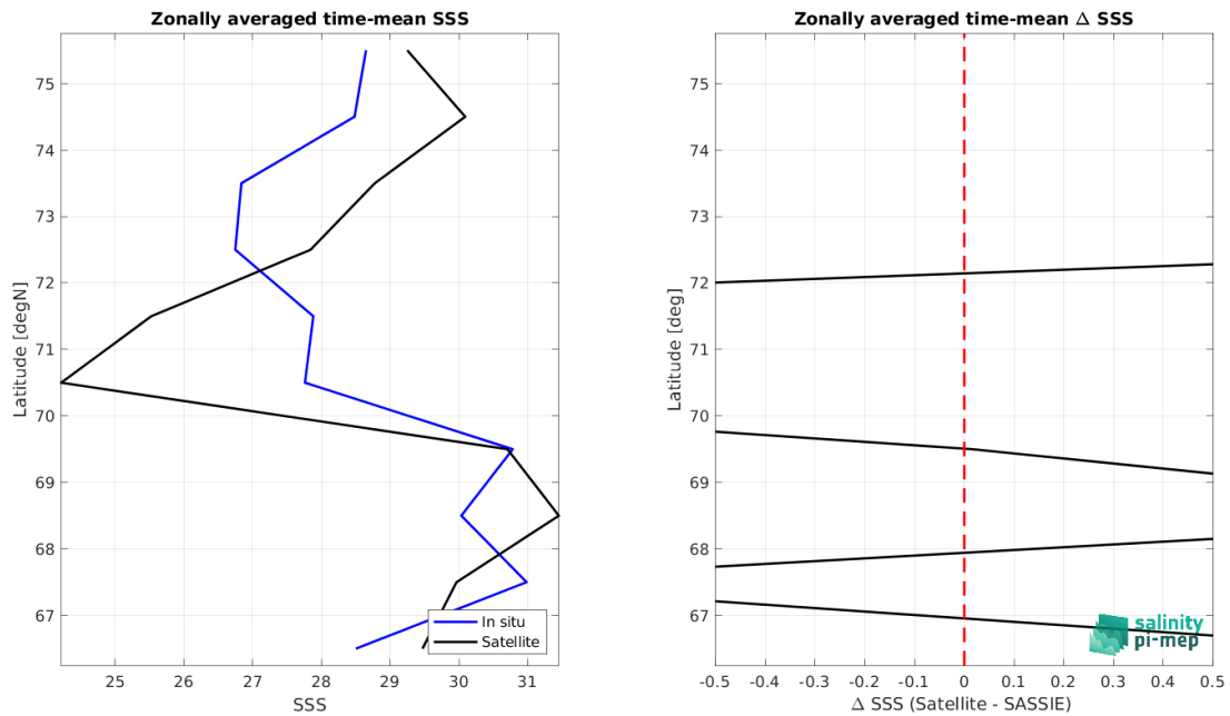
Figure 9: Left panel: Zonal mean SSS from SMOS SSS L3 v9 - 18 Days (CATDS-CEC-LOCEAN) satellite product (black) and from SASSIE (blue). Right panel: Zonal mean of \Delta SSS (Satellite - SASSIE) for all the collected Pi-MEP match-up pairs estimated over the full satellite product period.
