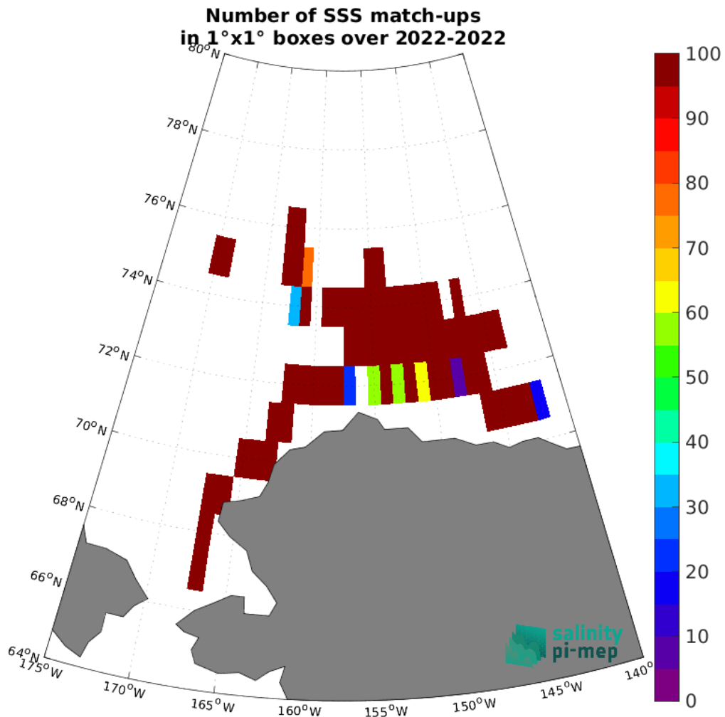
Figure 5: Number of SSS match-ups between SASSIE SSS and the SMOS SSS L3 v9 - 18 Days (CATDS-CEC-LOCEAN) SSS product for the Arctic Ocean Pi-MEP region over 1°x1° boxes and for the full satellite product period.
