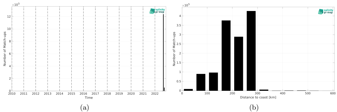
Figure 2: Number of match-ups between SASSIE and SMOS SSS L3 v9 - 18 Days (CATDS-CEC-LOCEAN) SSS as a function of time (a) and as function of the distance to coast (b) over the Arctic Ocean Pi-MEP region and for the full satellite product period.
