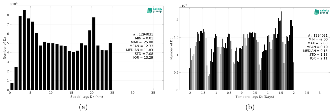
Figure 6: Histograms of the spatial (a) and temporal (b) lags between the location/time of the SASSIE measurement and the date of the corresponding SMOS SSS L3 v9 - 18 Days (CATDS-CEC-LOCEAN) SSS pixel.
