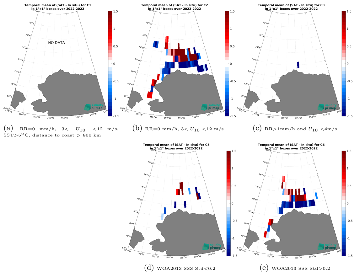
Figure 14: Temporal mean gridded over spatial boxes of size 1^\circ \times 1^\circ of \Delta SSS (SMOS SSS L3 v9 - 18 Days (CATDS-CEC-LOCEAN) - SASSIE) for 5 different subdatasets corresponding to:RR=0 mm/h, 3 < U_{10} < 12 m/s, SST>5°C, distance to coast > 800 km (a), RR=0 mm/h, 3 < U_{10} < 12 m/s (b), RR>1mm/h and U_{10} < 4 m/s (c), WOA2013 SSS Std<0.2 (d), WOA2013 SSS Std>0.2 (e).
