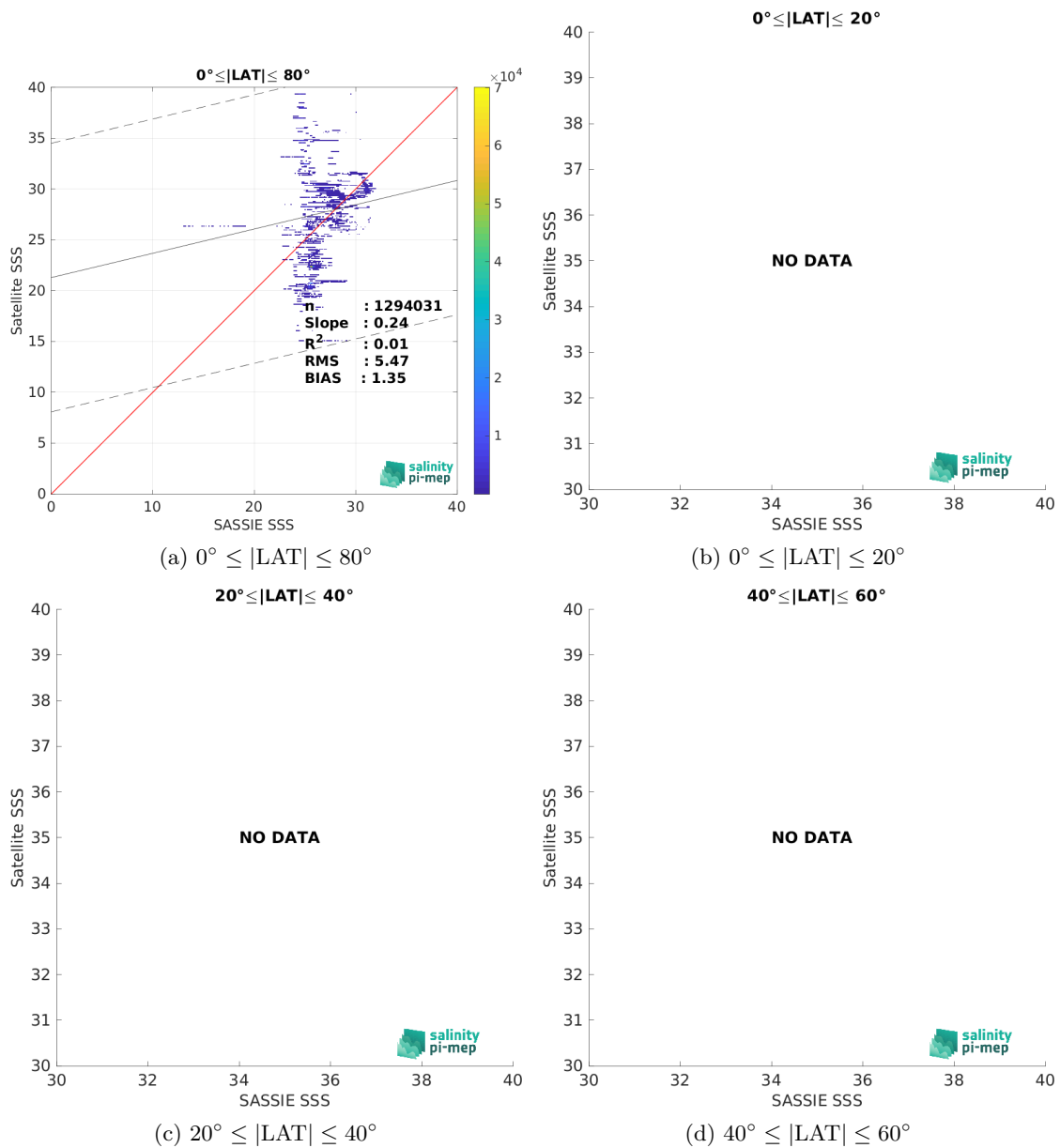
Figure 10: Contour maps of the concentration of SMOS SSS L3 v9 - 18 Days (CATDS-CEC-LOCEAN) SSS (y-axis) versus SASSIE SSS (x-axis) at match-up pairs for different latitude bands. For each plot, the red line shows x=y . The black thin and dashed lines indicate a linear fit through the data cloud and the \pm 95\% confidence levels, respectively. The number match-up pairs n , the slope and R^2 coefficient of the linear fit, the root mean square (RMS) and the mean bias between satellite and in situ data are indicated for each latitude band in each plots.
