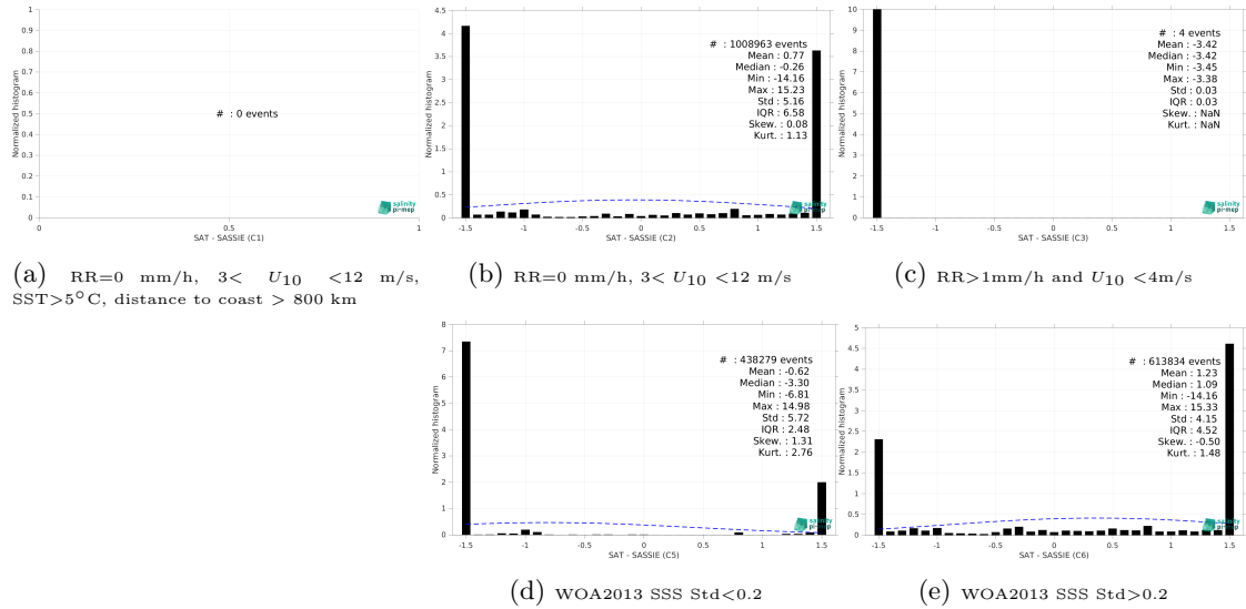
Figure 15: Normalized histogram of \Delta SSS (SMOS SSS L3 v9 - 18 Days (CATDS-CEC-LOCEAN) - SASSIE) for 5 different subdatasets corresponding to: RR=0 mm/h, 3 < U_{10} < 12 m/s, SST > 5°C, distance to coast > 800 km (a), RR=0 mm/h, 3 < U_{10} < 12 m/s (b), RR > 1mm/h and U_{10} < 4 m/s (c), WOA2013 SSS Std < 0.2 (d), WOA2013 SSS Std > 0.2 (e).
