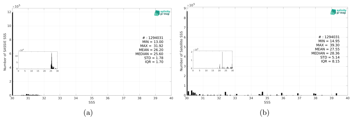
Figure 3: Histograms of SSS from SASSIE (a) and SMOS SSS L3 v9 - 18 Days (CATDS-CEC-LOCEAN) (b) considering all match-up pairs per bins of 0.1 over the Arctic Ocean Pi-MEP region and for the full satellite product period.
