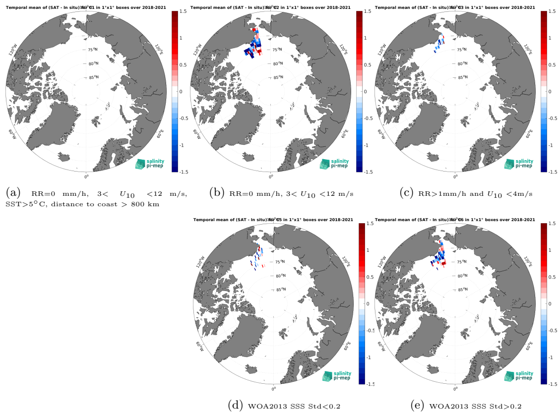
Figure 14: Temporal mean gridded over spatial boxes of size 1^\circ \times 1^\circ of \Delta SSS (SMOS SSS L3 v9 - 18 Days (CATDS-CEC-LOCEAN) - Sailydrone) for 5 different subdatasets corresponding to:RR=0 mm/h, 3 < U_{10} < 12 m/s, SST > 5^\circ\text{C} , distance to coast > 800 km (a), RR=0 mm/h, 3 < U_{10} < 12 m/s (b), RR > 1 mm/h and U_{10} < 4 m/s (c), WOA2013 SSS Std < 0.2 (d), WOA2013 SSS Std > 0.2 (e).
