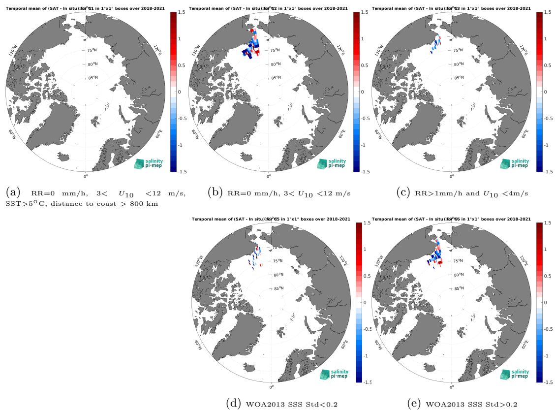
Figure 14: Temporal mean gridded over spatial boxes of size 1^\circ \times 1^\circ of \Delta\text{SSS} (SMOS SSS L3 v9 - 18 Days (CATDS-CEC-LOCEAN) - Sailydrone) for 5 different subdatasets corresponding to: RR=0 mm/h, 3 < U_{10} < 12 m/s, SST > 5°C, distance to coast > 800 km (a), RR=0 mm/h, 3 < U_{10} < 12 m/s (b), RR > 1mm/h and U_{10} < 4 m/s (c), WOA2013 SSS Std < 0.2 (d), WOA2013 SSS Std > 0.2 (e).
