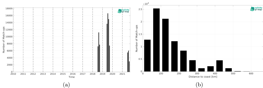
Figure 2: Number of match-ups between Saildrone and SMOS SSS L3 v9 - 18 Days (CATDS-CEC-LOCEAN) SSS as a function of time (a) and as function of the distance to coast (b) over the Arctic Ocean Pi-MEP region and for the full satellite product period.
