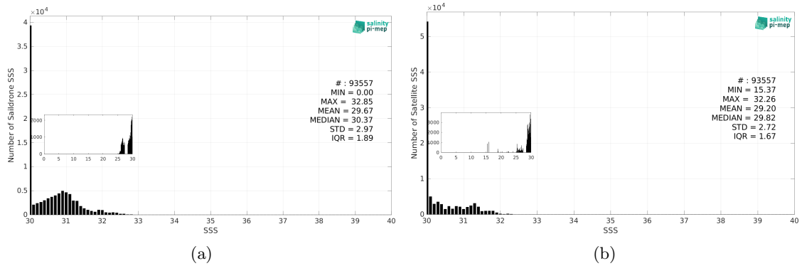
Figure 2: Histograms of SSS from Saildrone (a) and SMOS SSS L3 v9 - 18 Days (CATDS-CEC-LOCEAN) (b) considering all match-up pairs per bins of 0.1 over the Arctic Ocean Pi-MEP region and for the full satellite product period.
