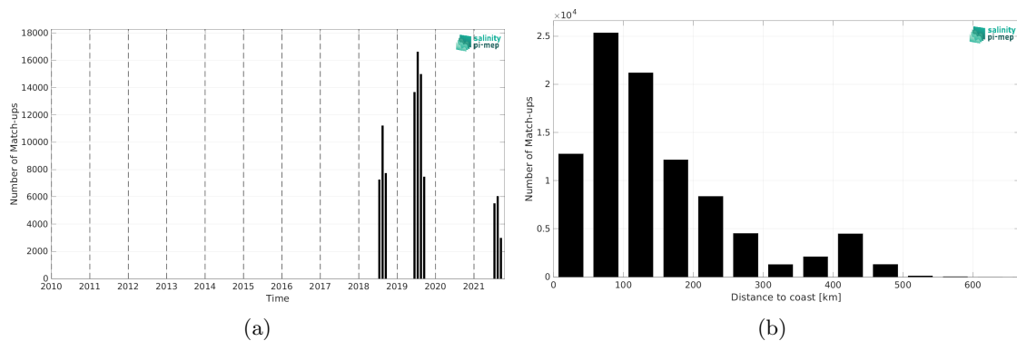
Figure 1: Number of match-ups between Saildrone and SMOS SSS L3 v9 - 18 Days (CATDS-CEC-LOCEAN) SSS as a function of time (a) and as function of the distance to coast (b) over the Arctic Ocean Pi-MEP region and for the full satellite product period.
