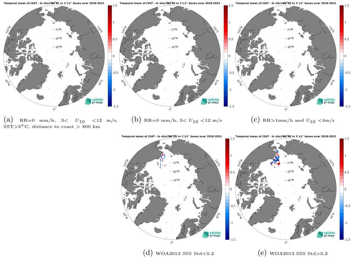
Figure 12: Temporal mean gridded over spatial boxes of size 1^{\circ}\times 1^{\circ} of \Delta\text{SSS} (SMOS SSS L3 v9 - 18 Days (CATDS-CEC-LOCEAN) - Sailydrone) for 5 different subdatasets corresponding to: RR=0 mm/h, 3 < U_{10} < 12 m/s, SST > 5^{\circ}\text{C} , distance to coast > 800 km (a), RR=0 mm/h, 3 < U_{10} < 12 m/s (b), RR > 1 mm/h and U_{10} < 4 m/s (c), WOA2013 SSS Std < 0.2 (d), WOA2013 SSS Std > 0.2 (e).
