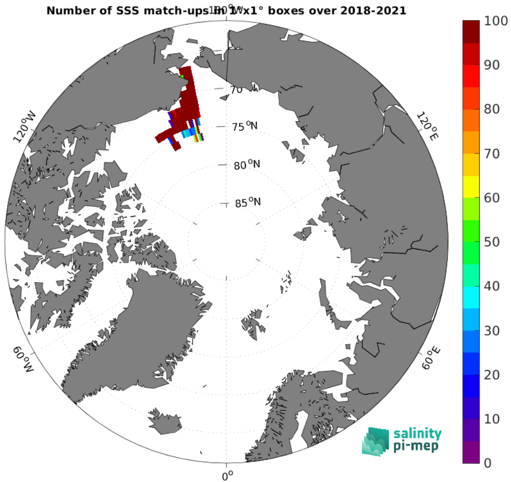
Figure 4: Number of SSS match-ups between Saildrone SSS and the SMOS SSS L3 v9 - 18 Days (CATDS-CEC-LOCEAN) SSS product for the Arctic Ocean Pi-MEP region over 1^\circ \times 1^\circ boxes and for the full satellite product period.
