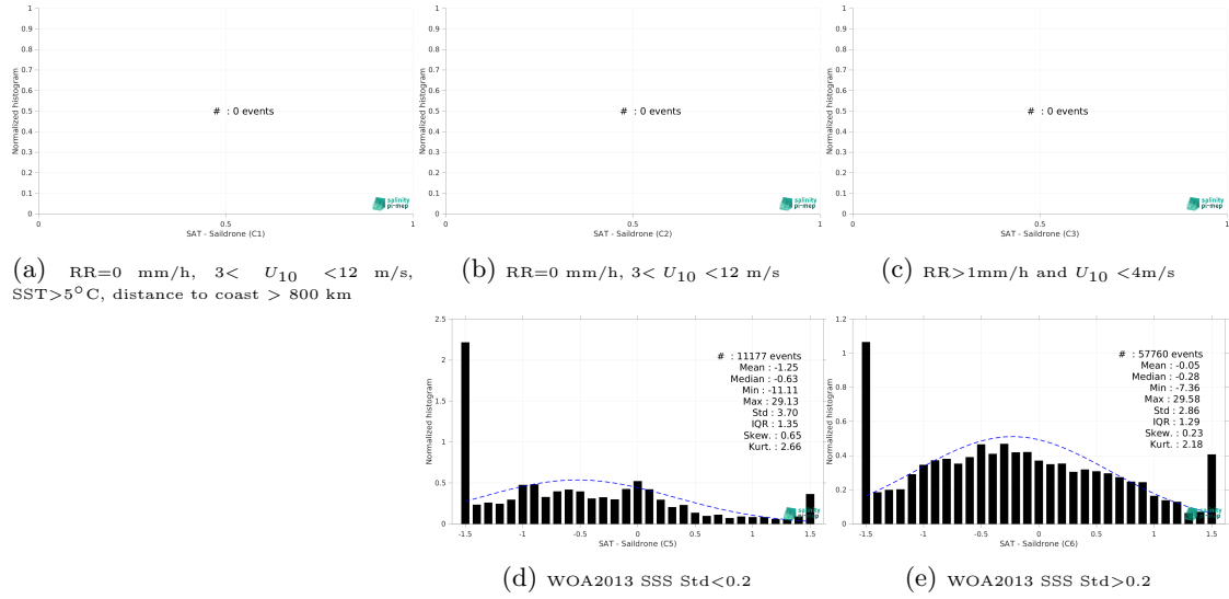
Figure 13: Normalized histogram of \Delta SSS (SMOS SSS L3 v9 - 18 Days (CATDS-CEC-LOCEAN) - Saildrone) for 5 different subdatasets corresponding to: RR=0 mm/h, 3 < U_{10} < 12 m/s, SST >5^{\circ} C, distance to coast > 800 km (a), RR=0 mm/h, 3 < U_{10} < 12 m/s (b), RR >1 mm/h and U_{10} < 4 m/s (c), WOA2013 SSS Std <0.2 (d), WOA2013 SSS Std >0.2 (e).
