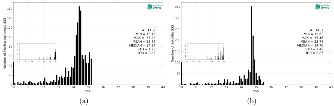
Figure 2: Histograms of SSS from Marine mammals (a) and SMOS SSS L3 v9 - 18 Days (CATDS-CEC-LOCEAN) (b) considering all match-up pairs per bins of 0.1 over the Arctic Ocean Pi-MEP region and for the full satellite product period.
