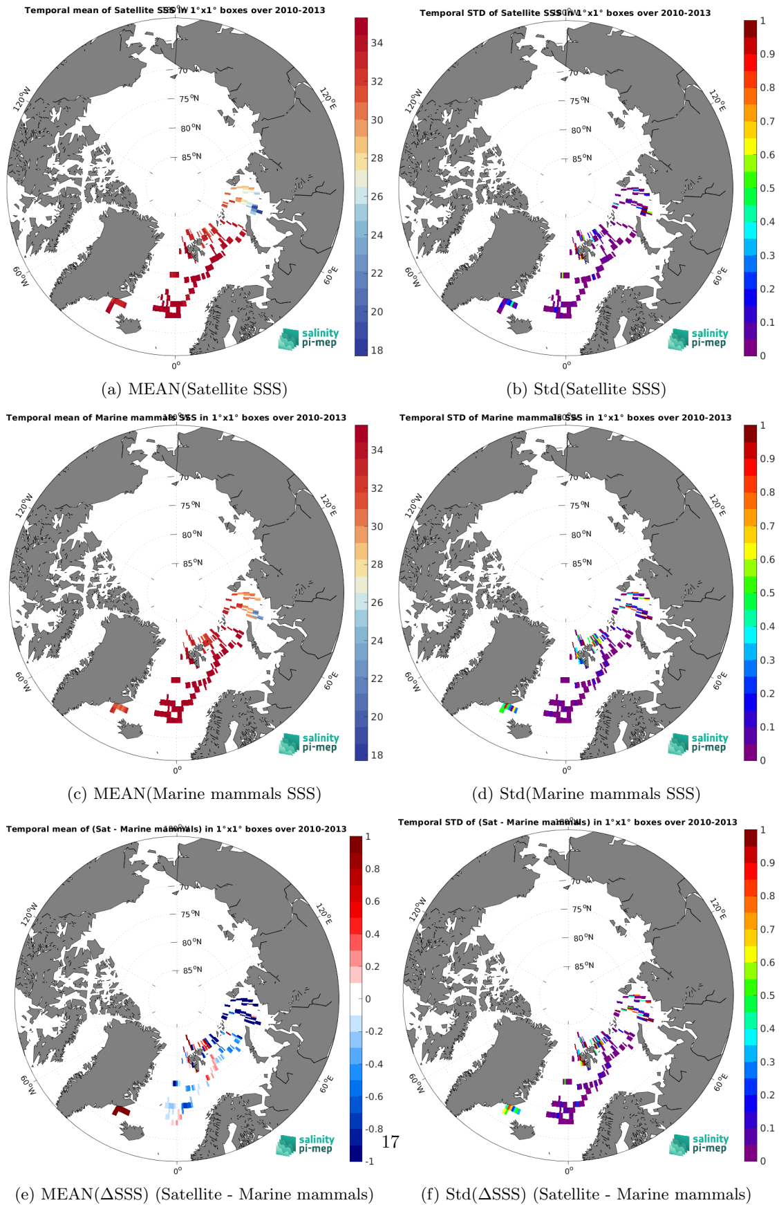
Figure 6: Temporal mean (left) and Std (right) of SSS from SMOS SSS L3 v9 - 18 Days (CATDS-CEC-LOCEAN) (top), Marine mammals (middle), and of \Delta SSS (Satellite - Marine mammals). Only match-up pairs are used to generate these maps.
