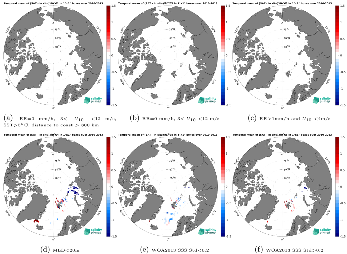
Figure 12: Temporal mean gridded over spatial boxes of size 1^{\circ}\times 1^{\circ} of \Delta\text{SSS} (SMOS SSS L3 v9 - 18 Days (CATDS-CEC-LOCEAN) - Marine mammals) for 6 different subdatasets corresponding to: RR=0 mm/h, 3 < U_{10} < 12 m/s, SST > 5^{\circ}\text{C} , distance to coast > 800 km (a), RR=0 mm/h, 3 < U_{10} < 12 m/s (b), RR > 1\text{mm/h} and U_{10} < 4\text{m/s} (c), MLD < 20\text{m} (d), WOA2013 SSS Std < 0.2 (e), WOA2013 SSS Std > 0.2 (f).
