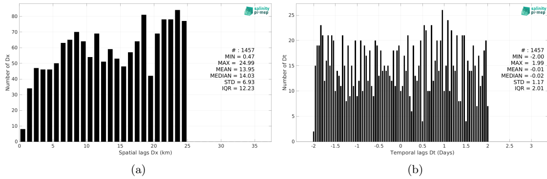
Figure 5: Histograms of the spatial (a) and temporal (b) lags between the location/time of the Marine mammals measurement and the date of the corresponding SMOS SSS L3 v9 - 18 Days (CATDS-CEC-LOCEAN) SSS pixel.
