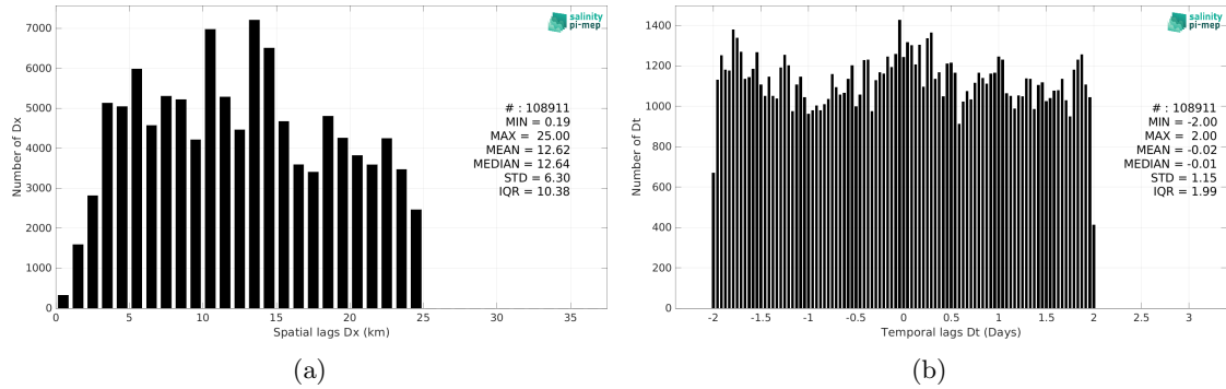
Figure 6: Histograms of the spatial (a) and temporal (b) lags between the location/time of the ICES measurement and the date of the corresponding SMOS SSS L3 v9 - 18 Days (CATDS-CEC-LOCEAN) SSS pixel.
