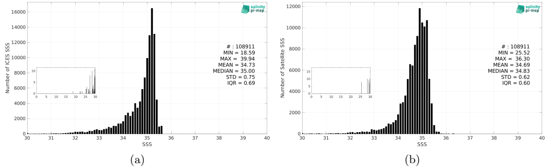
Figure 3: Histograms of SSS from ICES (a) and SMOS SSS L3 v9 - 18 Days (CATDS-CEC-LOCEAN) (b) considering all match-up pairs per bins of 0.1 over the Arctic Ocean Pi-MEP region and for the full satellite product period.
