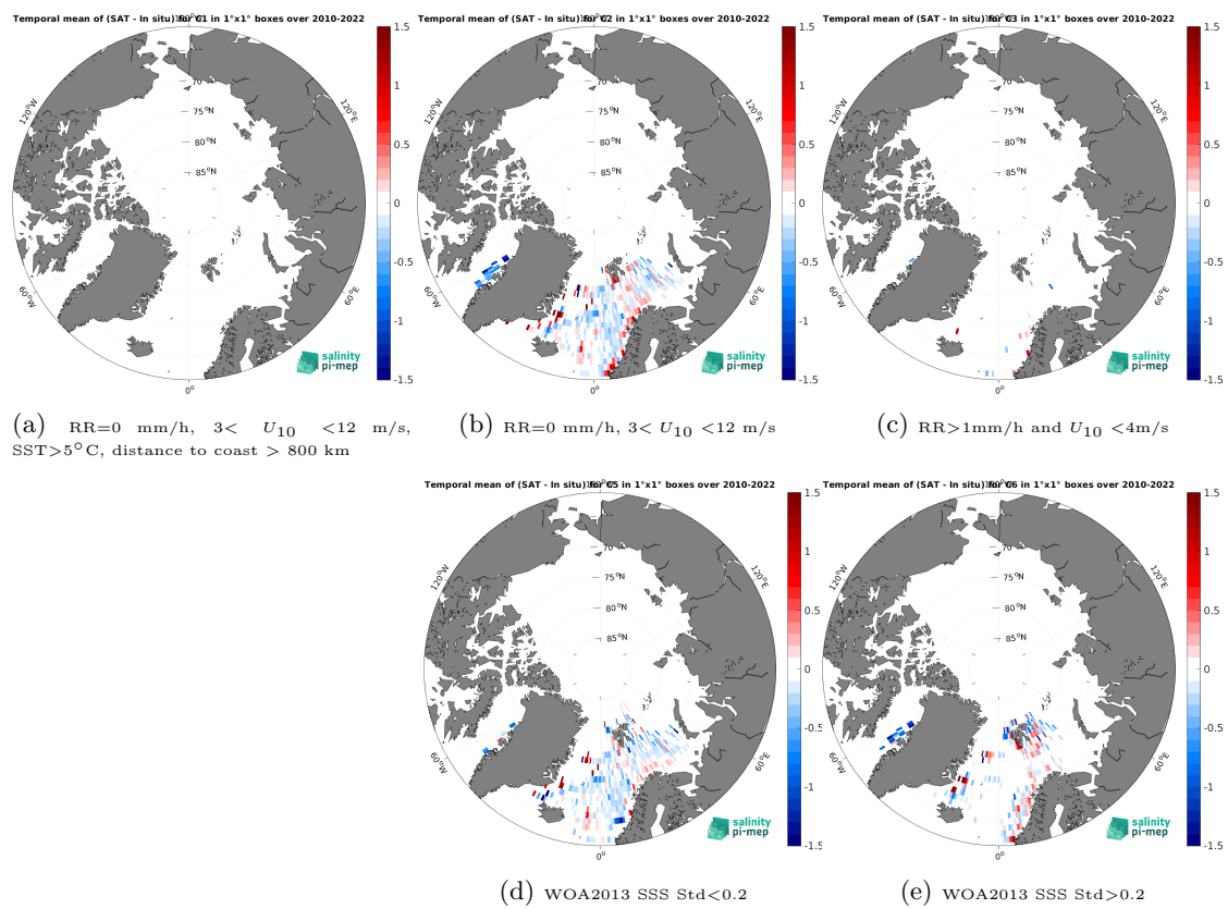
Figure 14: Temporal mean gridded over spatial boxes of size 1^\circ \times 1^\circ of \Delta SSS (SMOS SSS L3 v9 - 18 Days (CATDS-CEC-LOCEAN) - ICES) for 5 different subdatasets corresponding to:RR=0 mm/h, 3 < U_{10} < 12 m/s, SST > 5^\circ\text{C} , distance to coast > 800 km (a), RR=0 mm/h, 3 < U_{10} < 12 m/s (b), RR > 1 mm/h and U_{10} < 4 m/s (c), WOA2013 SSS Std < 0.2 (d), WOA2013 SSS Std > 0.2 (e).
