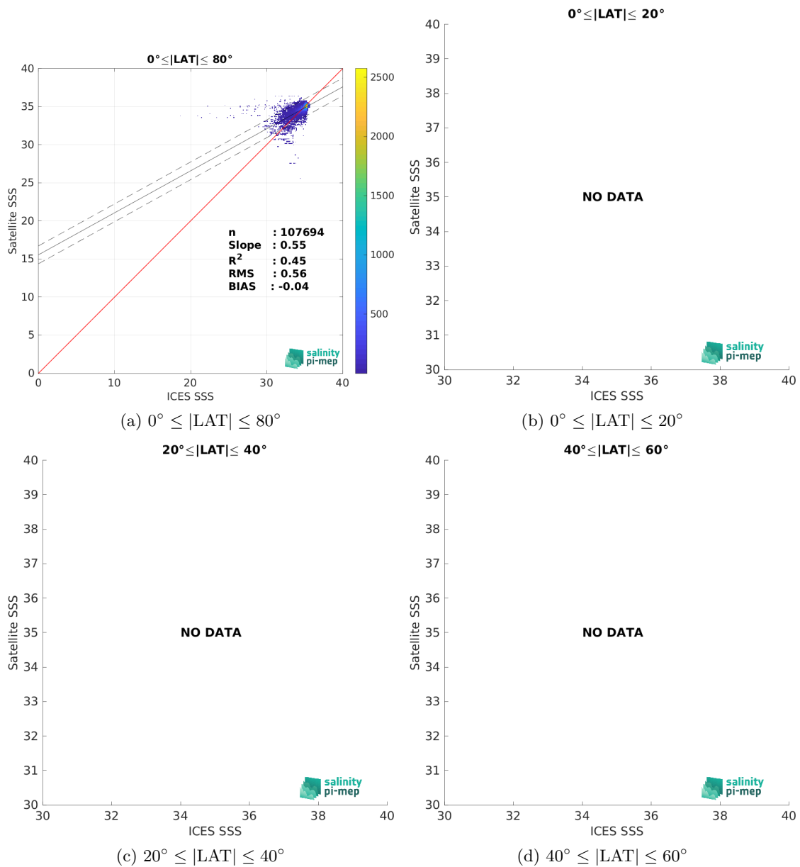
Figure 10: Contour maps of the concentration of SMOS SSS L3 v9 - 18 Days (CATDS-CEC-LOCEAN) SSS (y-axis) versus ICES SSS (x-axis) at match-up pairs for different latitude bands. For each plot, the red line shows x=y . The black thin and dashed lines indicate a linear fit through the data cloud and the \pm 95\% confidence levels, respectively. The number match-up pairs n , the slope and R^2 coefficient of the linear fit, the root mean square (RMS) and the mean bias between satellite and in situ data are indicated for each latitude band in each plots.
