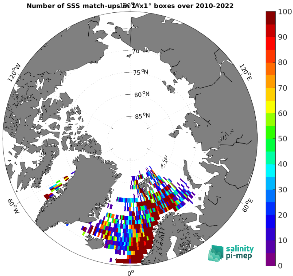
Figure 5: Number of SSS match-ups between ICES SSS and the SMOS SSS L3 v9 - 18 Days (CATDS-CEC-LOCEAN) SSS product for the Arctic Ocean Pi-MEP region over 1^\circ \times 1^\circ boxes and for the full satellite product period.
