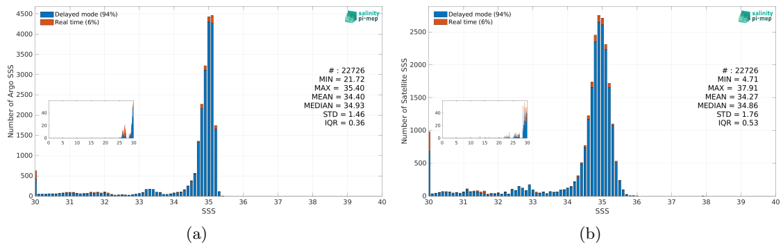
Figure 3: Histograms of SSS from Argo (a) and SMOS SSS L3 v9 - 18 Days (CATDS-CEC-LOCEAN) (b) considering all match-up pairs per bins of 0.1 over the Arctic Ocean Pi-MEP region and for the full satellite product period.
