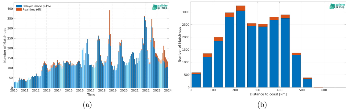
Figure 2: Number of match-ups between Argo and SMOS SSS L3 v9 - 18 Days (CATDS-CEC-LOCEAN) SSS as a function of time (a) and as function of the distance to coast (b) over the Arctic Ocean Pi-MEP region and for the full satellite product period.
