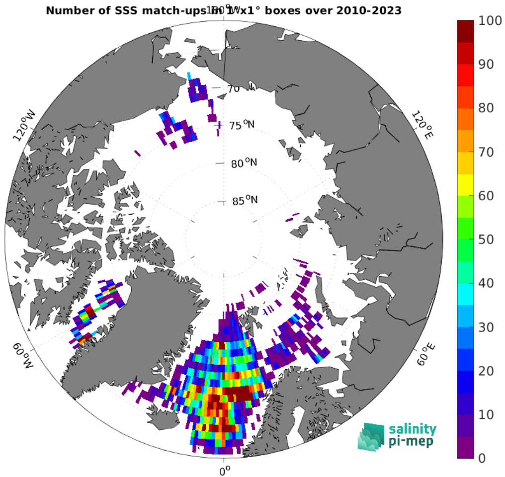
Figure 5: Number of SSS match-ups between Argo SSS and the SMOS SSS L3 v9 - 18 Days (CATDS-CEC-LOCEAN) SSS product for the Arctic Ocean Pi-MEP region over 1^\circ \times 1^\circ boxes and for the full satellite product period.
