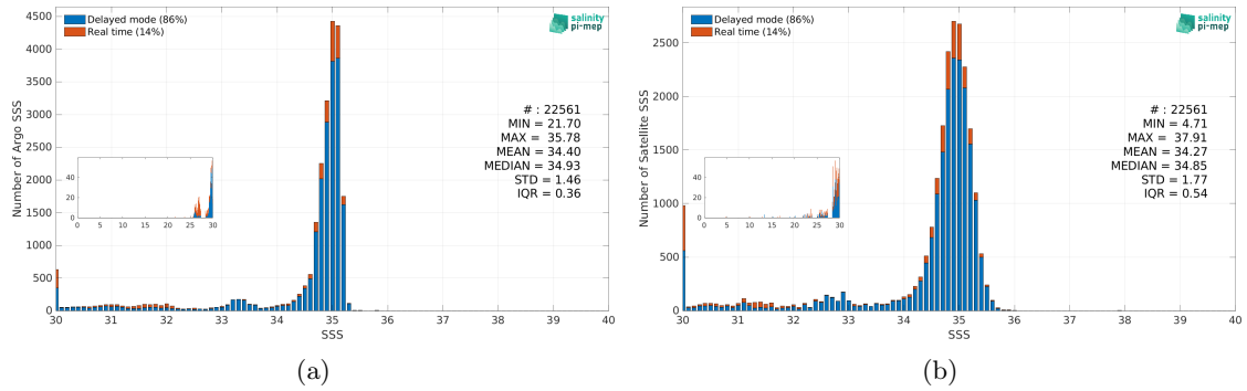
Figure 2: Histograms of SSS from Argo (a) and SMOS SSS L3 v9 - 18 Days (CATDS-CEC-LOCEAN) (b) considering all match-up pairs per bins of 0.1 over the Arctic Ocean Pi-MEP region and for the full satellite product period.
