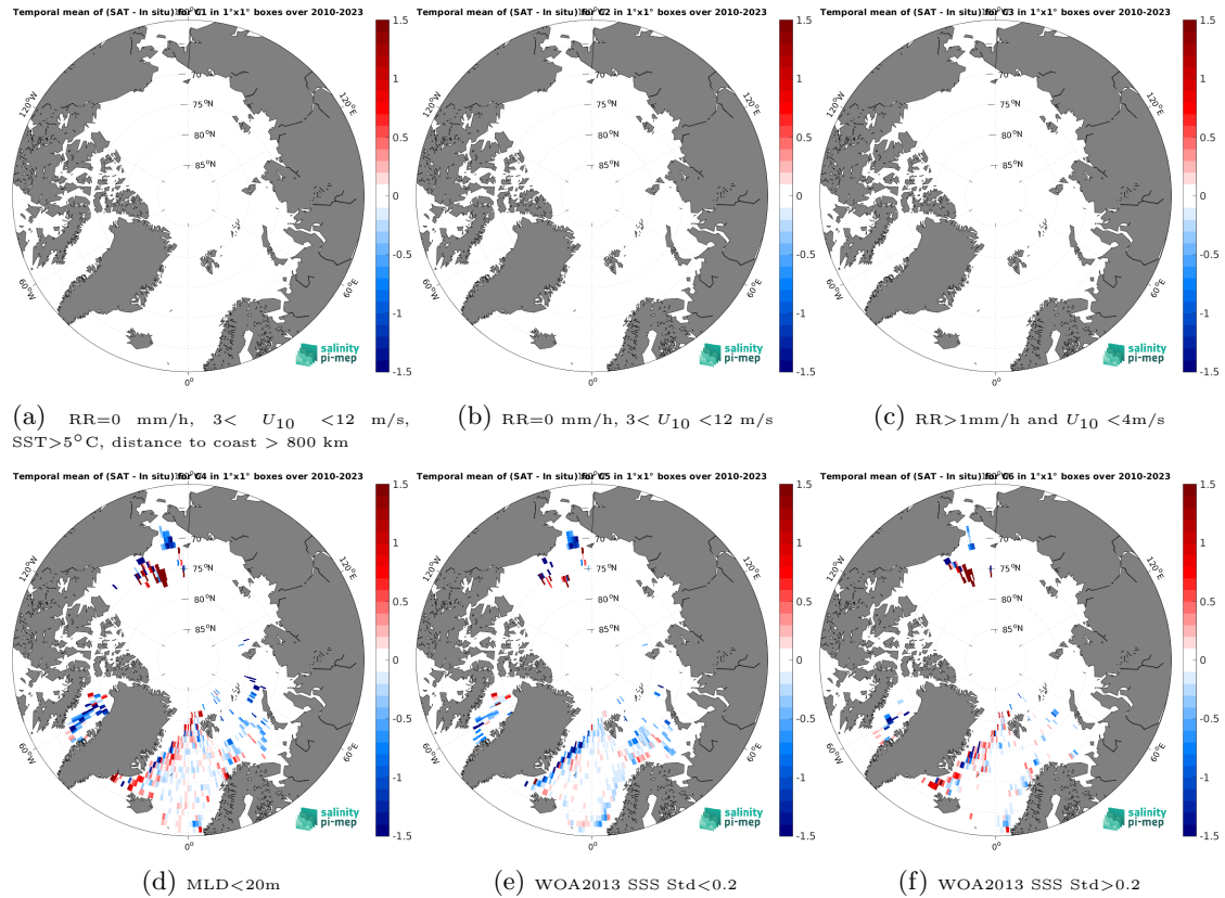
Figure 12: Temporal mean gridded over spatial boxes of size 1^{\circ}\times 1^{\circ} of \Delta\text{SSS} (SMOS SSS L3 v9 - 18 Days (CATDS-CEC-LOCEAN) - Argo) for 6 different subdatasets corresponding to:RR=0 mm/h, 3 < U_{10} < 12 m/s, SST >5^{\circ}\text{C} , distance to coast > 800 km (a), RR=0 mm/h, 3 < U_{10} < 12 m/s (b), RR >1\text{mm/h} and U_{10} < 4\text{m/s} (c),MLD <20\text{m} (d),WOA2013 SSS Std <0.2 (e),WOA2013 SSS Std >0.2 (f).
