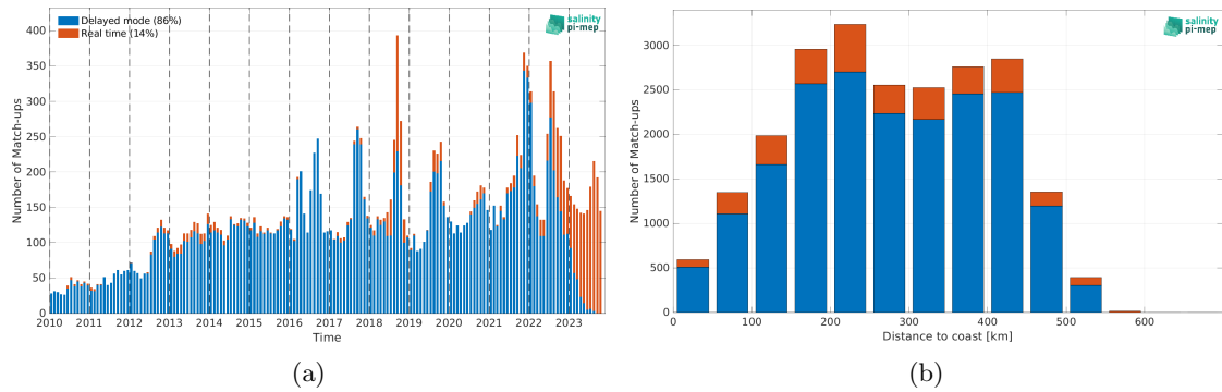
Figure 1: Number of match-ups between Argo and SMOS SSS L3 v9 - 18 Days (CATDS-CEC-LOCEAN) SSS as a function of time (a) and as function of the distance to coast (b) over the Arctic Ocean Pi-MEP region and for the full satellite product period.
