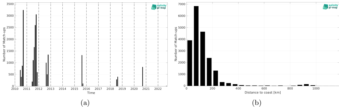
Figure 1: Number of match-ups between TSG (SAMOS) and SMOS SSS L3 v8 - 9 Days (CATDS-CEC-LOCEAN) SSS as a function of time (a) and as function of the distance to coast (b) over the Arctic Ocean Pi-MEP region and for the full satellite product period.
