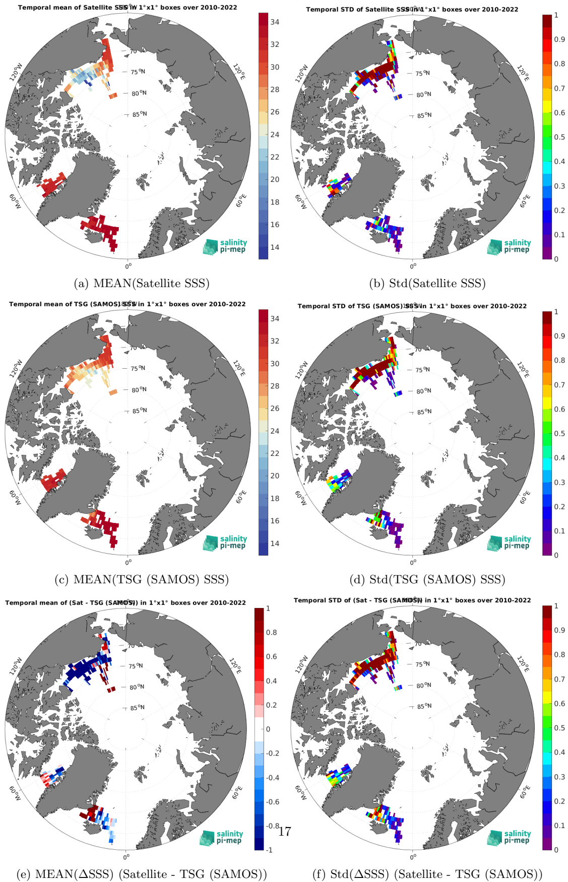
Figure 6: Temporal mean (left) and Std (right) of SSS from SMOS SSS L3 v8 - 9 Days (CATDS-CEC-LOCEAN) (top), TSG (SAMOS) (middle), and of \Delta SSS (Satellite - TSG (SAMOS)). Only match-up pairs are used to generate these maps.
