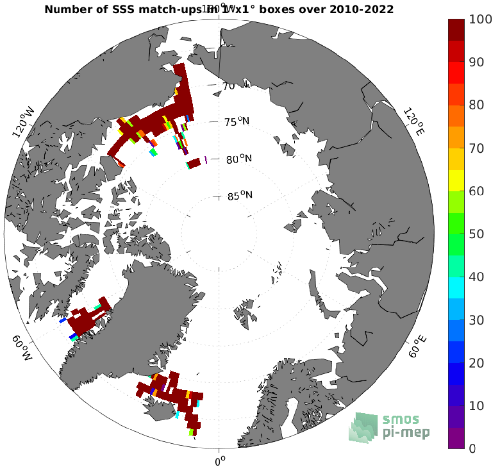
Figure 4: Number of SSS match-ups between TSG (SAMOS) SSS and the SMOS SSS L3 v8 - 9 Days (CATDS-CECOS-LOCEAN) SSS product for the Arctic Ocean Pi-MEP region over 1^\circ \times 1^\circ boxes and for the full satellite product period.
