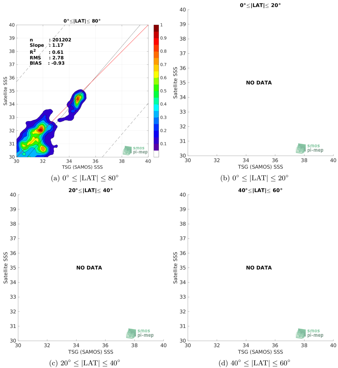
Figure 9: Contour maps of the concentration of SMOS SSS L3 v8 - 9 Days (CATDS-CECOS-LOCEAN) SSS (y-axis) versus TSG (SAMOS) SSS (x-axis) at match-up pairs for different latitude bands. For each plot, the red line shows x=y . The black thin and dashed lines indicate a linear fit through the data cloud and the \pm 95\% confidence levels, respectively. The number match-up pairs n , the slope and R^2 coefficient of the linear fit, the root mean square (RMS) and the mean bias between satellite and in situ data are indicated for each latitude band in each plots.
