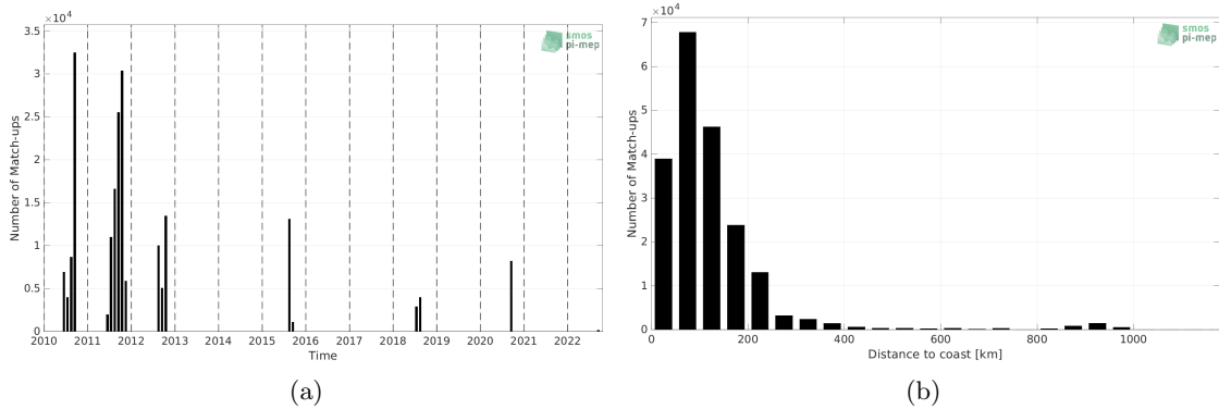
Figure 1: Number of match-ups between TSG (SAMOS) and SMOS SSS L3 v8 - 9 Days (CATDS-CECOS-LOCEAN) SSS as a function of time (a) and as function of the distance to coast (b) over the Arctic Ocean Pi-MEP region and for the full satellite product period.
