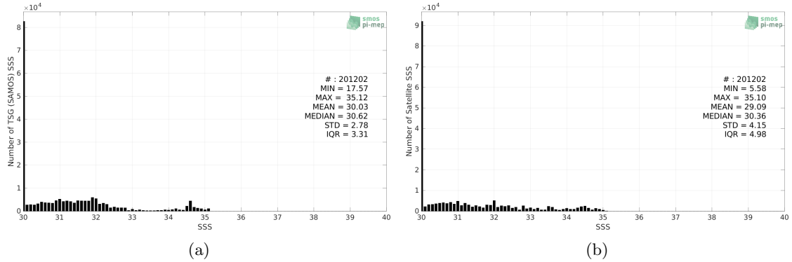
Figure 2: Histograms of SSS from TSG (SAMOS) (a) and SMOS SSS L3 v8 - 9 Days (CATDS-CECOS-LOCEAN) (b) considering all match-up pairs per bins of 0.1 over the Arctic Ocean Pi-MEP region and for the full satellite product period.
