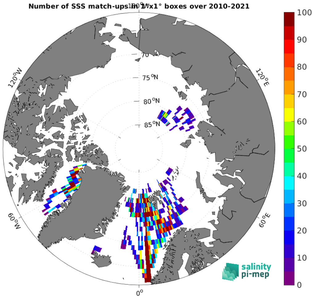
Figure 4: Number of SSS match-ups between TSG (Polarstern) SSS and the SMOS SSS L3 v8 - 9 Days (CATDS-CEC-LOCEAN) SSS product for the Arctic Ocean Pi-MEP region over 1^\circ \times 1^\circ boxes and for the full satellite product period.
