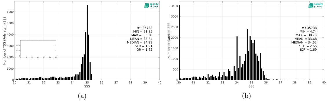
Figure 2: Histograms of SSS from TSG (Polarstern) (a) and SMOS SSS L3 v8 - 9 Days (CATDS-CEC-LOCEAN) (b) considering all match-up pairs per bins of 0.1 over the Arctic Ocean Pi-MEP region and for the full satellite product period.
