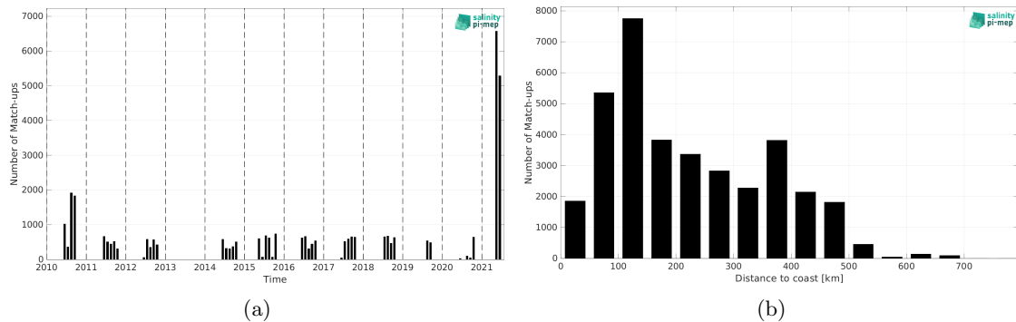
Figure 1: Number of match-ups between TSG (Polarstern) and SMOS SSS L3 v8 - 9 Days (CATDS-CEC-LOCEAN) SSS as a function of time (a) and as function of the distance to coast (b) over the Arctic Ocean Pi-MEP region and for the full satellite product period.
