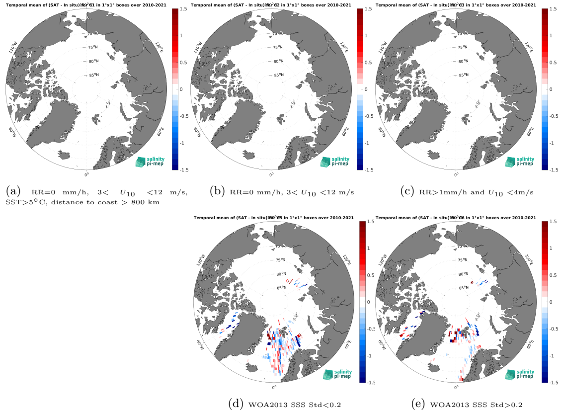
Figure 12: Temporal mean gridded over spatial boxes of size 1^{\circ}\times 1^{\circ} of \Delta\text{SSS} (SMOS SSS L3 v8 - 9 Days (CATDS-CEC-LOCEAN) - TSG (Polarstern)) for 5 different subdatasets corresponding to: RR=0 mm/h, 3 < U_{10} < 12 m/s, SST > 5^{\circ}\text{C} , distance to coast > 800 km (a), RR=0 mm/h, 3 < U_{10} < 12 m/s (b), RR > 1 mm/h and U_{10} < 4 m/s (c), WOA2013 SSS Std < 0.2 (d), WOA2013 SSS Std > 0.2 (e).
