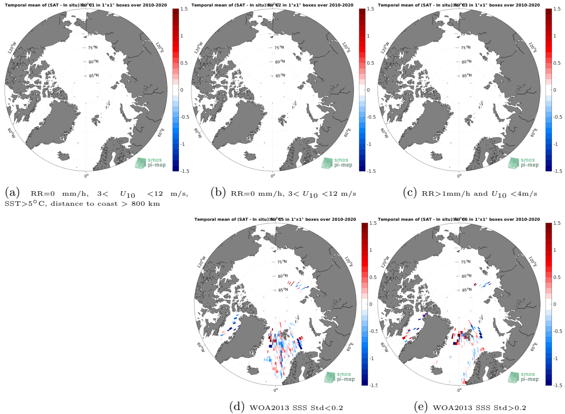
Figure 12: Temporal mean gridded over spatial boxes of size 1^{\circ}\times 1^{\circ} of \Delta\text{SSS} (SMOS SSS L3 v8 - 9 Days (CATDS-CECOS-LOCEAN) - TSG (Polarstern)) for 5 different subdatasets corresponding to:RR=0 mm/h, 3 < U_{10} < 12 m/s, SST >5^{\circ}\text{C} , distance to coast > 800 km (a), RR=0 mm/h, 3 < U_{10} < 12 m/s (b), RR >1 mm/h and U_{10} < 4 m/s (c), WOA2013 SSS Std <0.2 (d), WOA2013 SSS Std >0.2 (e).
