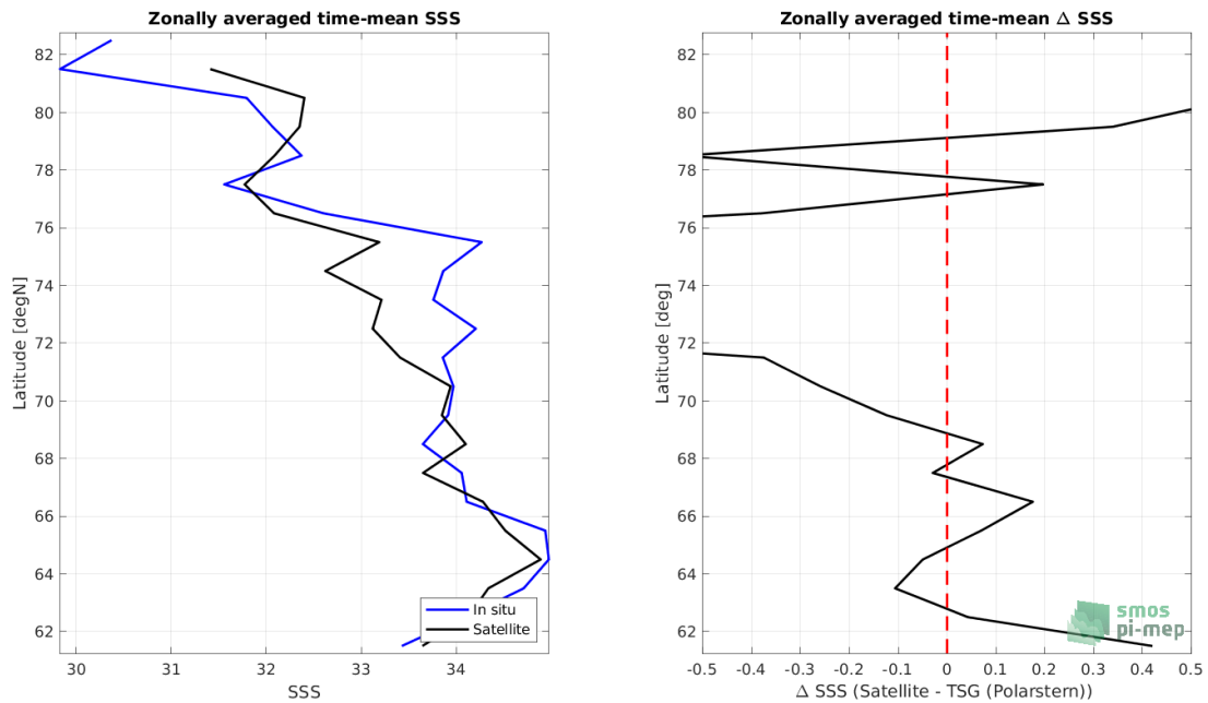
Figure 8: Left panel: Zonal mean SSS from SMOS SSS L3 v8 - 9 Days (CATDS-CECOS-LOCEAN) satellite product (black) and from TSG (Polarstern) (blue). Right panel: Zonal mean of \Delta SSS (Satellite - TSG (Polarstern)) for all the collected Pi-MEP match-up pairs estimated over the full satellite product period.
