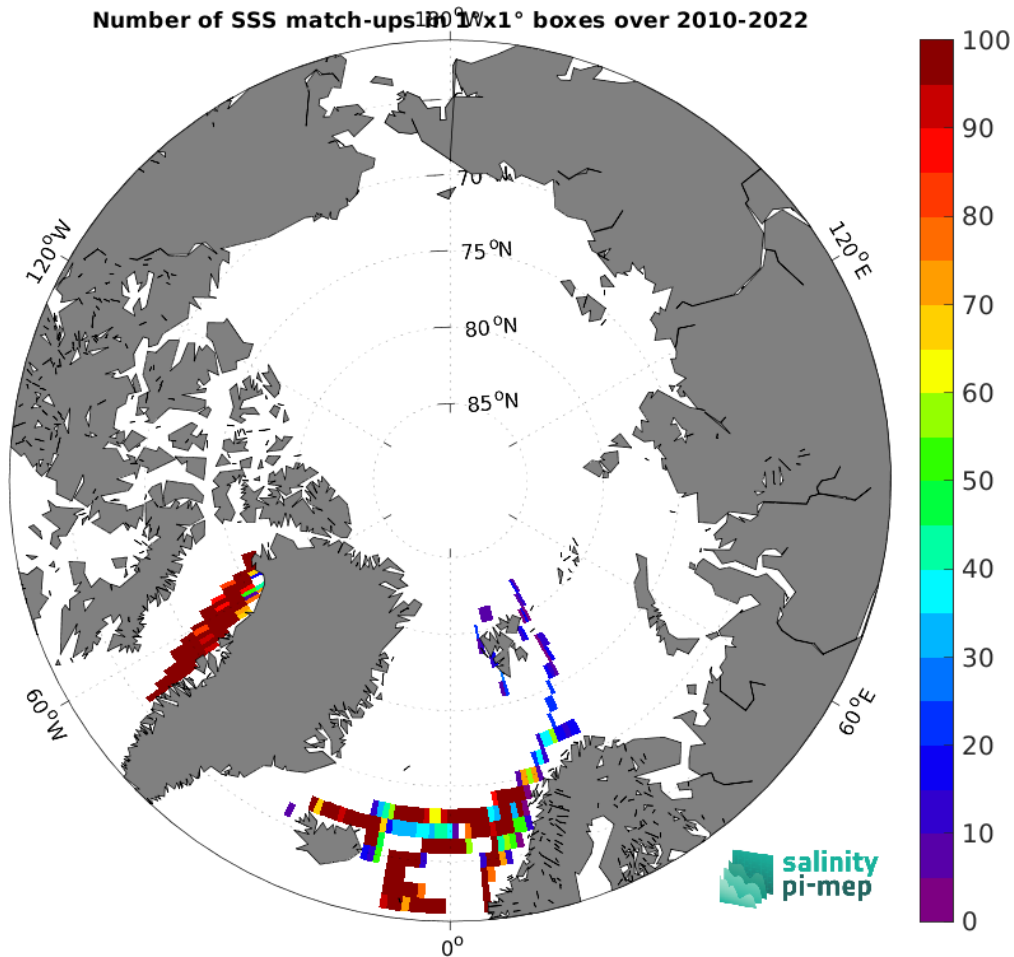
Figure 4: Number of SSS match-ups between TSG (LEGOS-DM) SSS and the SMOS SSS L3 v8 - 9 Days (CATDS-CEC-LOCEAN) SSS product for the Arctic Ocean Pi-MEP region over 1^\circ \times 1^\circ boxes and for the full satellite product period.
