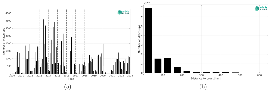
Figure 1: Number of match-ups between TSG (LEGOS-DM) and SMOS SSS L3 v8 - 9 Days (CATDS-CEC-LOCEAN) SSS as a function of time (a) and as function of the distance to coast (b) over the Arctic Ocean Pi-MEP region and for the full satellite product period.
