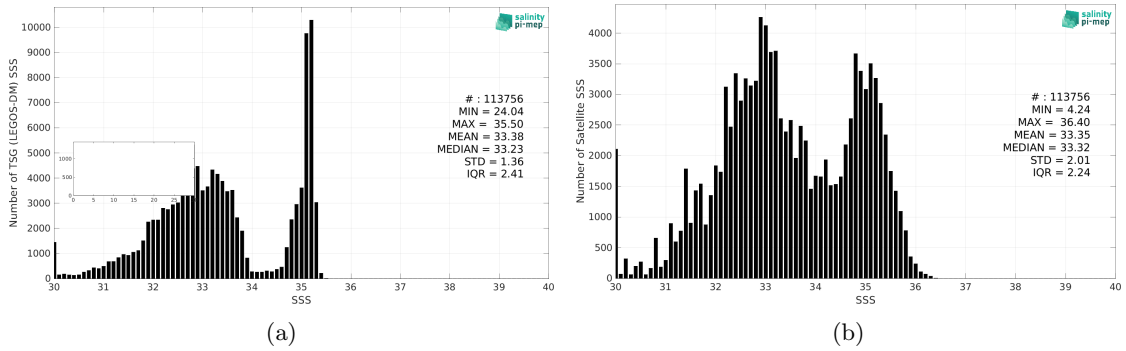
Figure 2: Histograms of SSS from TSG (LEGOS-DM) (a) and SMOS SSS L3 v8 - 9 Days (CATDS-CEC-LOCEAN) (b) considering all match-up pairs per bins of 0.1 over the Arctic Ocean Pi-MEP region and for the full satellite product period.
