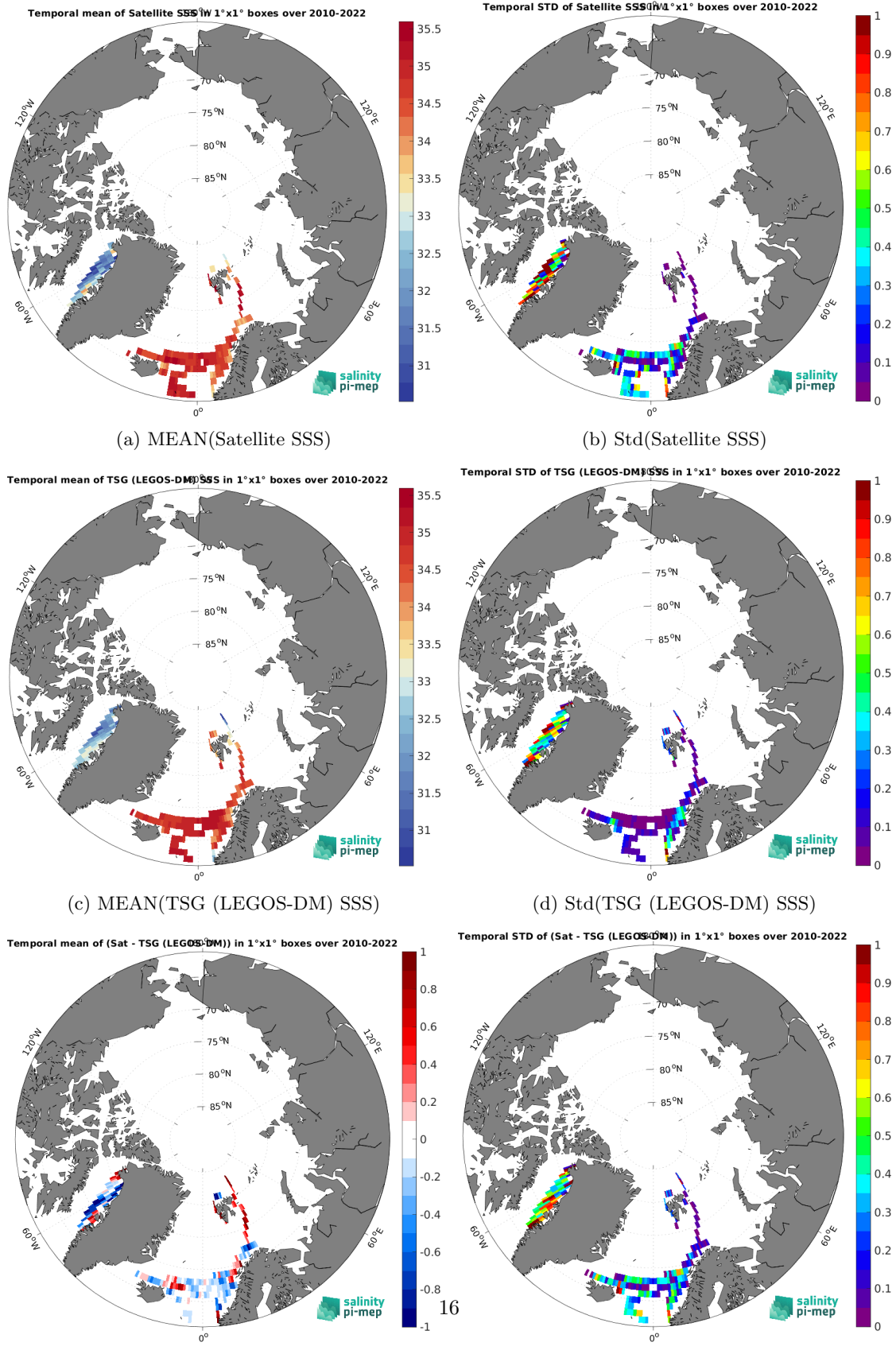
Figure 6: Temporal mean (left) and Std (right) of SSS from SMOS SSS L3 v8 - 9 Days (CATDS-CEC-LOCEAN) (top), TSG (LEGOS-DM) (middle), and of \Delta SSS (Satellite - TSG (LEGOS-DM)). Only match-up pairs are used to generate these maps.
