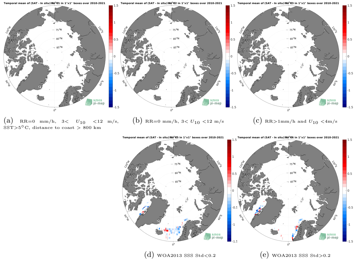
Figure 12: Temporal mean gridded over spatial boxes of size 1^{\circ}\times 1^{\circ} of \Delta\text{SSS} (SMOS SSS L3 v8 - 9 Days (CATDS-CECOS-LOCEAN) - TSG (LEGOS-DM)) for 5 different subdatasets corresponding to:RR=0 mm/h, 3 < U_{10} < 12 m/s, SST >5^{\circ}\text{C} , distance to coast > 800 km (a), RR=0 mm/h, 3 < U_{10} < 12 m/s (b), RR >1 mm/h and U_{10} < 4 m/s (c), WOA2013 SSS Std <0.2 (d), WOA2013 SSS Std >0.2 (e).
