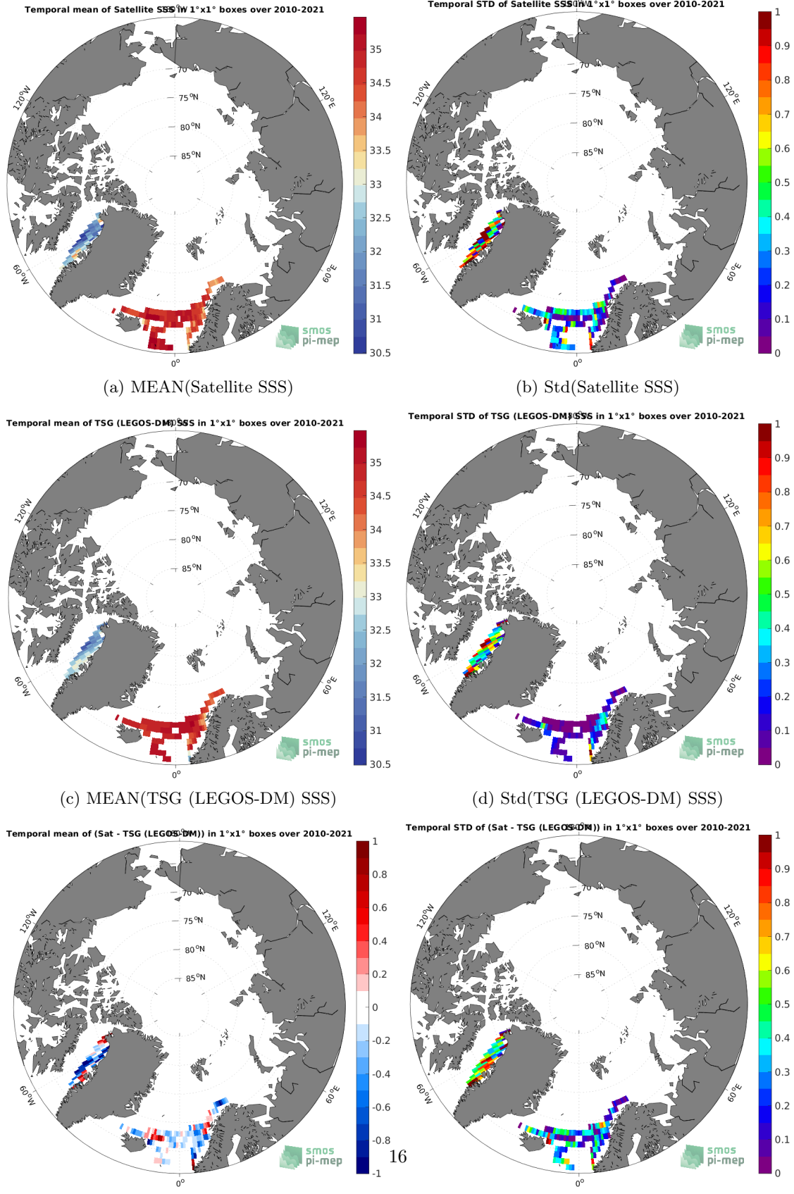
(e) MEAN( \Delta SSS) (Satellite - TSG (LEGOS-DM)) (f) Std( \Delta SSS) (Satellite - TSG (LEGOS-DM)) Figure 6: Temporal mean (left) and Std (right) of SSS from SMOS SSS L3 v8 - 9 Days (CATDS-CECOS-LOCEAN) (top), TSG (LEGOS-DM) (middle), and of \Delta SSS (Satellite - TSG (LEGOS-DM)). Only match-up pairs are used to generate these maps.
