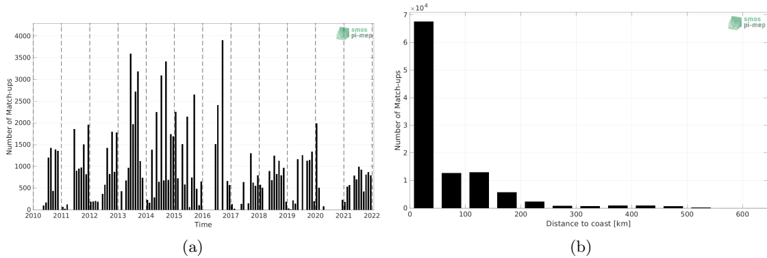
Figure 1: Number of match-ups between TSG (LEGOS-DM) and SMOS SSS L3 v8 - 9 Days (CATDS-CECOS-LOCEAN) SSS as a function of time (a) and as function of the distance to coast (b) over the Arctic Ocean Pi-MEP region and for the full satellite product period.
