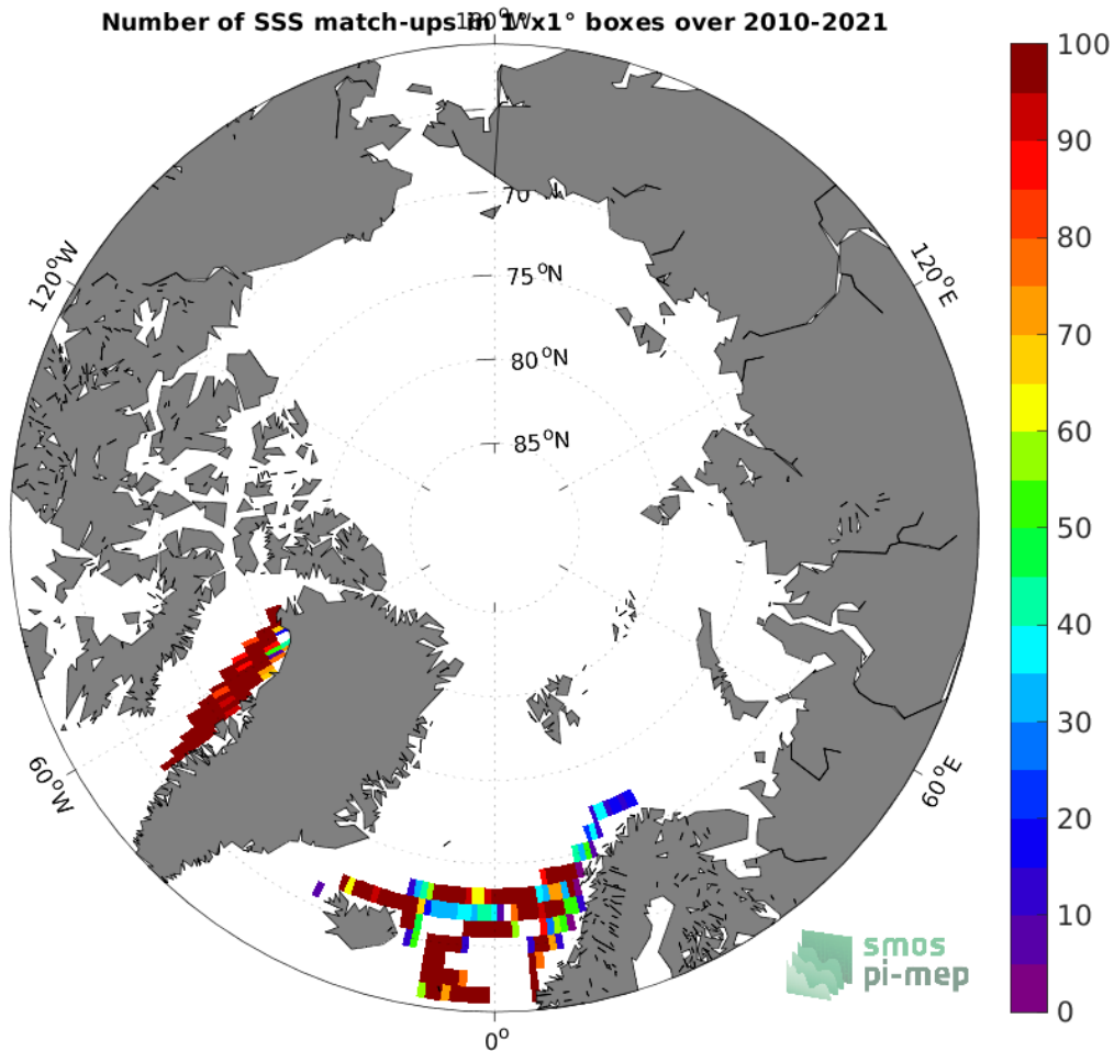
Figure 4: Number of SSS match-ups between TSG (LEGOS-DM) SSS and the SMOS SSS L3 v8 - 9 Days (CATDS-CECOS-LOCEAN) SSS product for the Arctic Ocean Pi-MEP region over 1^\circ \times 1^\circ boxes and for the full satellite product period.
