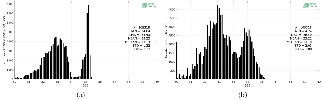
Figure 2: Histograms of SSS from TSG (LEGOS-DM) (a) and SMOS SSS L3 v8 - 9 Days (CATDS-CECOS-LOCEAN) (b) considering all match-up pairs per bins of 0.1 over the Arctic Ocean Pi-MEP region and for the full satellite product period.
