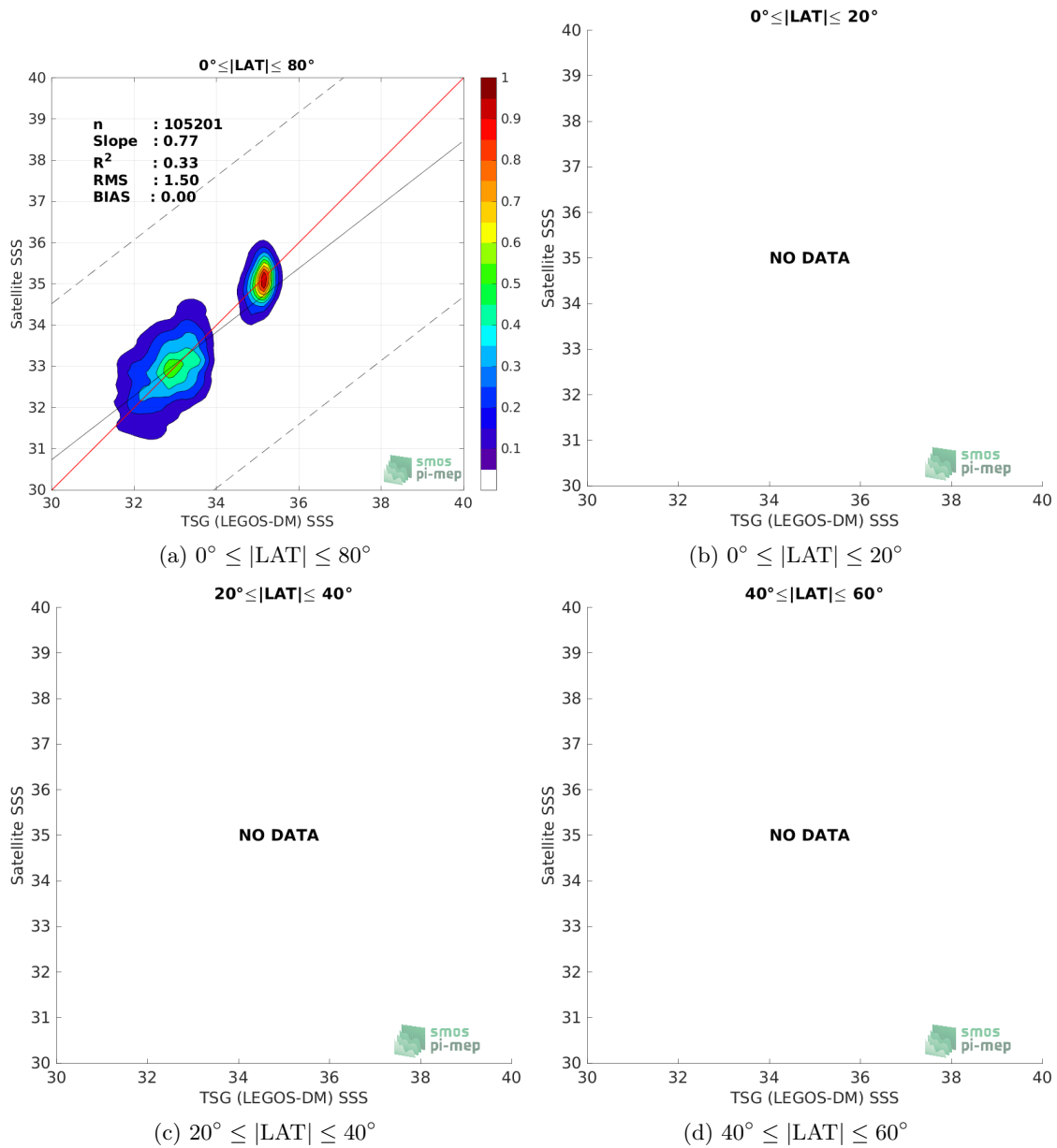
Figure 9: Contour maps of the concentration of SMOS SSS L3 v8 - 9 Days (CATDS-CECOS-LOCEAN) SSS (y-axis) versus TSG (LEGOS-DM) SSS (x-axis) at match-up pairs for different latitude bands. For each plot, the red line shows x=y . The black thin and dashed lines indicate a linear fit through the data cloud and the \pm 95\% confidence levels, respectively. The number match-up pairs n , the slope and R^2 coefficient of the linear fit, the root mean square (RMS) and the mean bias between satellite and in situ data are indicated for each latitude band in each plots.
