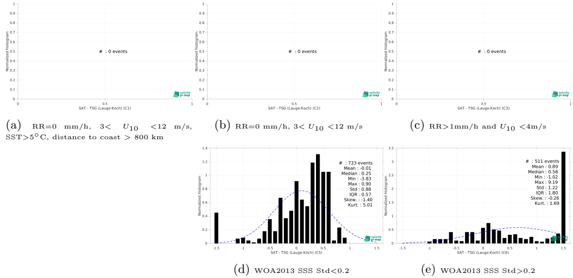
Figure 13: Normalized histogram of \Delta SSS (SMOS SSS L3 v8 - 9 Days (CATDS-CEC-LOCEAN) - TSG (Laue-Koch)) for 5 different subdatasets corresponding to: RR=0 mm/h, 3 < U_{10} < 12 m/s, SST>5°C, distance to coast > 800 km (a), RR=0 mm/h, 3 < U_{10} < 12 m/s (b), RR>1mm/h and U_{10} < 4 m/s (c), WOA2013 SSS Std<0.2 (d), WOA2013 SSS Std>0.2 (e).
