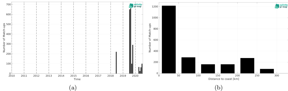
Figure 1: Number of match-ups between TSG (Lauge-Koch) and SMOS SSS L3 v8 - 9 Days (CATDS-CEC-LOCEAN) SSS as a function of time (a) and as function of the distance to coast (b) over the Arctic Ocean Pi-MEP region and for the full satellite product period.
