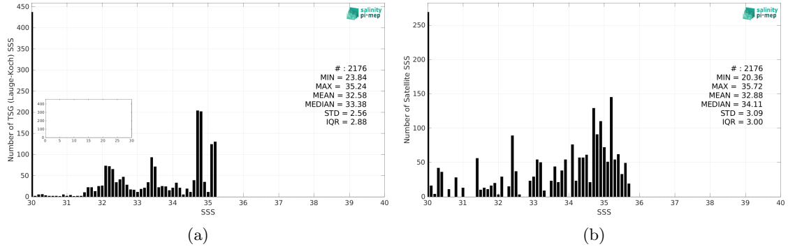
Figure 2: Histograms of SSS from TSG (Lauge-Koch) (a) and SMOS SSS L3 v8 - 9 Days (CATDS-CEC-LOCEAN) (b) considering all match-up pairs per bins of 0.1 over the Arctic Ocean Pi-MEP region and for the full satellite product period.
