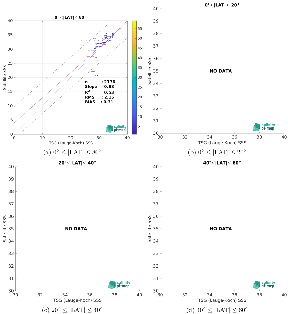
Figure 9: Contour maps of the concentration of SMOS SSS L3 v8 - 9 Days (CATDS-CEC-LOCEAN) SSS (y-axis) versus TSG (Lauge-Koch) SSS (x-axis) at match-up pairs for different latitude bands. For each plot, the red line shows x=y . The black thin and dashed lines indicate a linear fit through the data cloud and the \pm 95\% confidence levels, respectively. The number match-up pairs n , the slope and R^2 coefficient of the linear fit, the root mean square (RMS) and the mean bias between satellite and in situ data are indicated for each latitude band in each plots.
