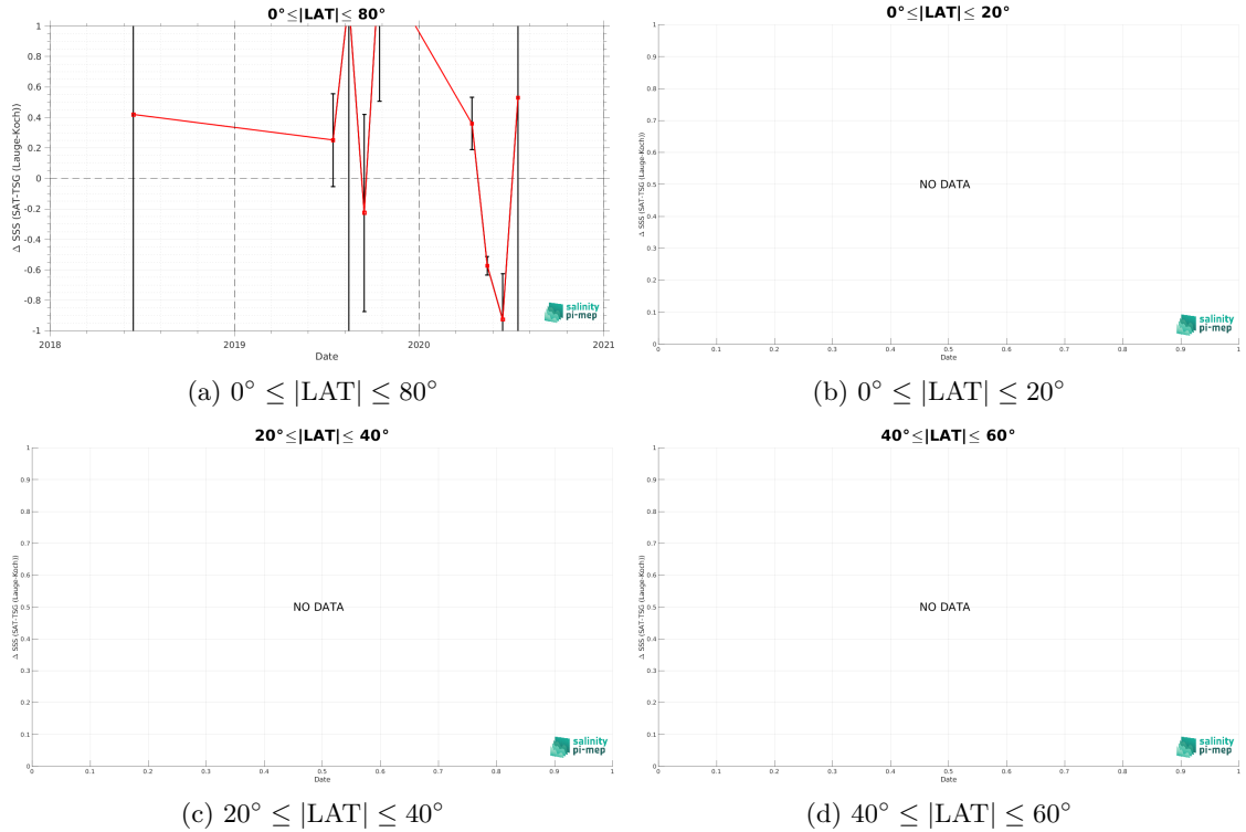
Figure 10: Monthly median (red curves) of \Delta SSS (Satellite - TSG (Lauge-Koch)) and \pm 1 Std (black vertical thick bars) as function of time for all the collected Pi-MEP match-up pairs estimated over the Arctic Ocean Pi-MEP region and for the full satellite product period are shown for different latitude bands: (a) 80^\circ\text{S}-80^\circ\text{N} , (b) 20^\circ\text{S}-20^\circ\text{N} , (c) 40^\circ\text{S}-20^\circ\text{S} and 20^\circ\text{N}-40^\circ\text{N} and (d) 60^\circ\text{S}-40^\circ\text{S} and 40^\circ\text{N}-60^\circ\text{N} .
