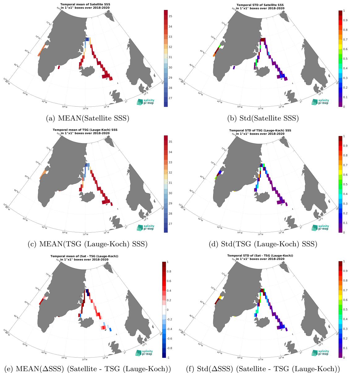
Figure 6: Temporal mean (left) and Std (right) of SSS from SMOS SSS L3 v8 - 9 Days (CATDS-CEC-LOCEAN) (top), TSG (Lauge-Koch) (middle), and of \Delta SSS (Satellite - TSG (Lauge-Koch)). Only match-up pairs are used to generate these maps.
