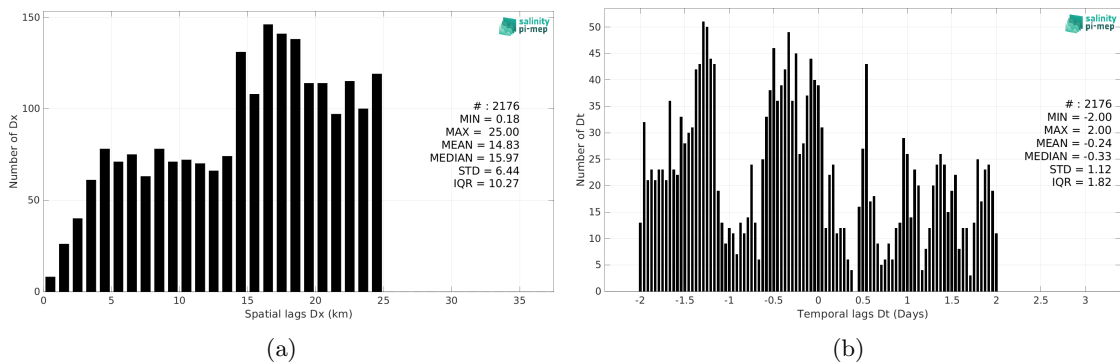
Figure 5: Histograms of the spatial (a) and temporal (b) lags between the location/time of the TSG (Lauge-Koch) measurement and the date of the corresponding SMOS SSS L3 v8 - 9 Days (CATDS-CEC-LOCEAN) SSS pixel.
