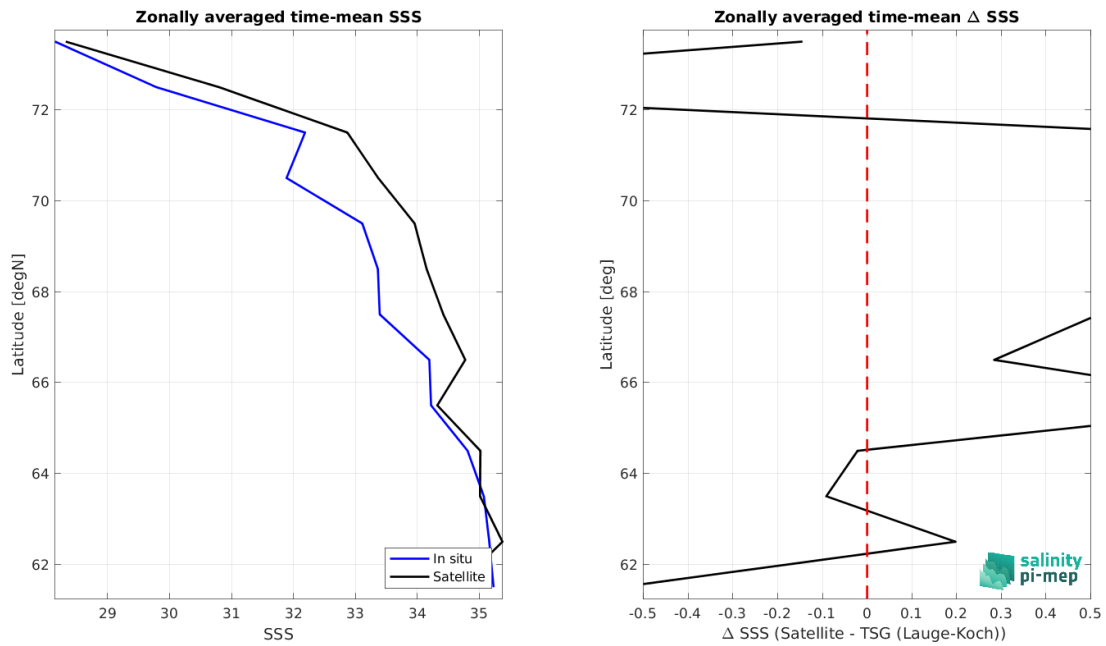
Figure 8: Left panel: Zonal mean SSS from SMOS SSS L3 v8 - 9 Days (CATDS-CEC-LOCEAN) satellite product (black) and from TSG (Lauge-Koch) (blue). Right panel: Zonal mean of \Delta SSS (Satellite - TSG (Lauge-Koch)) for all the collected Pi-MEP match-up pairs estimated over the full satellite product period.
