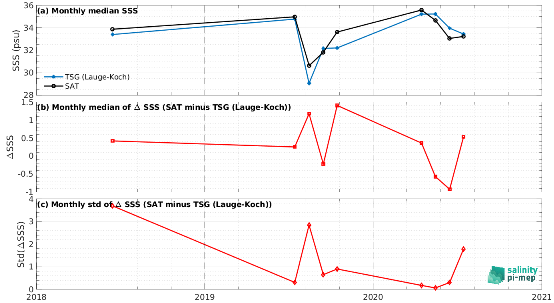
Figure 7: Time series of the monthly median SSS (top), median of \Delta SSS (Satellite - TSG (Lauge-Koch)) and Std of \Delta SSS (Satellite - TSG (Lauge-Koch)) over the Arctic Ocean Pi-MEP region considering all match-ups collected by the Pi-MEP.
