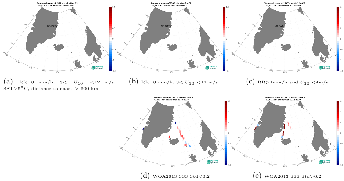
Figure 12: Temporal mean gridded over spatial boxes of size 1^{\circ}\times 1^{\circ} of \Delta\text{SSS} (SMOS SSS L3 v8 - 9 Days (CATDS-CEC-LOCEAN) - TSG (Lauge-Koch)) for 5 different subdatasets corresponding to:RR=0 mm/h, 3 < U_{10} < 12 m/s, SST > 5^{\circ}\text{C} , distance to coast > 800 km (a), RR=0 mm/h, 3 < U_{10} < 12 m/s (b), RR > 1 mm/h and U_{10} < 4 m/s (c), WOA2013 SSS Std < 0.2 (d), WOA2013 SSS Std > 0.2 (e).
