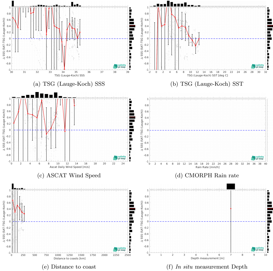
Figure 11: \Delta SSS (Satellite - TSG (Lauge-Koch)) sorted as function of TSG (Lauge-Koch) SSS values a), TSG (Lauge-Koch) SST b), ASCAT Wind speed c), CMORPH rain rate d), distance to coast (e) and in situ measurement depth (f). In all plots the median and Std of \Delta SSS for each bin is indicated by the red curves and black vertical thick bars ( \pm 1 Std)
