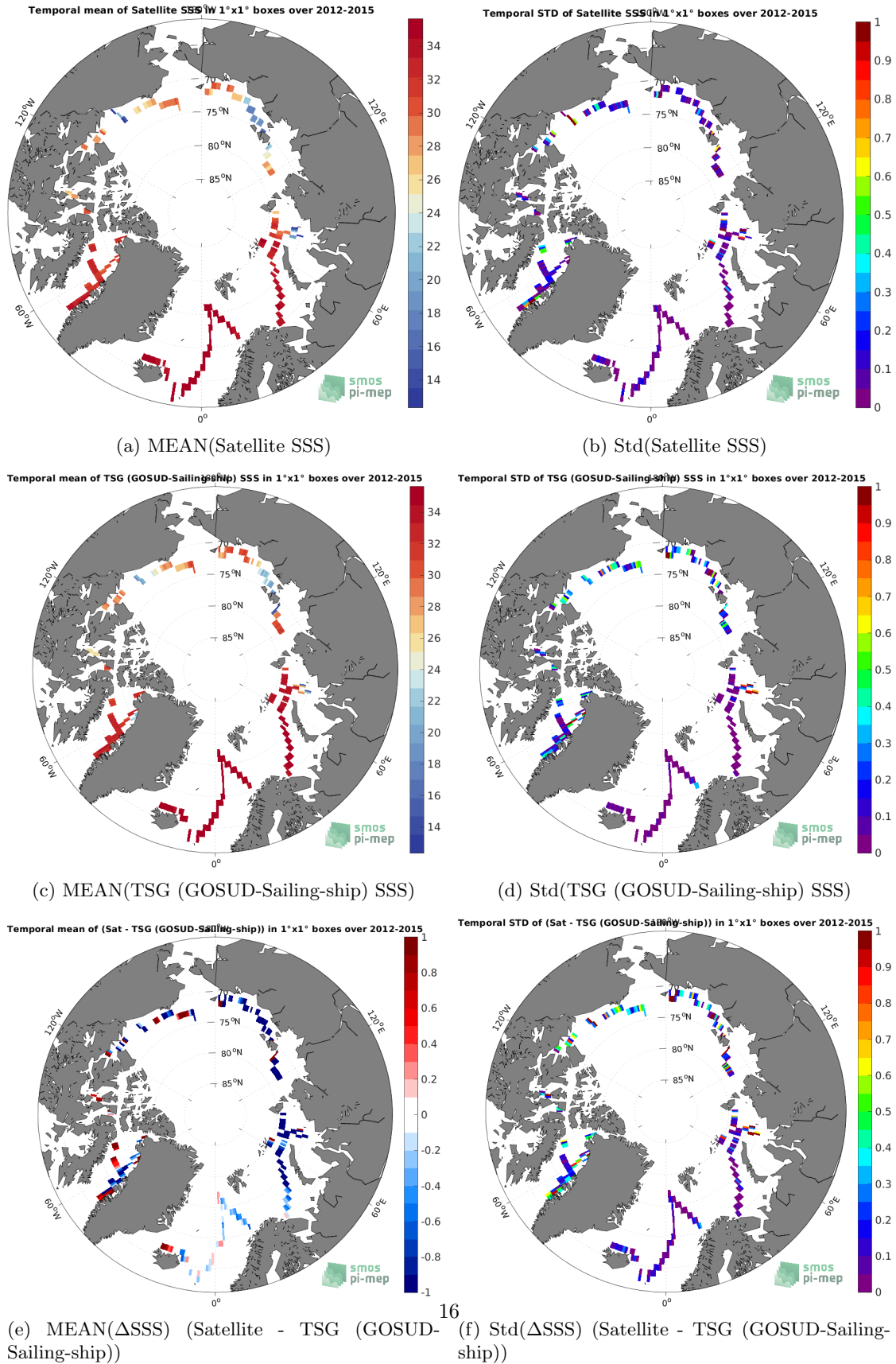
Figure 6: Temporal mean (left) and Std (right) of SSS from SMOS SSS L3 v8 - 9 Days (CATDS-CECOS-LOCEAN) (top), TSG (GOSUD-Sailing-ship) (middle), and of \Delta SSS (Satellite - TSG (GOSUD-Sailing-ship)). Only match-up pairs are used to generate these maps.
