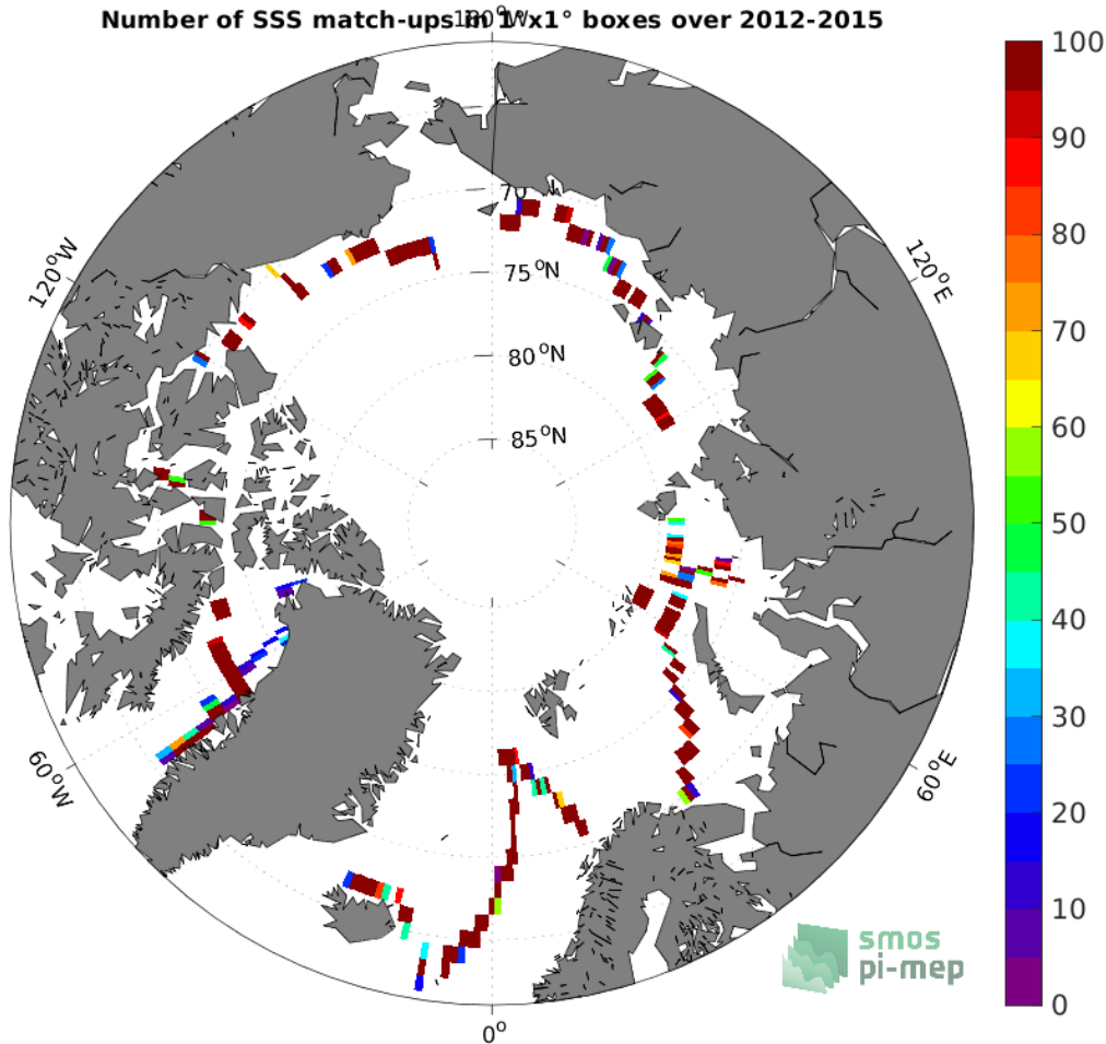
Figure 4: Number of SSS match-ups between TSG (GOSUD-Sailing-ship) SSS and the SMOS SSS L3 v8 - 9 Days (CATDS-CECOS-LOCEAN) SSS product for the Arctic Ocean Pi-MEP region over 1^\circ \times 1^\circ boxes and for the full satellite product period.
