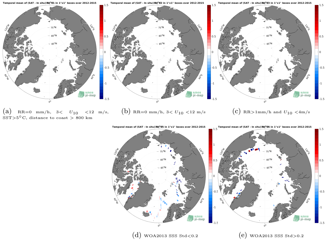
Figure 12: Temporal mean gridded over spatial boxes of size 1^\circ \times 1^\circ of \Delta SSS (SMOS SSS L3 v8 - 9 Days (CATDS-CECOS-LOCEAN) - TSG (GOSUD-Sailing-ship)) for 5 different subdatasets corresponding to: RR=0 mm/h, 3 < U_{10} < 12 m/s, SST > 5°C, distance to coast > 800 km (a), RR=0 mm/h, 3 < U_{10} < 12 m/s (b), RR > 1mm/h and U_{10} < 4 m/s (c), WOA2013 SSS Std < 0.2 (d), WOA2013 SSS Std > 0.2 (e).
