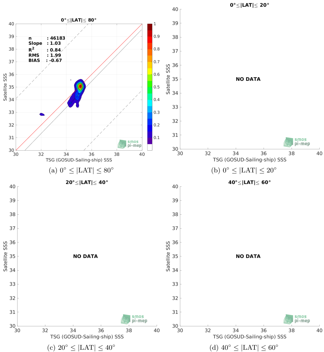
Figure 9: Contour maps of the concentration of SMOS SSS L3 v8 - 9 Days (CATDS-CECOS-LOCEAN) SSS (y-axis) versus TSG (GOSUD-Sailing-ship) SSS (x-axis) at match-up pairs for different latitude bands. For each plot, the red line shows x=y . The black thin and dashed lines indicate a linear fit through the data cloud and the \pm 95\% confidence levels, respectively. The number match-up pairs n , the slope and R^2 coefficient of the linear fit, the root mean square (RMS) and the mean bias between satellite and in situ data are indicated for each latitude band in each plots.
