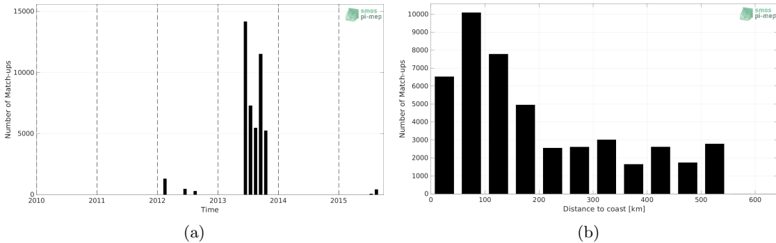
Figure 1: Number of match-ups between TSG (GOSUD-Sailing-ship) and SMOS SSS L3 v8 - 9 Days (CATDS-CECOS-LOCEAN) SSS as a function of time (a) and as function of the distance to coast (b) over the Arctic Ocean Pi-MEP region and for the full satellite product period.
