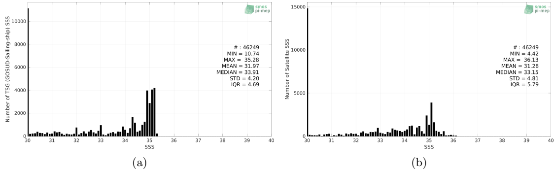
Figure 2: Histograms of SSS from TSG (GOSUD-Sailing-ship) (a) and SMOS SSS L3 v8 - 9 Days (CATDS-CECOS-LOCEAN) (b) considering all match-up pairs per bins of 0.1 over the Arctic Ocean Pi-MEP region and for the full satellite product period.
