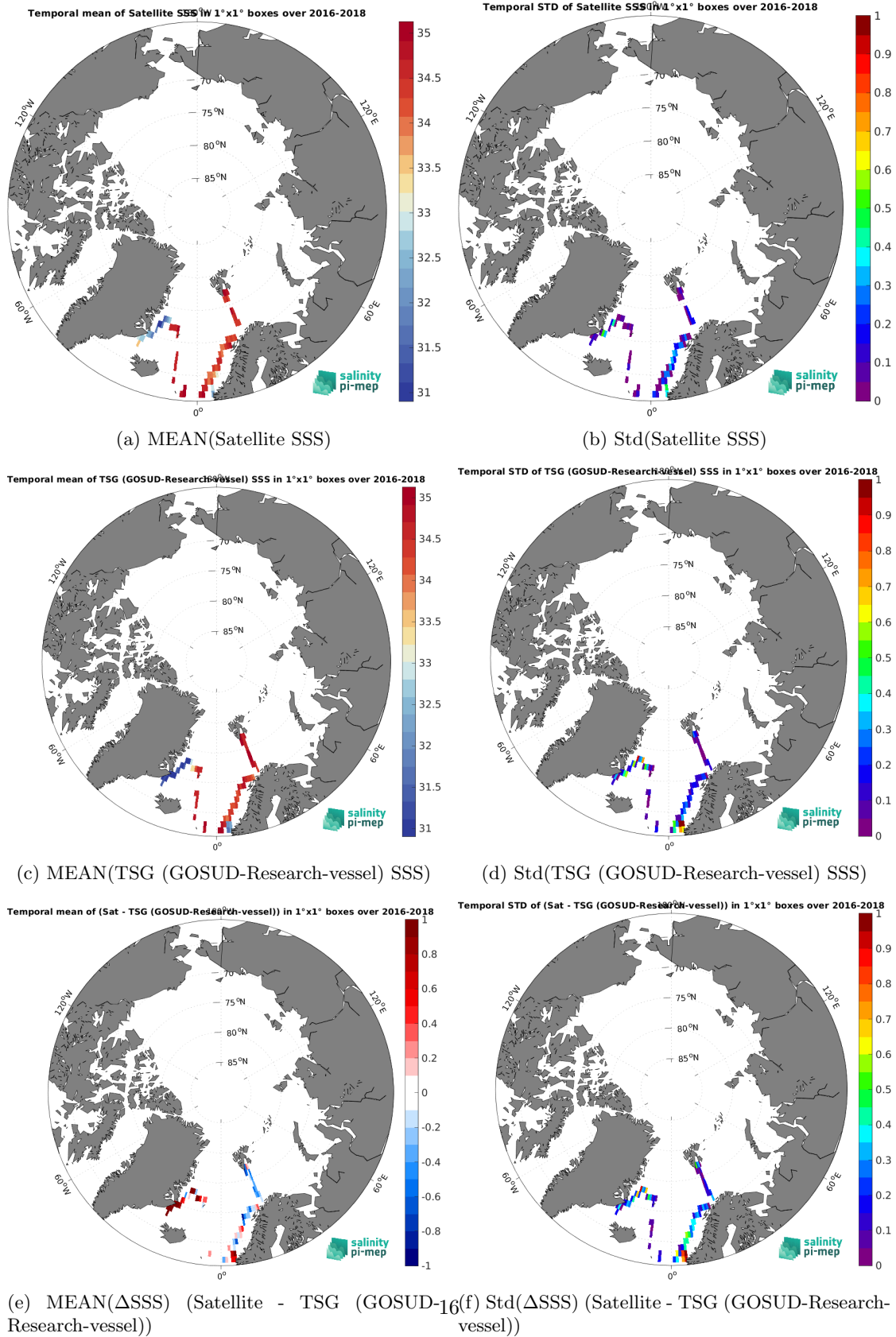
Figure 6: Temporal mean (left) and Std (right) of SSS from SMOS SSS L3 v8 - 9 Days (CATDS-CEC-LOCEAN) (top), TSG (GOSUD-Research-vessel) (middle), and of \Delta SSS (Satellite - TSG (GOSUD-Research-vessel)). Only match-up pairs are used to generate these maps.
