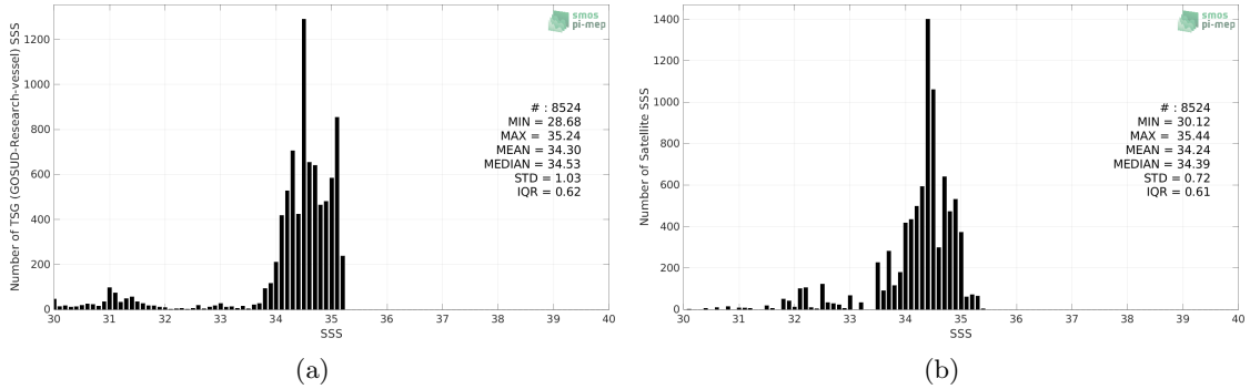
Figure 2: Histograms of SSS from TSG (GOSUD-Research-vessel) (a) and SMOS SSS L3 v8 - 9 Days (CATDS-CECOS-LOCEAN) (b) considering all match-up pairs per bins of 0.1 over the Arctic Ocean Pi-MEP region and for the full satellite product period.
