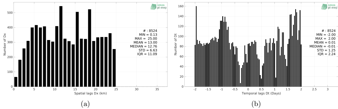
Figure 5: Histograms of the spatial (a) and temporal (b) lags between the location/time of the TSG (GOSUD-Research-vessel) measurement and the date of the corresponding SMOS SSS L3 v8 - 9 Days (CATDS-CECOS-LOCEAN) SSS pixel.
