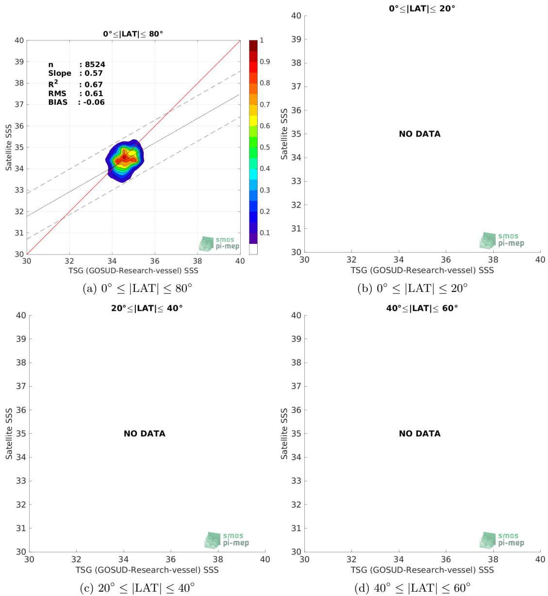
Figure 9: Contour maps of the concentration of SMOS SSS L3 v8 - 9 Days (CATDS-CECOS-LOCEAN) SSS (y-axis) versus TSG (GOSUD-Research-vessel) SSS (x-axis) at match-up pairs for different latitude bands. For each plot, the red line shows x=y . The black thin and dashed lines indicate a linear fit through the data cloud and the \pm 95\% confidence levels, respectively. The number match-up pairs n , the slope and R^2 coefficient of the linear fit, the root mean square (RMS) and the mean bias between satellite and in situ data are indicated for each latitude band in each plots.
