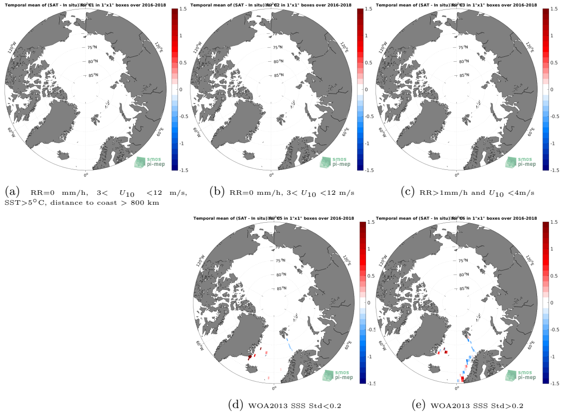
Figure 12: Temporal mean gridded over spatial boxes of size 1^\circ \times 1^\circ of \Delta SSS (SMOS SSS L3 v8 - 9 Days (CATDS-CECOS-LOCEAN) - TSG (GOSUD-Research-vessel)) for 5 different subdatasets corresponding to: RR=0 mm/h, 3 < U_{10} < 12 m/s, SST > 5°C, distance to coast > 800 km (a), RR=0 mm/h, 3 < U_{10} < 12 m/s (b), RR > 1mm/h and U_{10} < 4 m/s (c), WOA2013 SSS Std < 0.2 (d), WOA2013 SSS Std > 0.2 (e).
