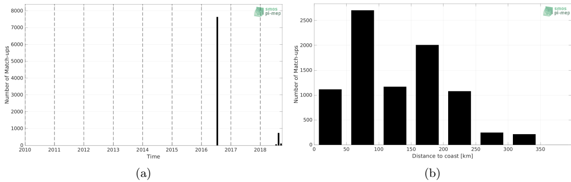
Figure 1: Number of match-ups between TSG (GOSUD-Research-vessel) and SMOS SSS L3 v8 - 9 Days (CATDS-CECOS-LOCEAN) SSS as a function of time (a) and as function of the distance to coast (b) over the Arctic Ocean Pi-MEP region and for the full satellite product period.
