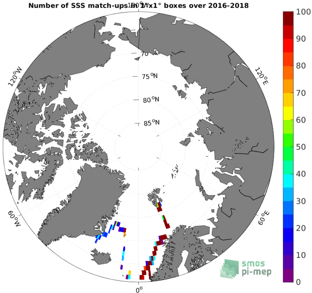
Figure 4: Number of SSS match-ups between TSG (GOSUD-Research-vessel) SSS and the SMOS SSS L3 v8 - 9 Days (CATDS-CECOS-LOCEAN) SSS product for the Arctic Ocean Pi-MEP region over 1^\circ \times 1^\circ boxes and for the full satellite product period.
