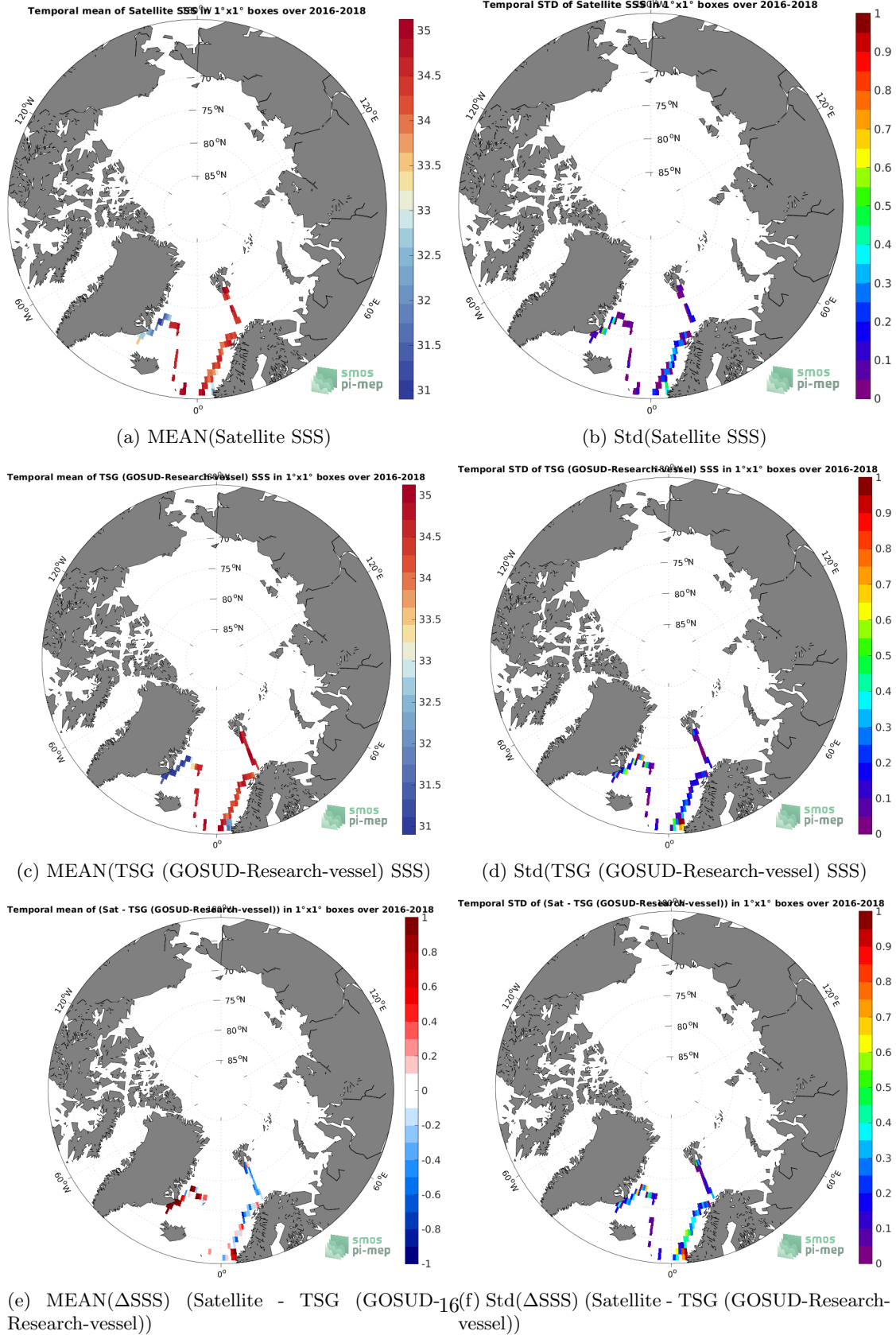
Figure 6: Temporal mean (left) and Std (right) of SSS from SMOS SSS L3 v8 - 9 Days (CATDS-CECOS-LOCEAN) (top), TSG (GOSUD-Research-vessel) (middle), and of \Delta SSS (Satellite - TSG (GOSUD-Research-vessel)). Only match-up pairs are used to generate these maps.
