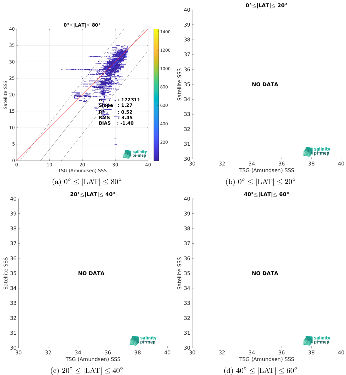
Figure 9: Contour maps of the concentration of SMOS SSS L3 v8 - 9 Days (CATDS-CEC-LOCEAN) SSS (y-axis) versus TSG (Amundsen) SSS (x-axis) at match-up pairs for different latitude bands. For each plot, the red line shows x=y . The black thin and dashed lines indicate a linear fit through the data cloud and the \pm 95\% confidence levels, respectively. The number match-up pairs n , the slope and R^2 coefficient of the linear fit, the root mean square (RMS) and the mean bias between satellite and in situ data are indicated for each latitude band in each plots.
