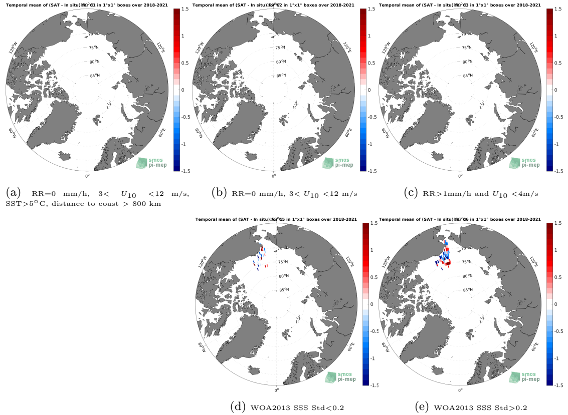
Figure 12: Temporal mean gridded over spatial boxes of size 1^{\circ}\times 1^{\circ} of \Delta\text{SSS} (SMOS SSS L3 v8 - 9 Days (CATDS-CECOS-LOCEAN) - Saildrone) for 5 different subdatasets corresponding to:RR=0 mm/h, 3 < U_{10} < 12 m/s, SST > 5^{\circ}\text{C} , distance to coast > 800 km (a), RR=0 mm/h, 3 < U_{10} < 12 m/s (b), RR > 1 mm/h and U_{10} < 4 m/s (c), WOA2013 SSS Std < 0.2 (d), WOA2013 SSS Std > 0.2 (e).
