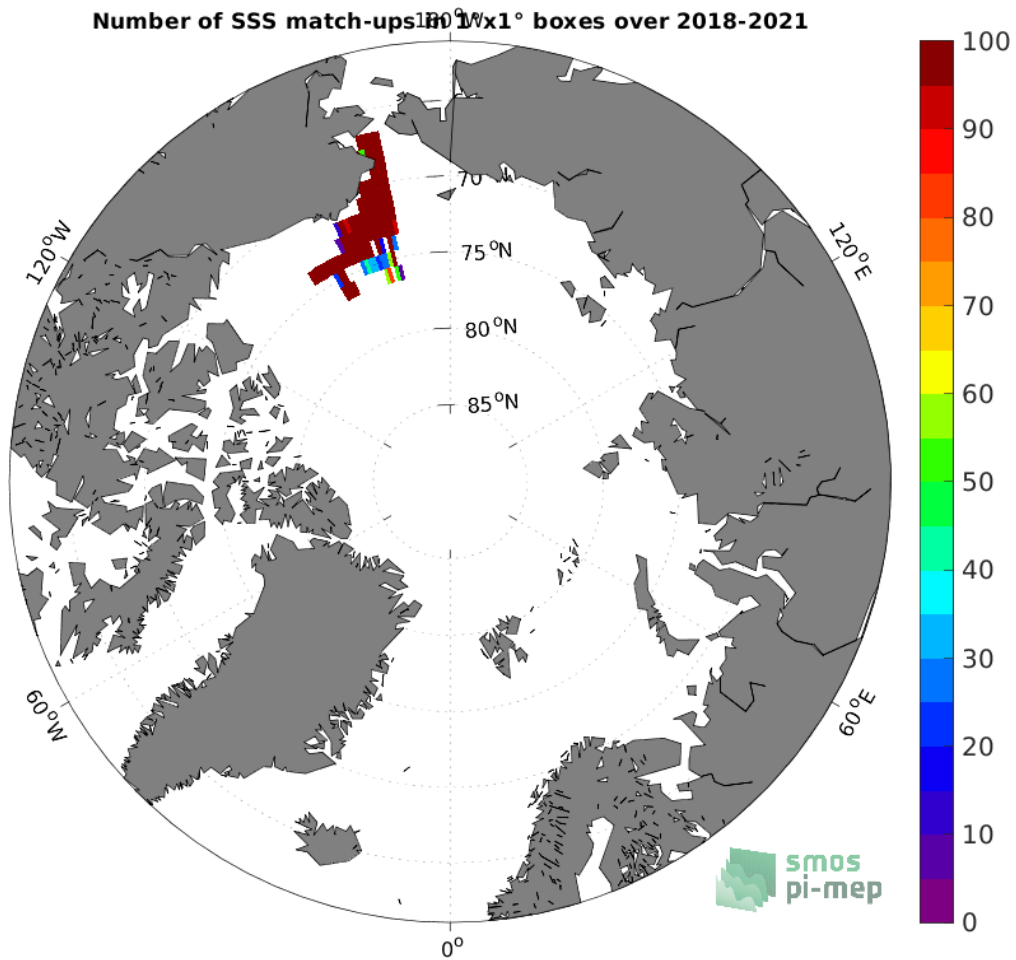
Figure 4: Number of SSS match-ups between Sailldrone SSS and the SMOS SSS L3 v8 - 9 Days (CATDS-CECOS-LOCEAN) SSS product for the Arctic Ocean Pi-MEP region over 1^\circ \times 1^\circ boxes and for the full satellite product period.
