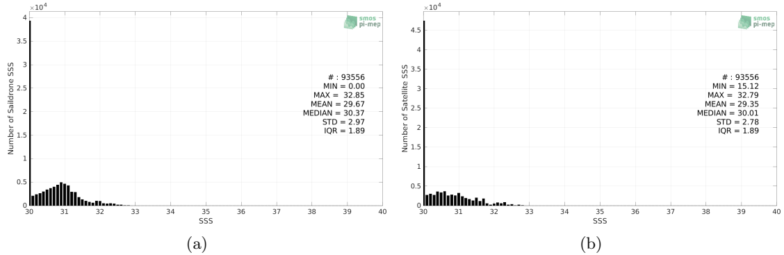
Figure 2: Histograms of SSS from Sairdrone (a) and SMOS SSS L3 v8 - 9 Days (CATDS-CECOS-LOCEAN) (b) considering all match-up pairs per bins of 0.1 over the Arctic Ocean Pi-MEP region and for the full satellite product period.
