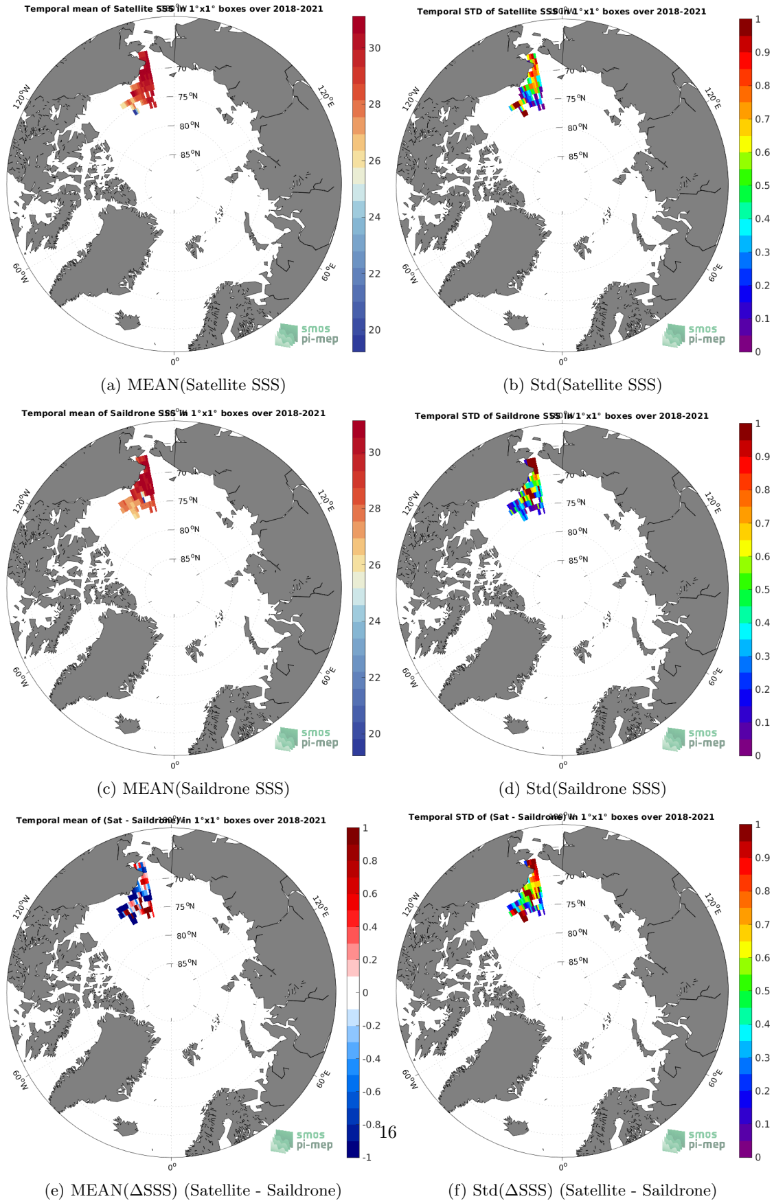
Figure 6: Temporal mean (left) and Std (right) of SSS from SMOS SSS L3 v8 - 9 Days (CATDS-CECOS-LOCEAN) (top), Saildrone (middle), and of \Delta SSS (Satellite - Saildrone). Only match-pairs are used to generate these maps.
