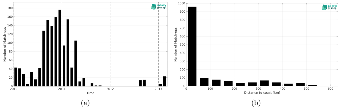
Figure 1: Number of match-ups between Marine mammals and SMOS SSS L3 v8 - 9 Days (CATDS-CEC-LOCEAN) SSS as a function of time (a) and as function of the distance to coast (b) over the Arctic Ocean Pi-MEP region and for the full satellite product period.
