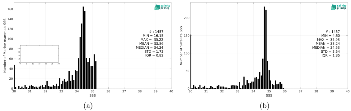
Figure 2: Histograms of SSS from Marine mammals (a) and SMOS SSS L3 v8 - 9 Days (CATDS-CEC-LOCEAN) (b) considering all match-up pairs per bins of 0.1 over the Arctic Ocean Pi-MEP region and for the full satellite product period.
