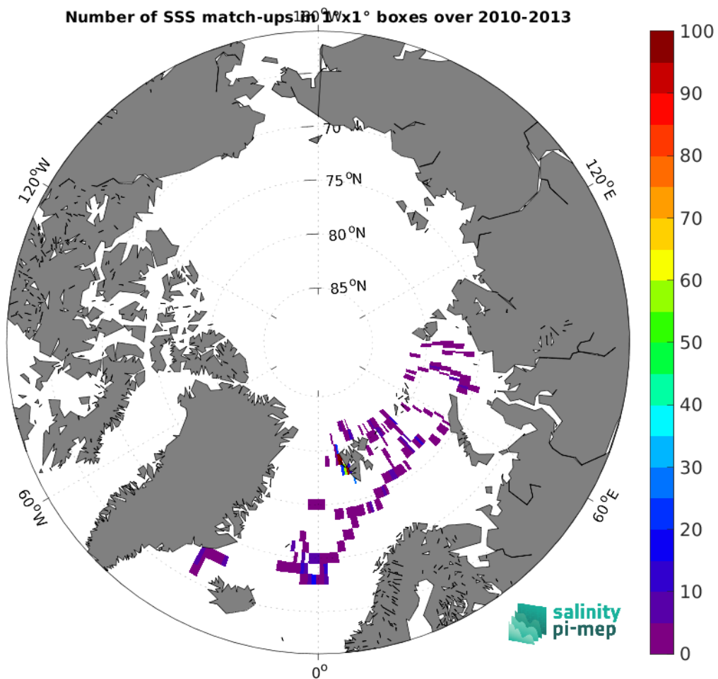
Figure 4: Number of SSS match-ups between Marine mammals SSS and the SMOS SSS L3 v8 - 9 Days (CATDS-CEC-LOCEAN) SSS product for the Arctic Ocean Pi-MEP region over 1^\circ \times 1^\circ boxes and for the full satellite product period.
