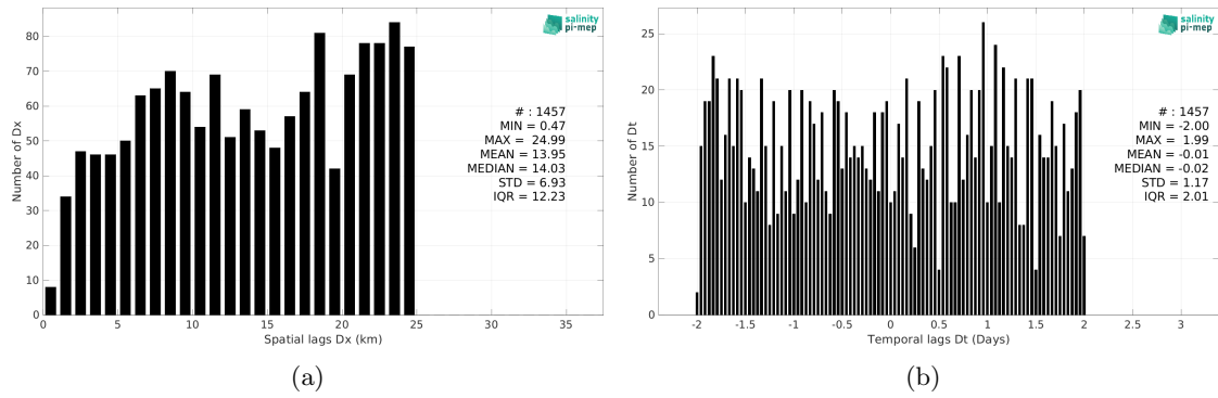
Figure 5: Histograms of the spatial (a) and temporal (b) lags between the location/time of the Marine mammals measurement and the date of the corresponding SMOS SSS L3 v8 - 9 Days (CATDS-CEC-LOCEAN) SSS pixel.
