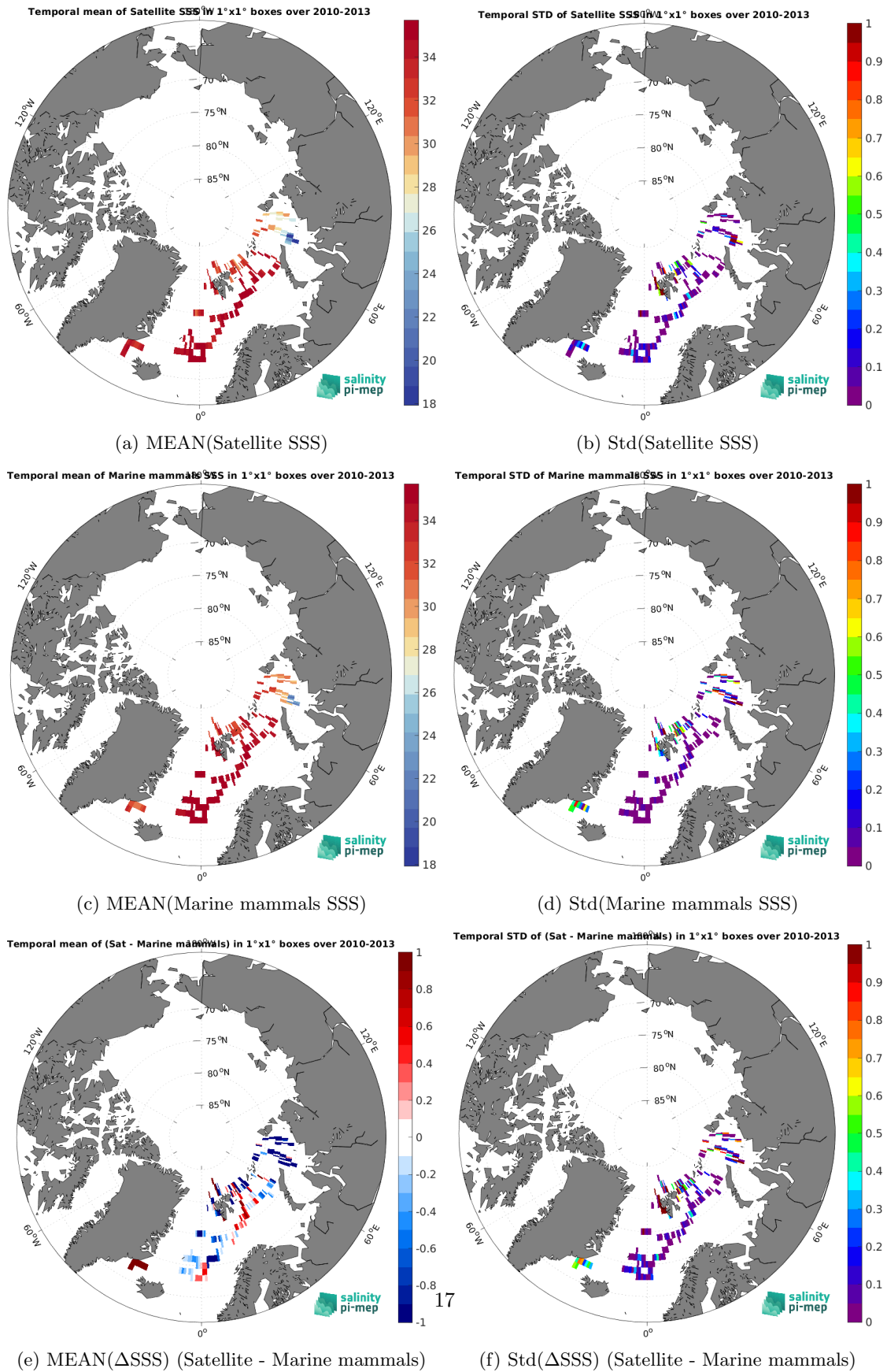
Figure 6: Temporal mean (left) and Std (right) of SSS from SMOS SSS L3 v8 - 9 Days (CATDS-CEC-LOCEAN) (top), Marine mammals (middle), and of \Delta SSS (Satellite - Marine mammals). Only match-up pairs are used to generate these maps.
