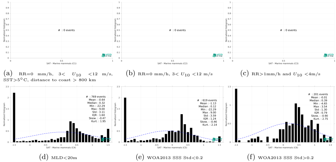
Figure 13: Normalized histogram of \Delta\text{SSS} (SMOS SSS L3 v8 - 9 Days (CATDS-CEC-LOCEAN) - Marine mammals) for 6 different subdatasets corresponding to: RR=0 mm/h, 3 < U_{10} < 12 m/s, SST > 5^\circ\text{C} , distance to coast > 800 km (a), RR=0 mm/h, 3 < U_{10} < 12 m/s (b), RR > 1\text{mm/h} and U_{10} < 4\text{m/s} (c), MLD < 20\text{m} (d), WOA2013 SSS Std < 0.2 (e), WOA2013 SSS Std > 0.2 (f).
