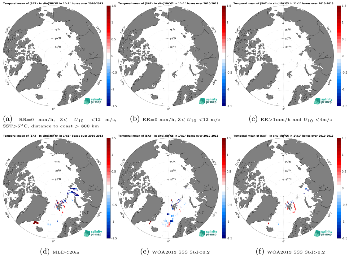
Figure 12: Temporal mean gridded over spatial boxes of size 1^{\circ}\times 1^{\circ} of \Delta\text{SSS} (SMOS SSS L3 v8 - 9 Days (CATDS-CEC-LOCEAN) - Marine mammals) for 6 different subdatasets corresponding to:RR=0 mm/h, 3 < U_{10} < 12 m/s, SST > 5^{\circ}\text{C} , distance to coast > 800 km (a), RR=0 mm/h, 3 < U_{10} < 12 m/s (b), RR > 1\text{mm/h} and U_{10} < 4\text{m/s} (c),MLD < 20\text{m} (d),WOA2013 SSS Std < 0.2 (e),WOA2013 SSS Std > 0.2 (f).
