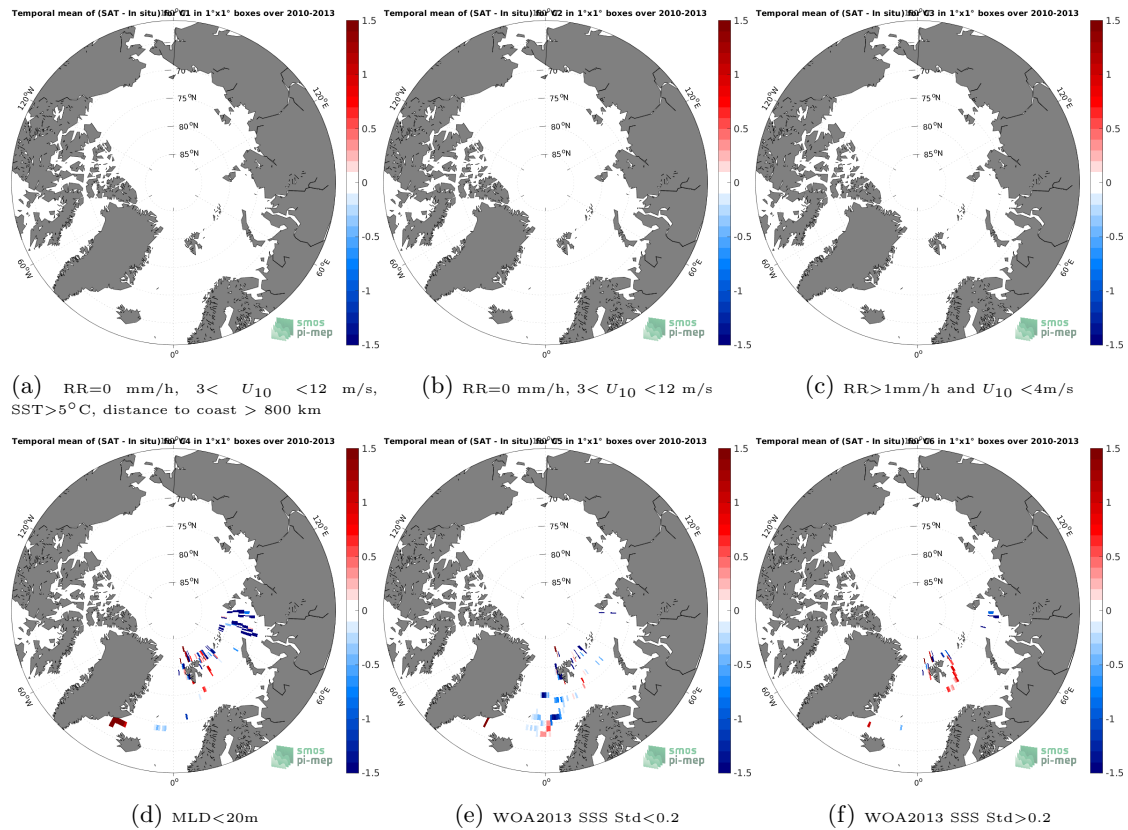
Figure 12: Temporal mean gridded over spatial boxes of size 1^{\circ}\times 1^{\circ} of \Delta\text{SSS} (SMOS SSS L3 v8 - 9 Days (CATDS-CECOS-LOCEAN) - Marine mammals) for 6 different subdatasets corresponding to:RR=0 mm/h, 3 < U_{10} < 12 m/s, SST >5^{\circ}\text{C} , distance to coast > 800 km (a), RR=0 mm/h, 3 < U_{10} < 12 m/s (b), RR >1 mm/h and U_{10} < 4 m/s (c),MLD <20 m (d),WOA2013 SSS Std <0.2 (e),WOA2013 SSS Std >0.2 (f).
