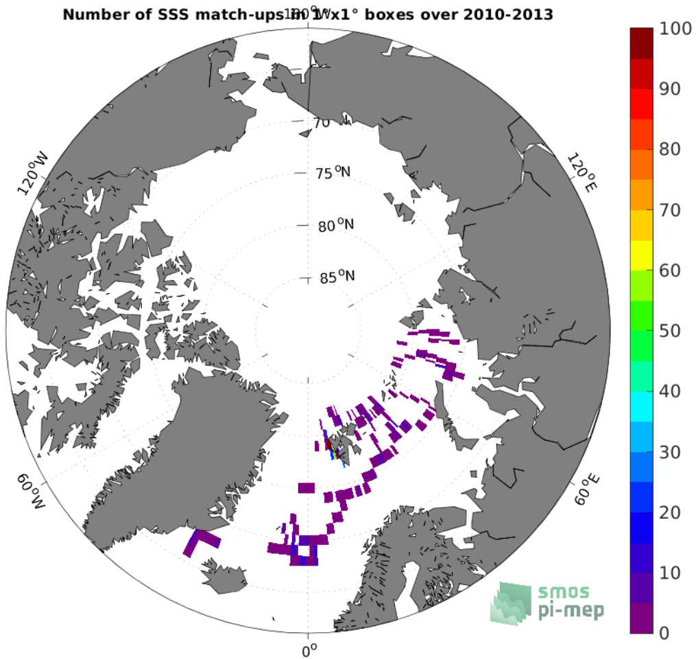
Figure 4: Number of SSS match-ups between Marine mammals SSS and the SMOS SSS L3 v8 - 9 Days (CATDS-CECOS-LOCEAN) SSS product for the Arctic Ocean Pi-MEP region over 1^\circ \times 1^\circ boxes and for the full satellite product period.
