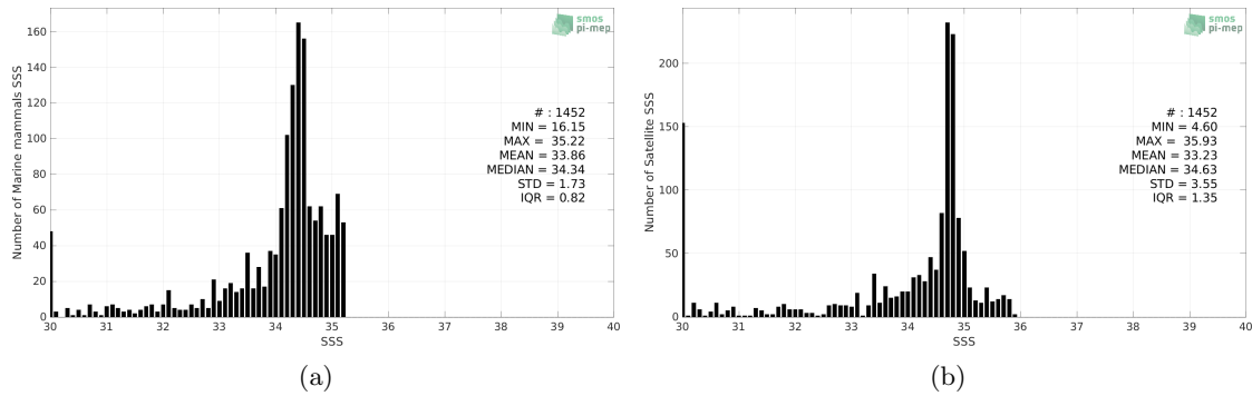
Figure 2: Histograms of SSS from Marine mammals (a) and SMOS SSS L3 v8 - 9 Days (CATDS-CECOS-LOCEAN) (b) considering all match-up pairs per bins of 0.1 over the Arctic Ocean Pi-MEP region and for the full satellite product period.
