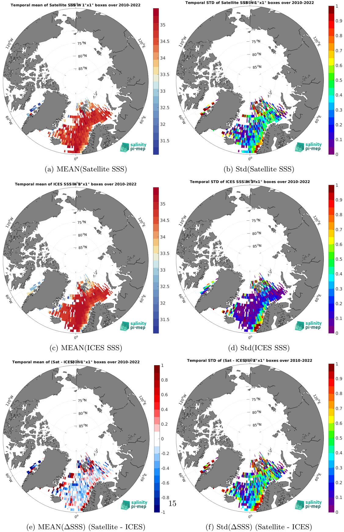
Figure 6: Temporal mean (left) and Std (right) of SSS from SMOS SSS L3 v8 - 9 Days (CATDS-CEC-LOCEAN) (top), ICES (middle), and of \Delta SSS (Satellite - ICES). Only match-up pairs are used to generate these maps.
