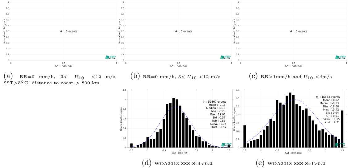
Figure 13: Normalized histogram of \Delta SSS (SMOS SSS L3 v8 - 9 Days (CATDS-CEC-LOCEAN) - ICES) for 5 different subdatasets corresponding to: RR=0 mm/h, 3 < U_{10} < 12 m/s, SST > 5°C, distance to coast > 800 km (a), RR=0 mm/h, 3 < U_{10} < 12 m/s (b), RR > 1mm/h and U_{10} < 4 m/s (c), WOA2013 SSS Std < 0.2 (d), WOA2013 SSS Std > 0.2 (e).
