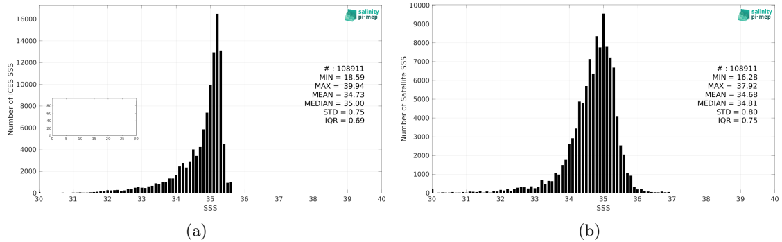
Figure 2: Histograms of SSS from ICES (a) and SMOS SSS L3 v8 - 9 Days (CATDS-CEC-LOCEAN) (b) considering all match-up pairs per bins of 0.1 over the Arctic Ocean Pi-MEP region and for the full satellite product period.
