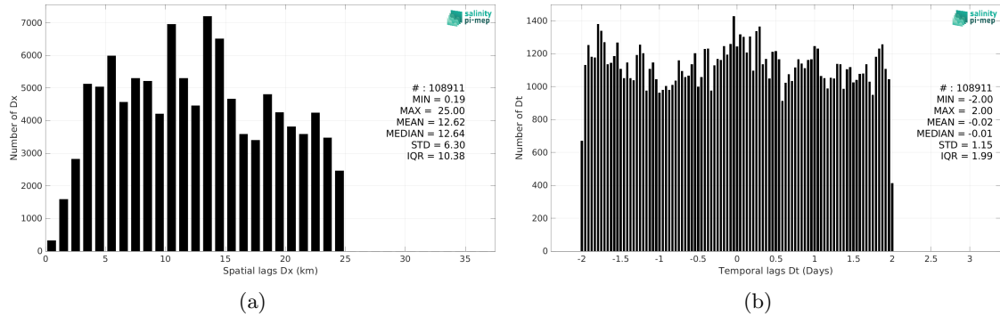
Figure 5: Histograms of the spatial (a) and temporal (b) lags between the location/time of the ICES measurement and the date of the corresponding SMOS SSS L3 v8 - 9 Days (CATDS-CEC-LOCEAN) SSS pixel.
