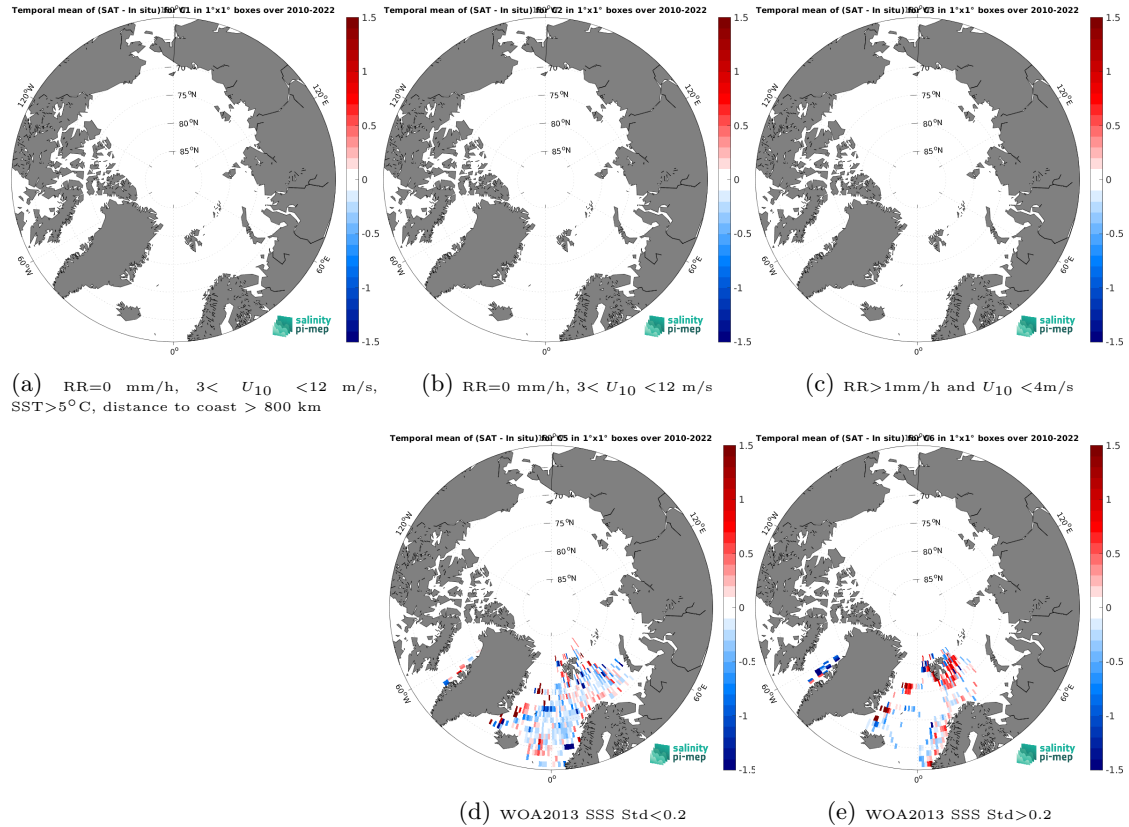
Figure 12: Temporal mean gridded over spatial boxes of size 1^{\circ}\times 1^{\circ} of \Delta\text{SSS} (SMOS SSS L3 v8 - 9 Days (CATDS-CEC-LOCEAN) - ICES) for 5 different subdatasets corresponding to:RR=0 mm/h, 3 < U_{10} < 12 m/s, SST > 5^{\circ}\text{C} , distance to coast > 800 km (a), RR=0 mm/h, 3 < U_{10} < 12 m/s (b), RR > 1 mm/h and U_{10} < 4 m/s (c), WOA2013 SSS Std < 0.2 (d), WOA2013 SSS Std > 0.2 (e).
