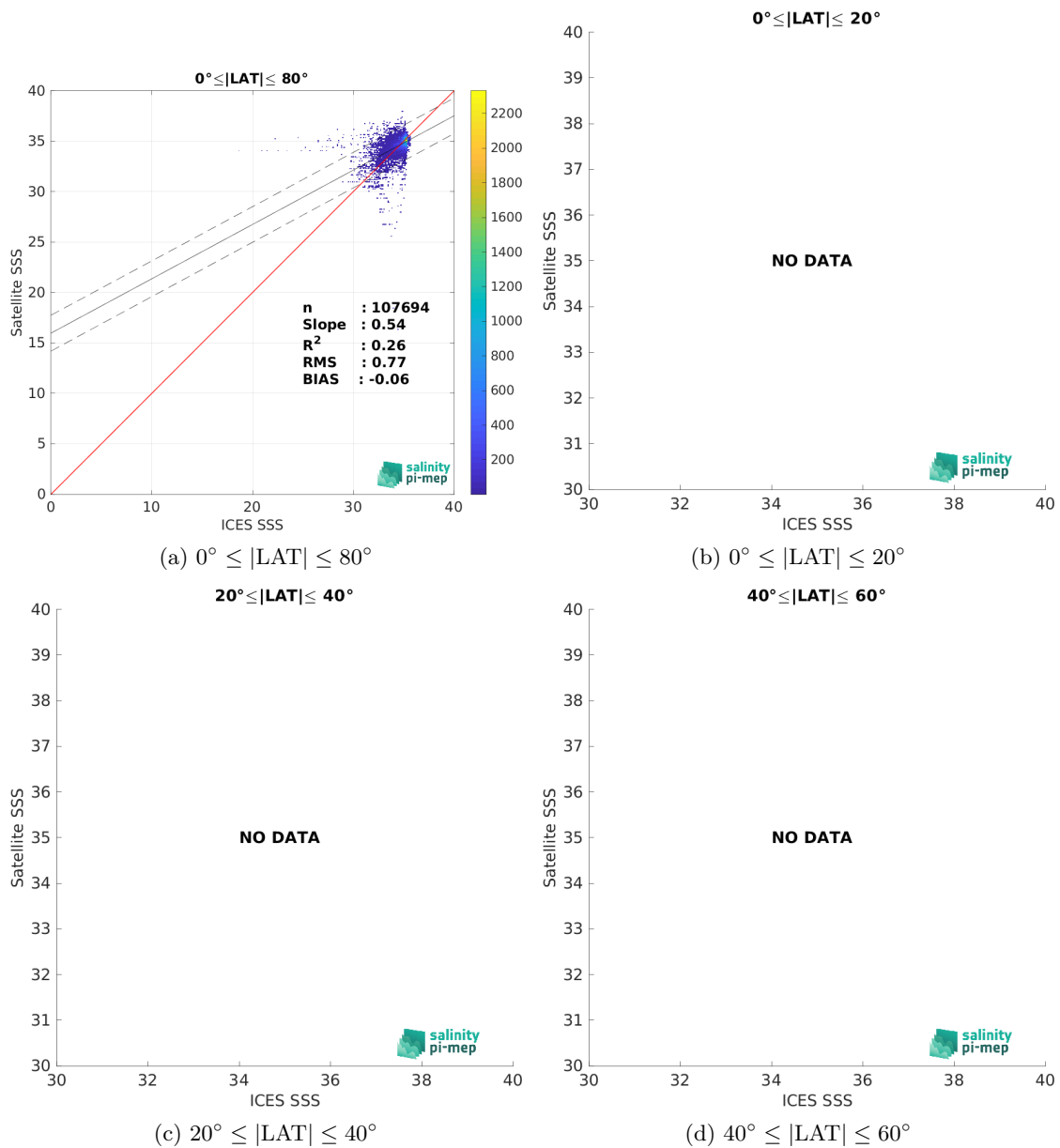
Figure 9: Contour maps of the concentration of SMOS SSS L3 v8 - 9 Days (CATDS-CEC-LOCEAN) SSS (y-axis) versus ICES SSS (x-axis) at match-up pairs for different latitude bands. For each plot, the red line shows x=y . The black thin and dashed lines indicate a linear fit through the data cloud and the \pm 95\% confidence levels, respectively. The number match-up pairs n , the slope and R^2 coefficient of the linear fit, the root mean square (RMS) and the mean bias between satellite and in situ data are indicated for each latitude band in each plots.
