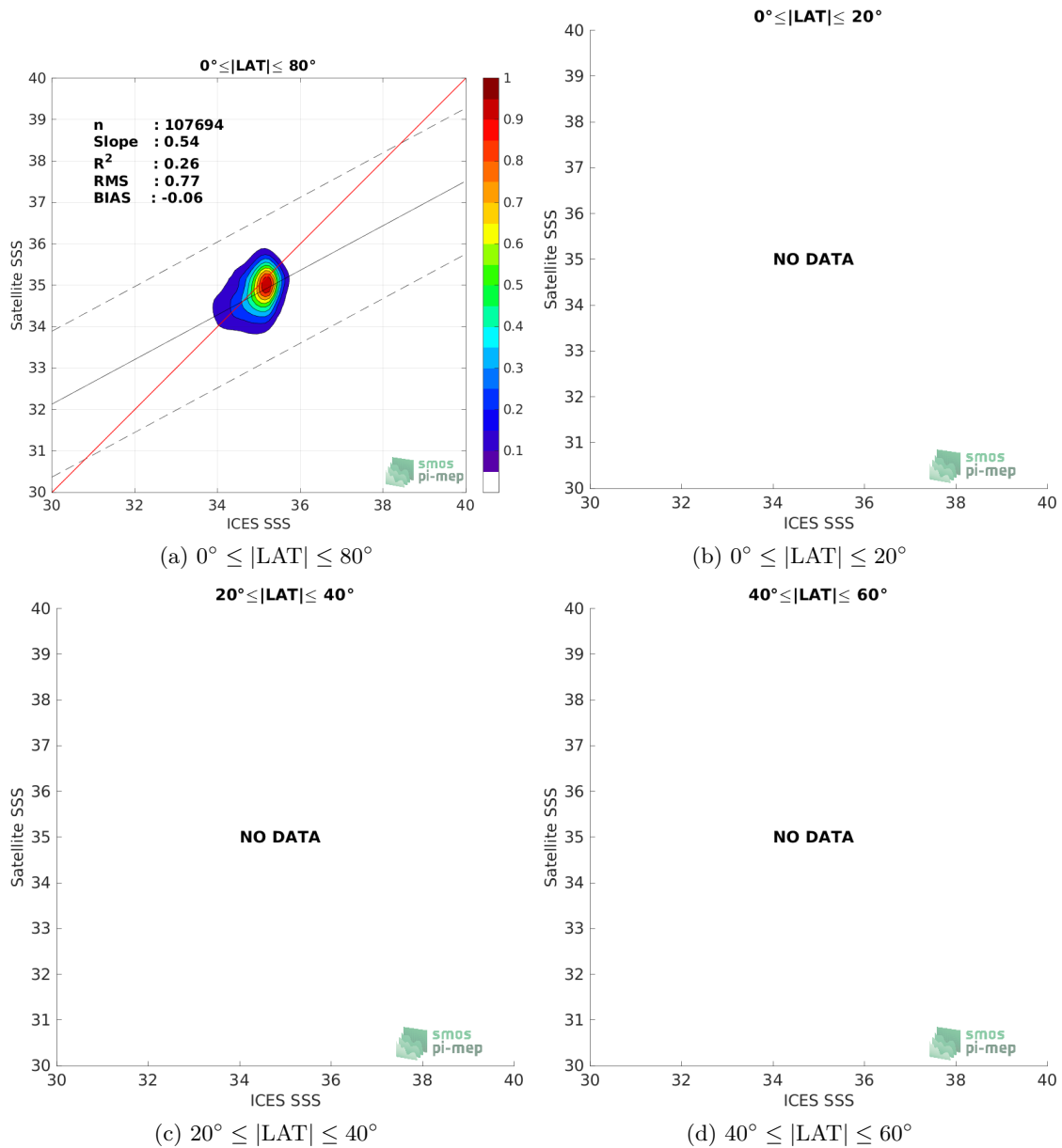
Figure 9: Contour maps of the concentration of SMOS SSS L3 v8 - 9 Days (CATDS-CECOS-LOCEAN) SSS (y-axis) versus ICES SSS (x-axis) at match-up pairs for different latitude bands. For each plot, the red line shows x=y . The black thin and dashed lines indicate a linear fit through the data cloud and the \pm 95\% confidence levels, respectively. The number match-up pairs n , the slope and R^2 coefficient of the linear fit, the root mean square (RMS) and the mean bias between satellite and in situ data are indicated for each latitude band in each plots.
