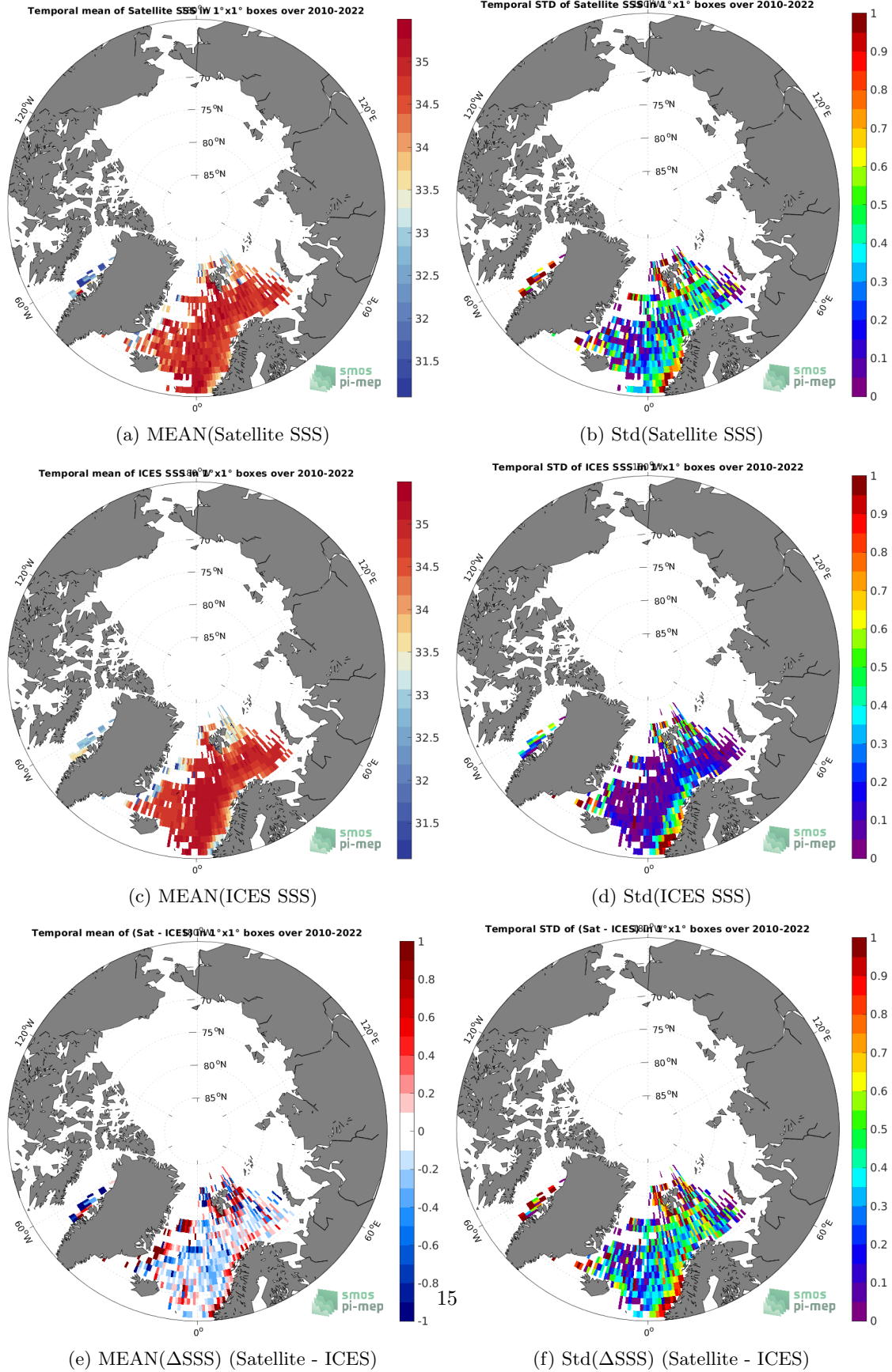
Figure 6: Temporal mean (left) and Std (right) of SSS from SMOS SSS L3 v8 - 9 Days (CATDS-CECOS-LOCEAN) (top), ICES (middle), and of \Delta SSS (Satellite - ICES). Only match-up pairs are used to generate these maps.
