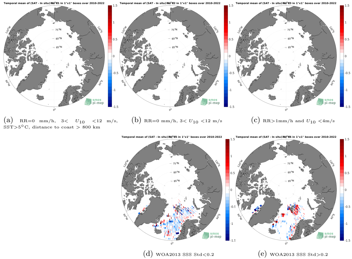
Figure 12: Temporal mean gridded over spatial boxes of size 1^{\circ}\times 1^{\circ} of \Delta\text{SSS} (SMOS SSS L3 v8 - 9 Days (CATDS-CECOS-LOCEAN) - ICES) for 5 different subdatasets corresponding to:RR=0 mm/h, 3 < U_{10} < 12 m/s, SST > 5^{\circ}\text{C} , distance to coast > 800 km (a), RR=0 mm/h, 3 < U_{10} < 12 m/s (b), RR > 1 mm/h and U_{10} < 4 m/s (c), WOA2013 SSS Std < 0.2 (d), WOA2013 SSS Std > 0.2 (e).
