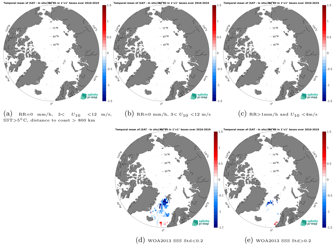
Figure 11: Temporal mean gridded over spatial boxes of size 1^{\circ}\times 1^{\circ} of \Delta\text{SSS} (SMOS SSS L3 v8 - 9 Days (CATDS-CEC-LOCEAN) - Surface drifters) for 5 different subdatasets corresponding to:RR=0 mm/h, 3 < U_{10} < 12 m/s, SST >5^{\circ}\text{C} , distance to coast > 800 km (a), RR=0 mm/h, 3 < U_{10} < 12 m/s (b), RR >1 mm/h and U_{10} < 4 m/s (c), WOA2013 SSS Std <0.2 (d), WOA2013 SSS Std >0.2 (e).
