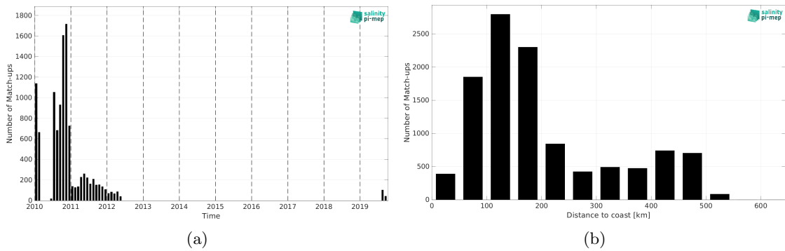
Figure 1: Number of match-ups between Surface drifters and SMOS SSS L3 v8 - 9 Days (CATDS-CEC-LOCEAN) SSS as a function of time (a) and as function of the distance to coast (b) over the Arctic Ocean Pi-MEP region and for the full satellite product period.
