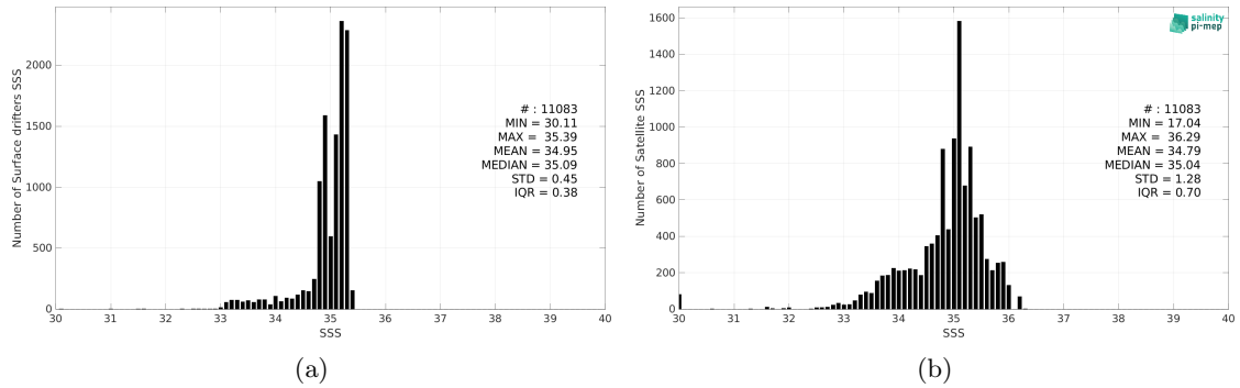
Figure 2: Histograms of SSS from Surface drifters (a) and SMOS SSS L3 v8 - 9 Days (CATDS-CEC-LOCEAN) (b) considering all match-up pairs per bins of 0.1 over the Arctic Ocean Pi-MEP region and for the full satellite product period.
