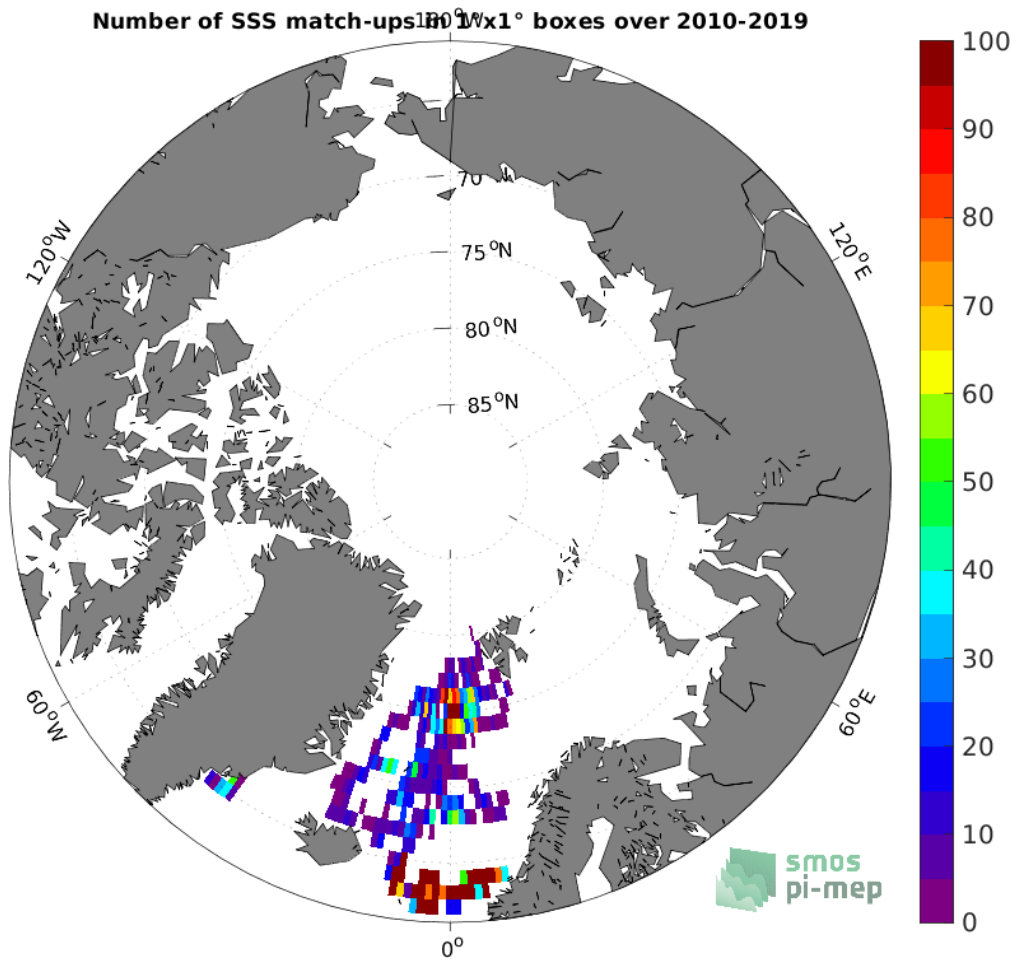
Figure 3: Number of SSS match-ups between Surface drifters SSS and the SMOS SSS L3 v8 - 9 Days (CATDS-CECOS-LOCEAN) SSS product for the Arctic Ocean Pi-MEP region over 1^\circ \times 1^\circ boxes and for the full satellite product period.
