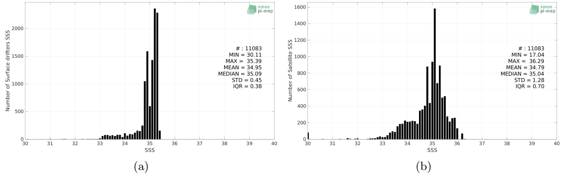
Figure 2: Histograms of SSS from Surface drifters (a) and SMOS SSS L3 v8 - 9 Days (CATDS-CECOS-LOCEAN) (b) considering all match-up pairs per bins of 0.1 over the Arctic Ocean Pi-MEP region and for the full satellite product period.
