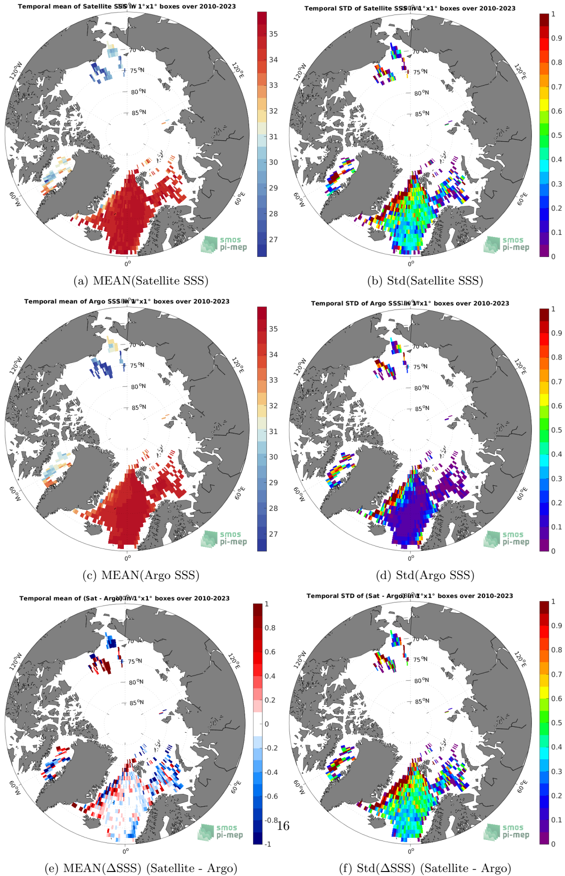
Figure 6: Temporal mean (left) and Std (right) of SSS from SMOS SSS L3 v8 - 9 Days (CATDS-CECOS-LOCEAN) (top), Argo (middle), and of \Delta SSS (Satellite - Argo). Only match-up pairs are used to generate these maps.
