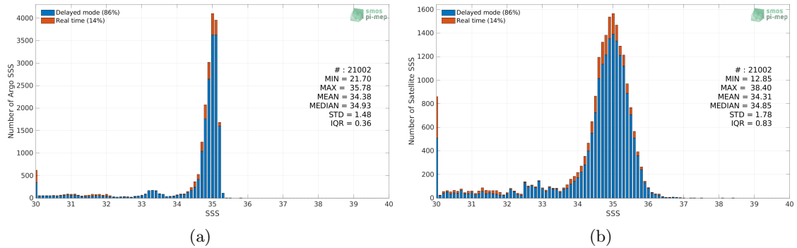
Figure 2: Histograms of SSS from Argo (a) and SMOS SSS L3 v8 - 9 Days (CATDS-CECOS-LOCEAN) (b) considering all match-up pairs per bins of 0.1 over the Arctic Ocean Pi-MEP region and for the full satellite product period.
