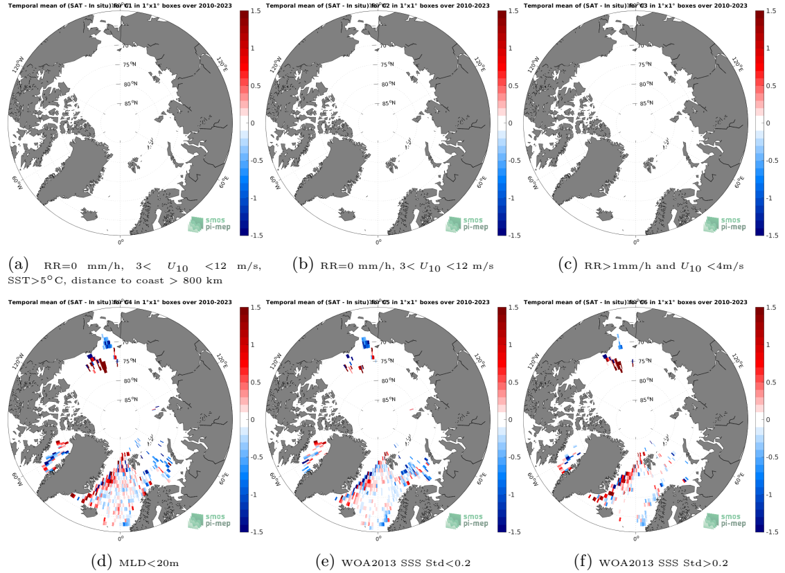
Figure 12: Temporal mean gridded over spatial boxes of size 1^{\circ}\times 1^{\circ} of \Delta\text{SSS} (SMOS SSS L3 v8 - 9 Days (CATDS-CECOS-LOCEAN) - Argo) for 6 different subdatasets corresponding to:RR=0 mm/h, 3 < U_{10} < 12 m/s, SST >5^{\circ}\text{C} , distance to coast > 800 km (a), RR=0 mm/h, 3 < U_{10} < 12 m/s (b), RR >1 mm/h and U_{10} < 4 m/s (c),MLD <20 m (d),WOA2013 SSS Std <0.2 (e),WOA2013 SSS Std >0.2 (f).
