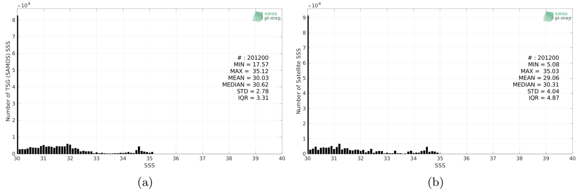
Figure 2: Histograms of SSS from TSG (SAMOS) (a) and SMOS SSS L3 v8 - 18 Days (CATDS-CECOS-LOCEAN) (b) considering all match-up pairs per bins of 0.1 over the Arctic Ocean Pi-MEP region and for the full satellite product period.
