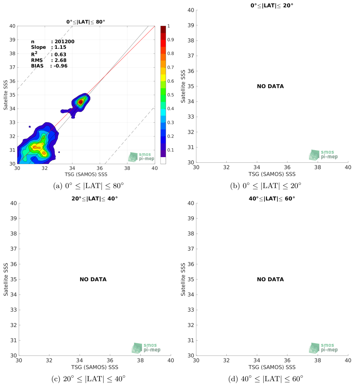
Figure 9: Contour maps of the concentration of SMOS SSS L3 v8 - 18 Days (CATDS-CECOS-LOCEAN) SSS (y-axis) versus TSG (SAMOS) SSS (x-axis) at match-up pairs for different latitude bands. For each plot, the red line shows x=y . The black thin and dashed lines indicate a linear fit through the data cloud and the \pm 95\% confidence levels, respectively. The number match-up pairs n , the slope and R^2 coefficient of the linear fit, the root mean square (RMS) and the mean bias between satellite and in situ data are indicated for each latitude band in each plots.
