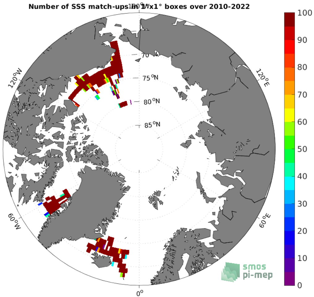
Figure 4: Number of SSS match-ups between TSG (SAMOS) SSS and the SMOS SSS L3 v8 - 18 Days (CATDS-CECOS-LOCEAN) SSS product for the Arctic Ocean Pi-MEP region over 1^\circ \times 1^\circ boxes and for the full satellite product period.
