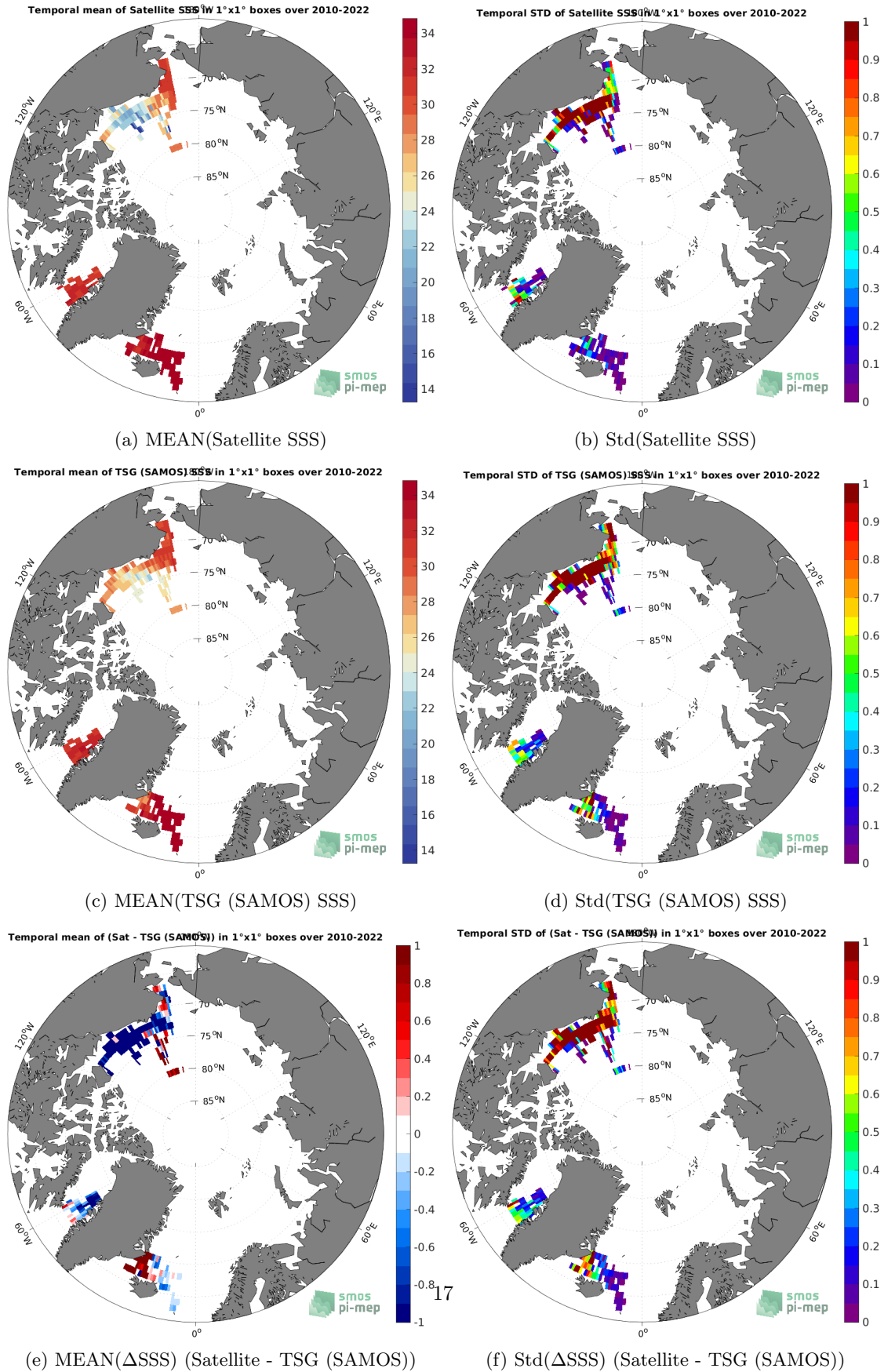
Figure 6: Temporal mean (left) and Std (right) of SSS from SMOS SSS L3 v8 - 18 Days (CATDS-CECOS-LOCEAN) (top), TSG (SAMOS) (middle), and of \Delta SSS (Satellite - TSG (SAMOS)). Only match-up pairs are used to generate these maps.
