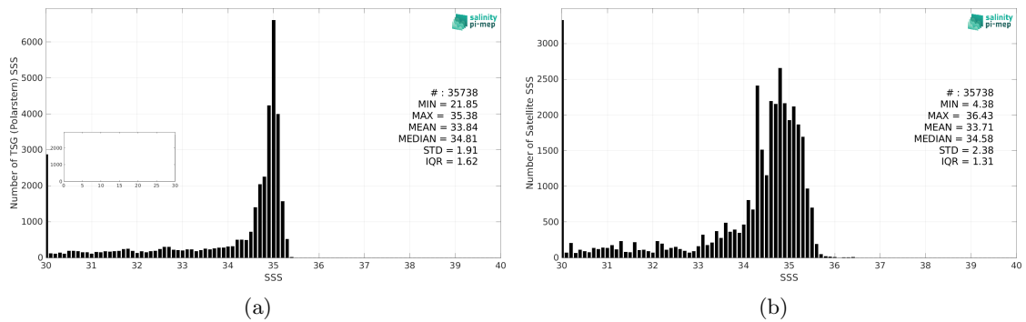
Figure 2: Histograms of SSS from TSG (Polarstern) (a) and SMOS SSS L3 v8 - 18 Days (CATDS-CEC-LOCEAN) (b) considering all match-up pairs per bins of 0.1 over the Arctic Ocean Pi-MEP region and for the full satellite product period.
