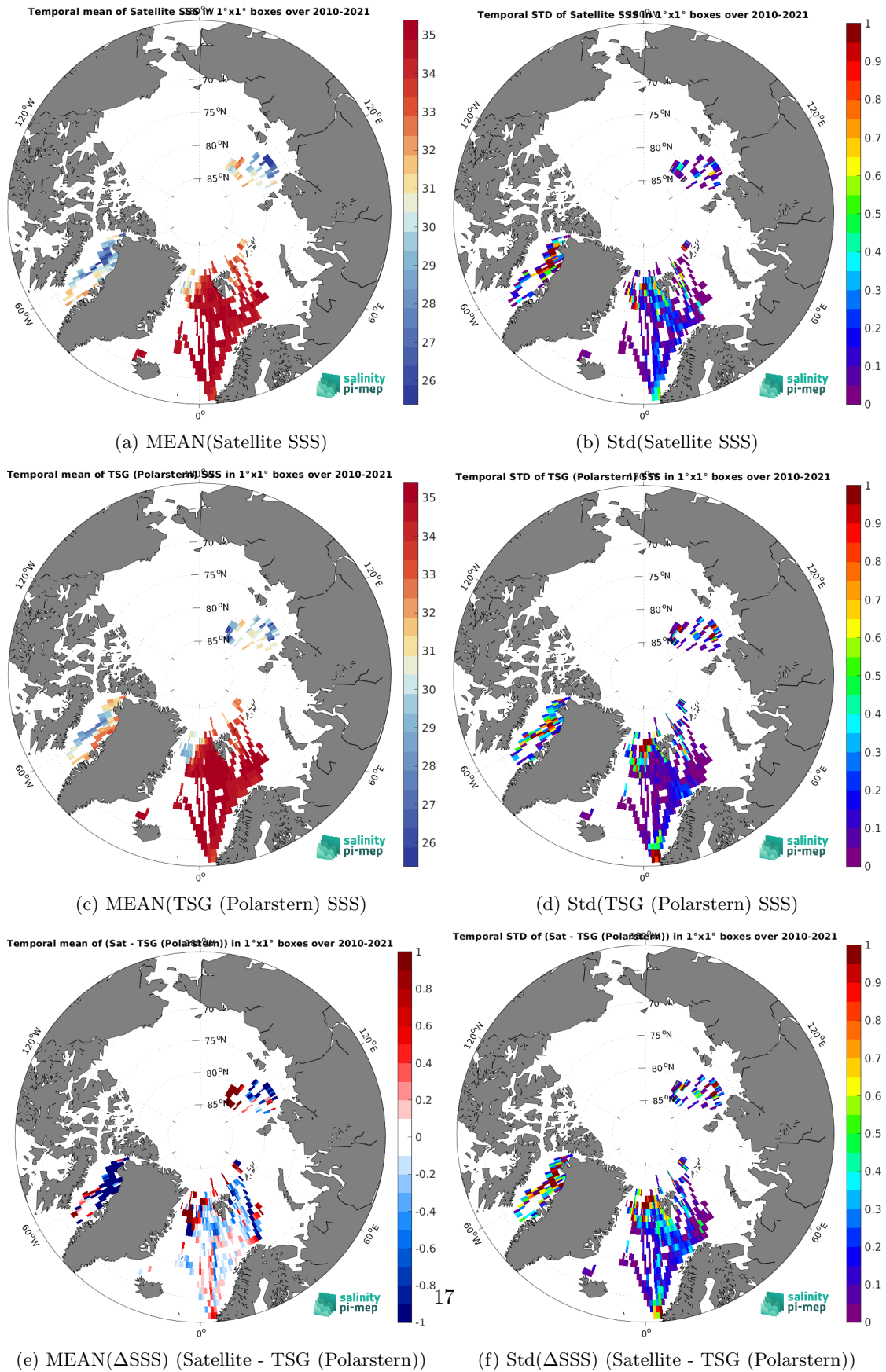
Figure 6: Temporal mean (left) and Std (right) of SSS from SMOS SSS L3 v8 - 18 Days (CATDS-CEC-LOCEAN) (top), TSG (Polarstern) (middle), and of \Delta SSS (Satellite - TSG (Polarstern)). Only match-up pairs are used to generate these maps.
