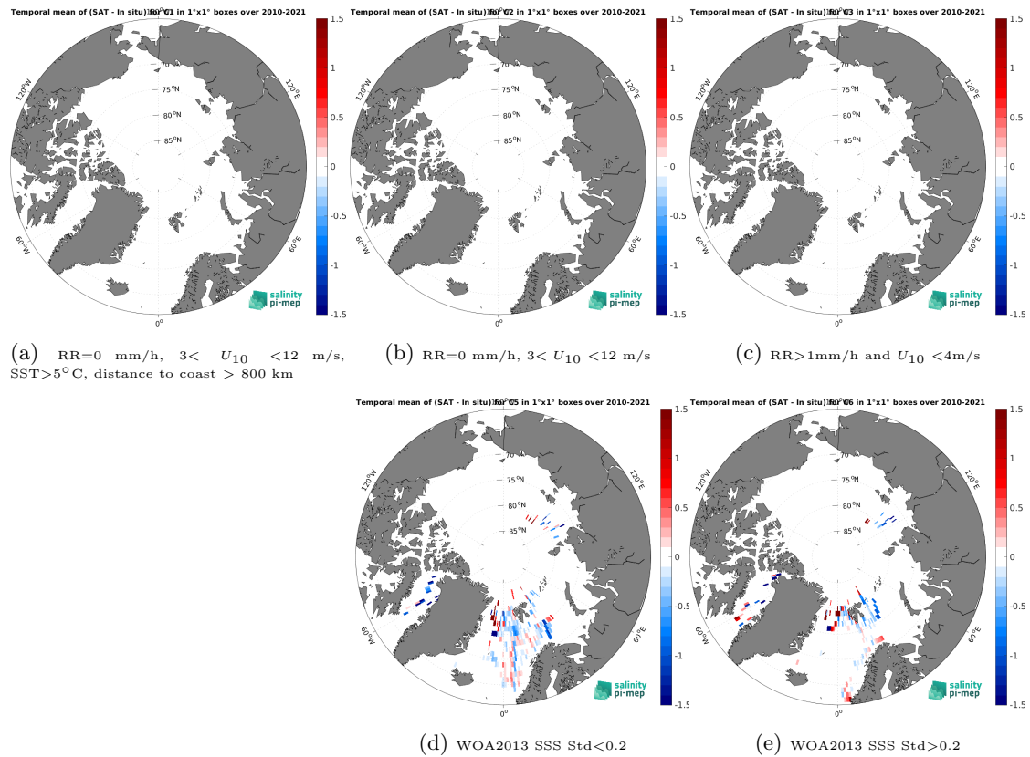
Figure 12: Temporal mean gridded over spatial boxes of size 1^{\circ}\times 1^{\circ} of \Delta\text{SSS} (SMOS SSS L3 v8 - 18 Days (CATDS-CEC-LOCEAN) - TSG (Polarstern)) for 5 different subdatasets corresponding to: RR=0 mm/h, 3 < U_{10} < 12 m/s, SST > 5^{\circ}\text{C} , distance to coast > 800 km (a), RR=0 mm/h, 3 < U_{10} < 12 m/s (b), RR > 1 mm/h and U_{10} < 4 m/s (c), WOA2013 SSS Std < 0.2 (d), WOA2013 SSS Std > 0.2 (e).
