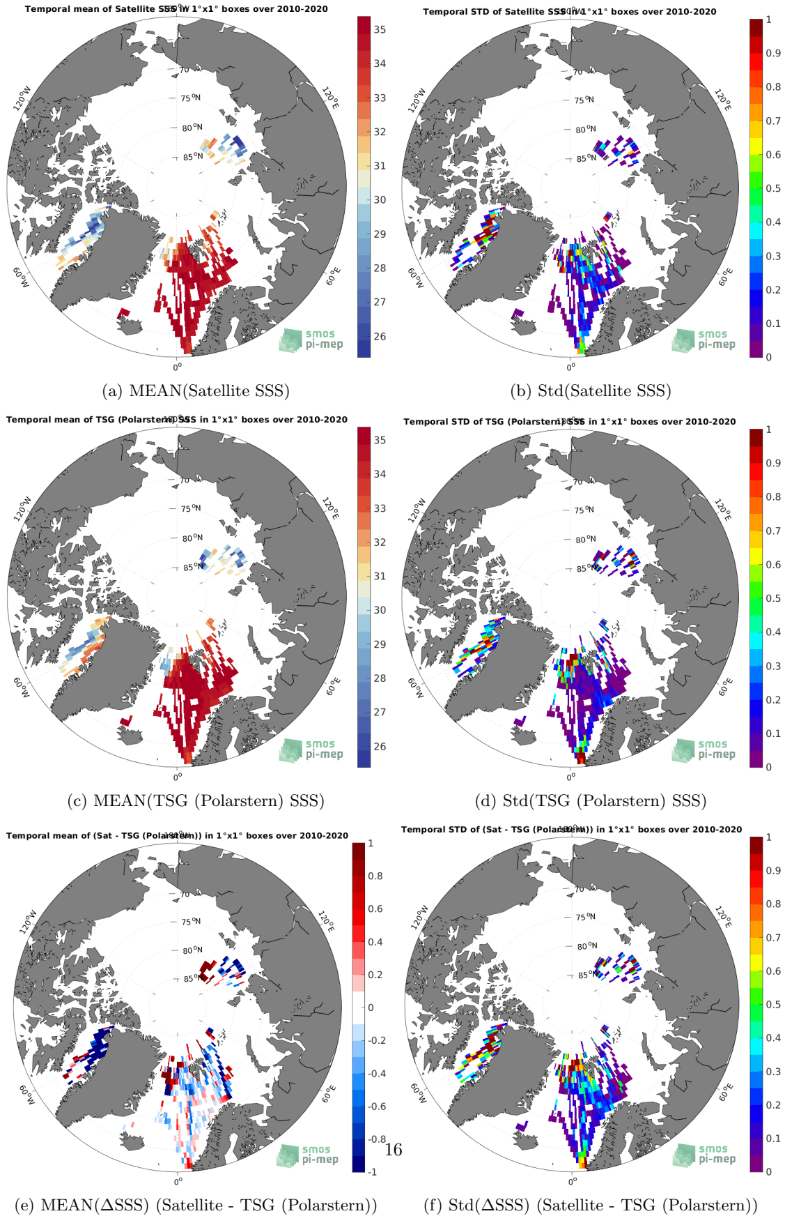
Figure 6: Temporal mean (left) and Std (right) of SSS from SMOS SSS L3 v8 - 18 Days (CATDS-CECOS-LOCEAN) (top), TSG (Polarstern) (middle), and of \Delta SSS (Satellite - TSG (Polarstern)). Only match-up pairs are used to generate these maps.
