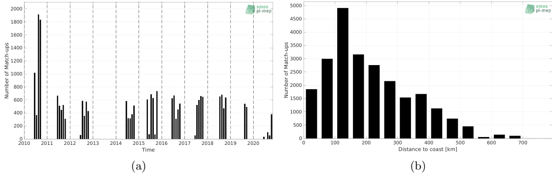
Figure 1: Number of match-ups between TSG (Polarstern) and SMOS SSS L3 v8 - 18 Days (CATDS-CECOS-LOCEAN) SSS as a function of time (a) and as function of the distance to coast (b) over the Arctic Ocean Pi-MEP region and for the full satellite product period.
