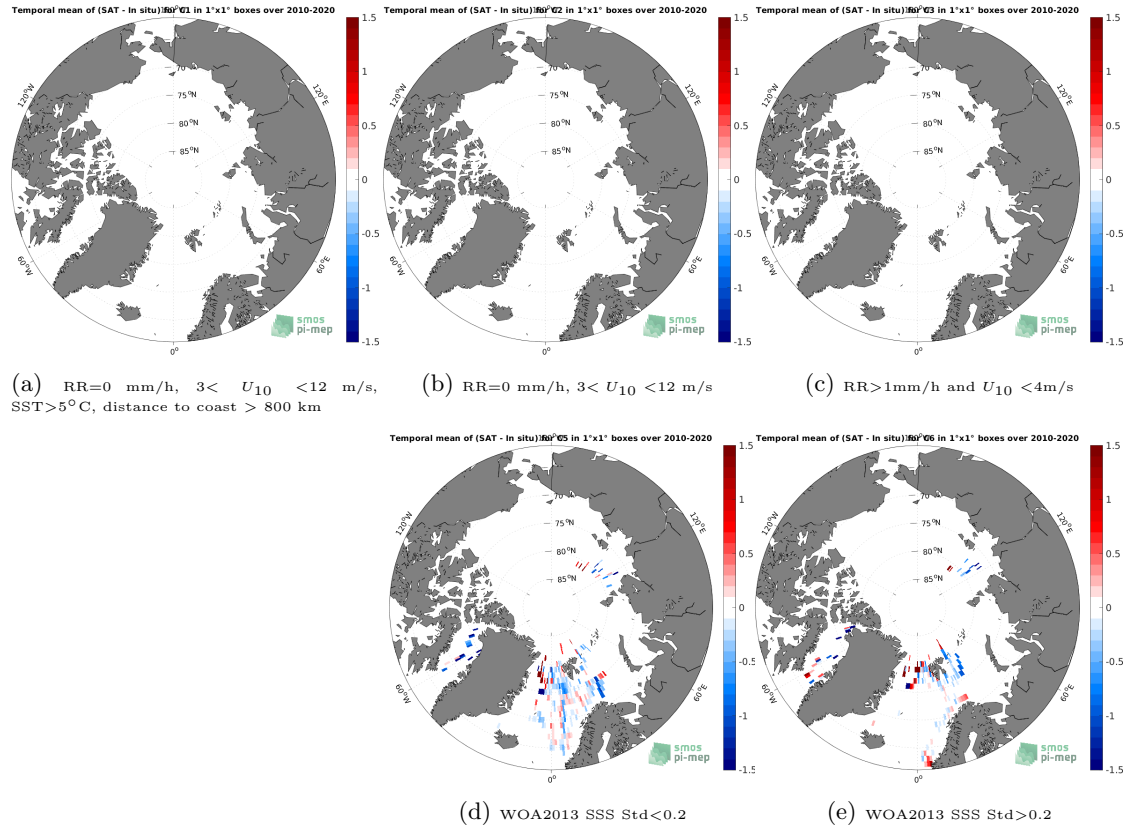
Figure 12: Temporal mean gridded over spatial boxes of size 1^{\circ}\times 1^{\circ} of \Delta\text{SSS} (SMOS SSS L3 v8 - 18 Days (CATDS-CECOS-LOCEAN) - TSG (Polarstern)) for 5 different subdatasets corresponding to:RR=0 mm/h, 3 < U_{10} < 12 m/s, SST >5^{\circ}\text{C} , distance to coast > 800 km (a), RR=0 mm/h, 3 < U_{10} < 12 m/s (b), RR >1 mm/h and U_{10} < 4 m/s (c), WOA2013 SSS Std <0.2 (d), WOA2013 SSS Std >0.2 (e).
