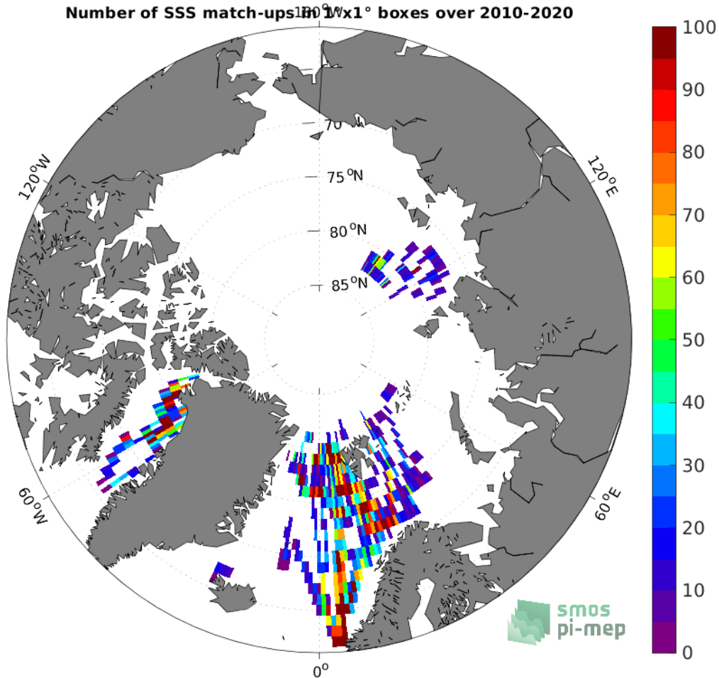
Figure 4: Number of SSS match-ups between TSG (Polarstern) SSS and the SMOS SSS L3 v8 - 18 Days (CATDS-CECOS-LOCEAN) SSS product for the Arctic Ocean Pi-MEP region over 1^\circ \times 1^\circ boxes and for the full satellite product period.
