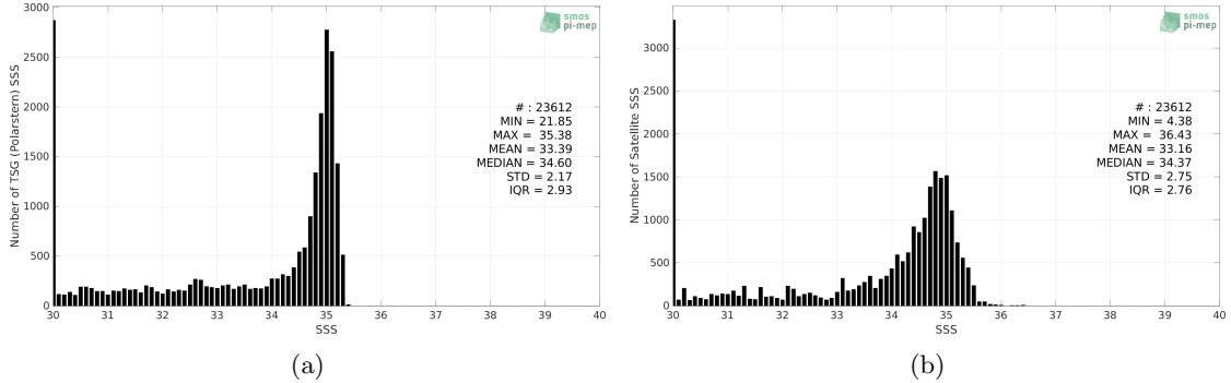
Figure 2: Histograms of SSS from TSG (Polarstern) (a) and SMOS SSS L3 v8 - 18 Days (CATDS-CECOS-LOCEAN) (b) considering all match-up pairs per bins of 0.1 over the Arctic Ocean Pi-MEP region and for the full satellite product period.
