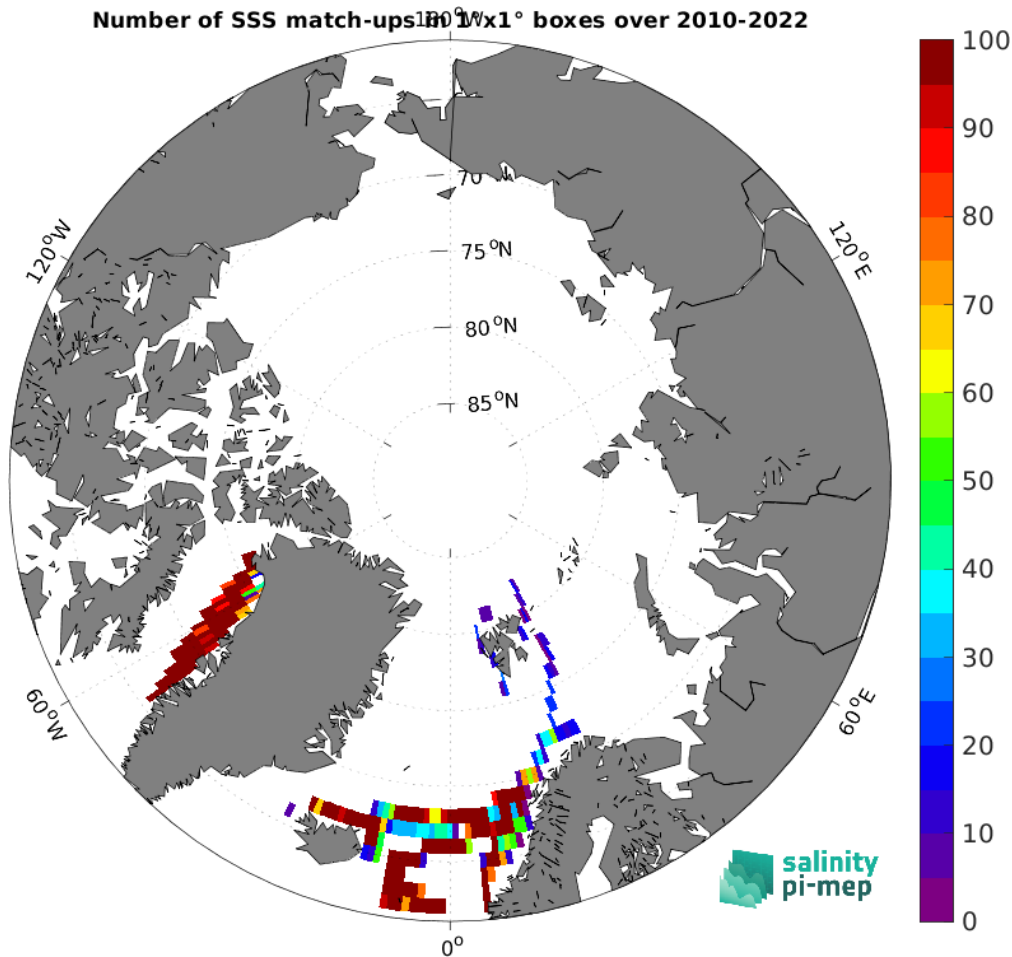
Figure 4: Number of SSS match-ups between TSG (LEGOS-DM) SSS and the SMOS SSS L3 v8 - 18 Days (CATDS-CEC-LOCEAN) SSS product for the Arctic Ocean Pi-MEP region over 1^\circ \times 1^\circ boxes and for the full satellite product period.
