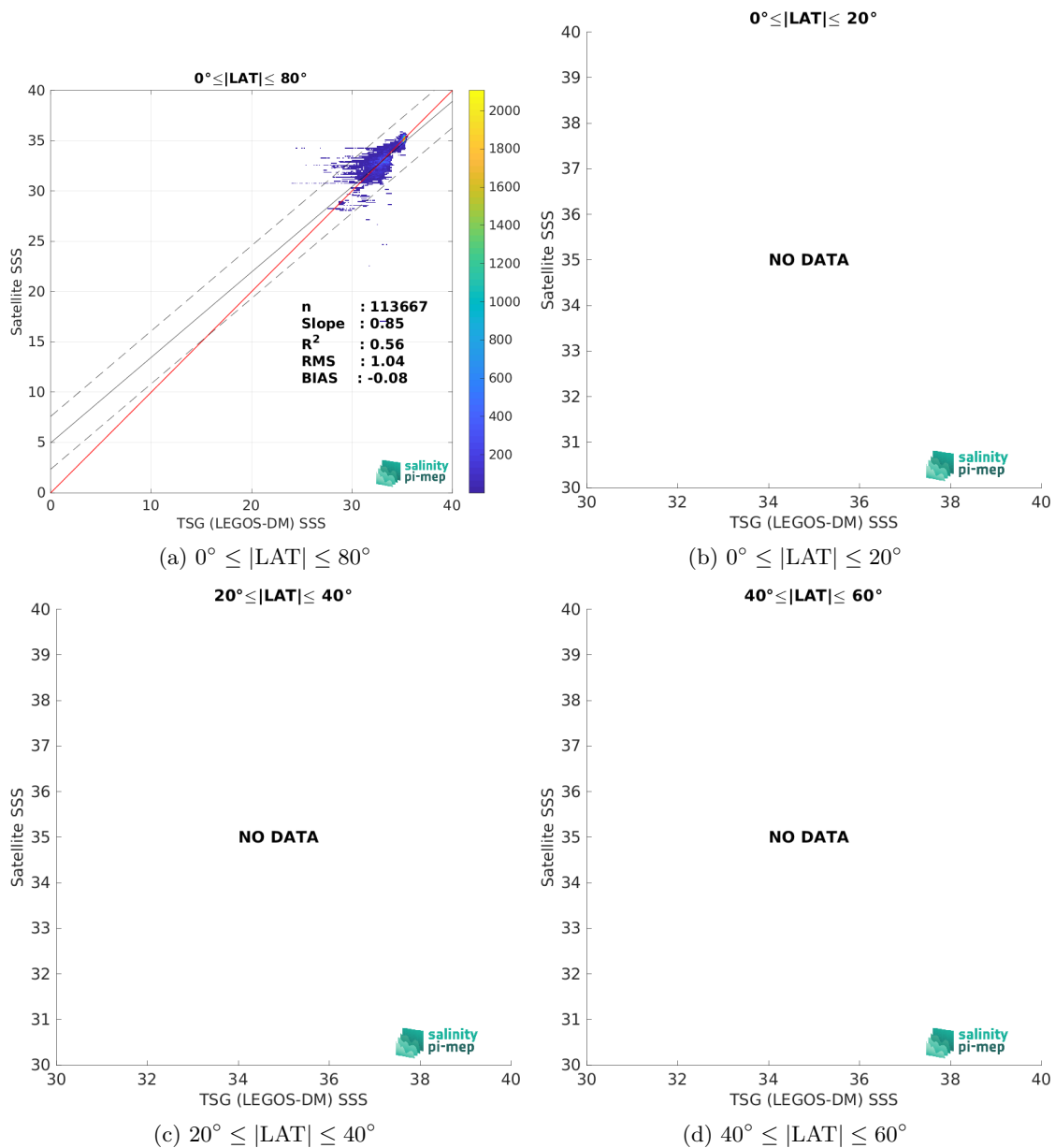
Figure 9: Contour maps of the concentration of SMOS SSS L3 v8 - 18 Days (CATDS-CEC-LOCEAN) SSS (y-axis) versus TSG (LEGOS-DM) SSS (x-axis) at match-up pairs for different latitude bands. For each plot, the red line shows x=y . The black thin and dashed lines indicate a linear fit through the data cloud and the \pm 95\% confidence levels, respectively. The number match-up pairs n , the slope and R^2 coefficient of the linear fit, the root mean square (RMS) and the mean bias between satellite and in situ data are indicated for each latitude band in each plots.
