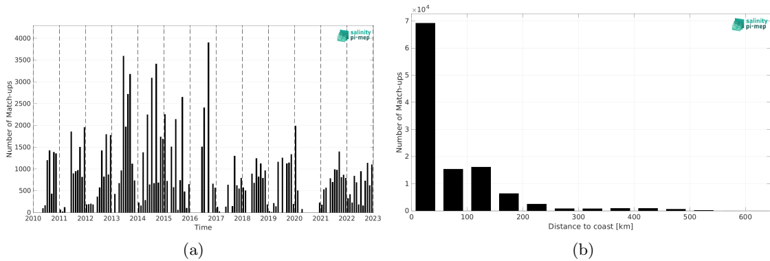
Figure 1: Number of match-ups between TSG (LEGOS-DM) and SMOS SSS L3 v8 - 18 Days (CATDS-CEC-LOCEAN) SSS as a function of time (a) and as function of the distance to coast (b) over the Arctic Ocean Pi-MEP region and for the full satellite product period.
