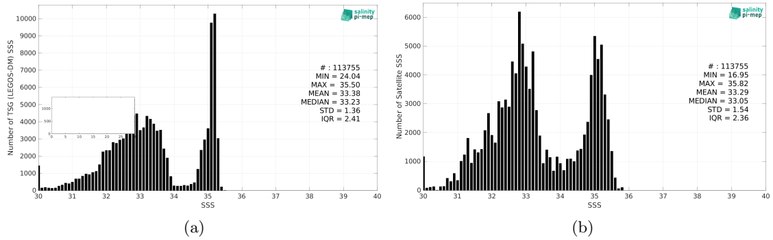
Figure 2: Histograms of SSS from TSG (LEGOS-DM) (a) and SMOS SSS L3 v8 - 18 Days (CATDS-CEC-LOCEAN) (b) considering all match-up pairs per bins of 0.1 over the Arctic Ocean Pi-MEP region and for the full satellite product period.
