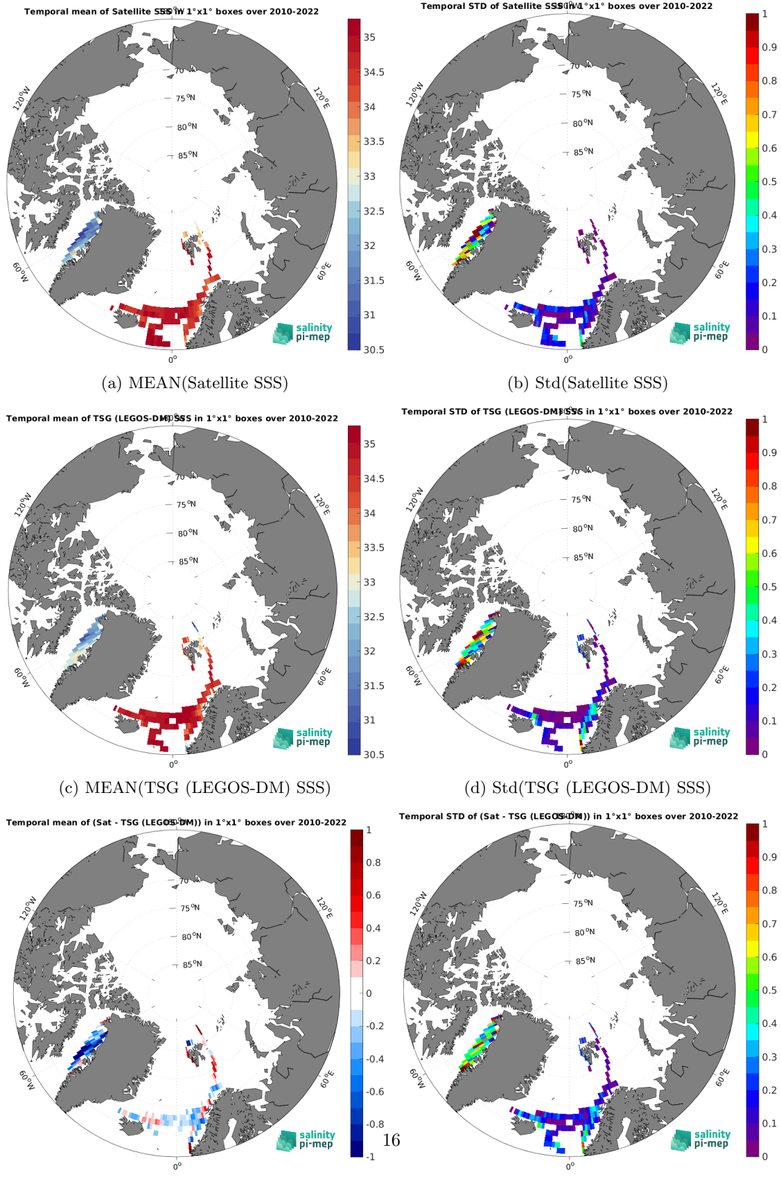
(e) MEAN( \Delta SSS) (Satellite - TSG (LEGOS-DM)) (f) Std( \Delta SSS) (Satellite - TSG (LEGOS-DM)) Figure 6: Temporal mean (left) and Std (right) of SSS from SMOS SSS L3 v8 - 18 Days (CATDS-CEC-LOCEAN) (top), TSG (LEGOS-DM) (middle), and of \Delta SSS (Satellite - TSG (LEGOS-DM)). Only match-up pairs are used to generate these maps.
