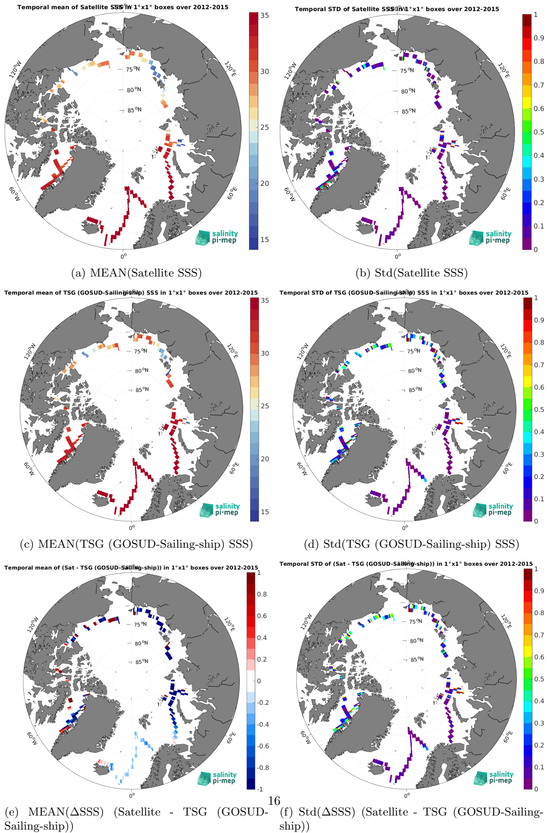
Figure 6: Temporal mean (left) and Std (right) of SSS from SMOS SSS L3 v8 - 18 Days (CATDS-CEC-LOCEAN) (top), TSG (GOSUD-Sailing-ship) (middle), and of \Delta SSS (Satellite - TSG (GOSUD-Sailing-ship)). Only match-up pairs are used to generate these maps.
