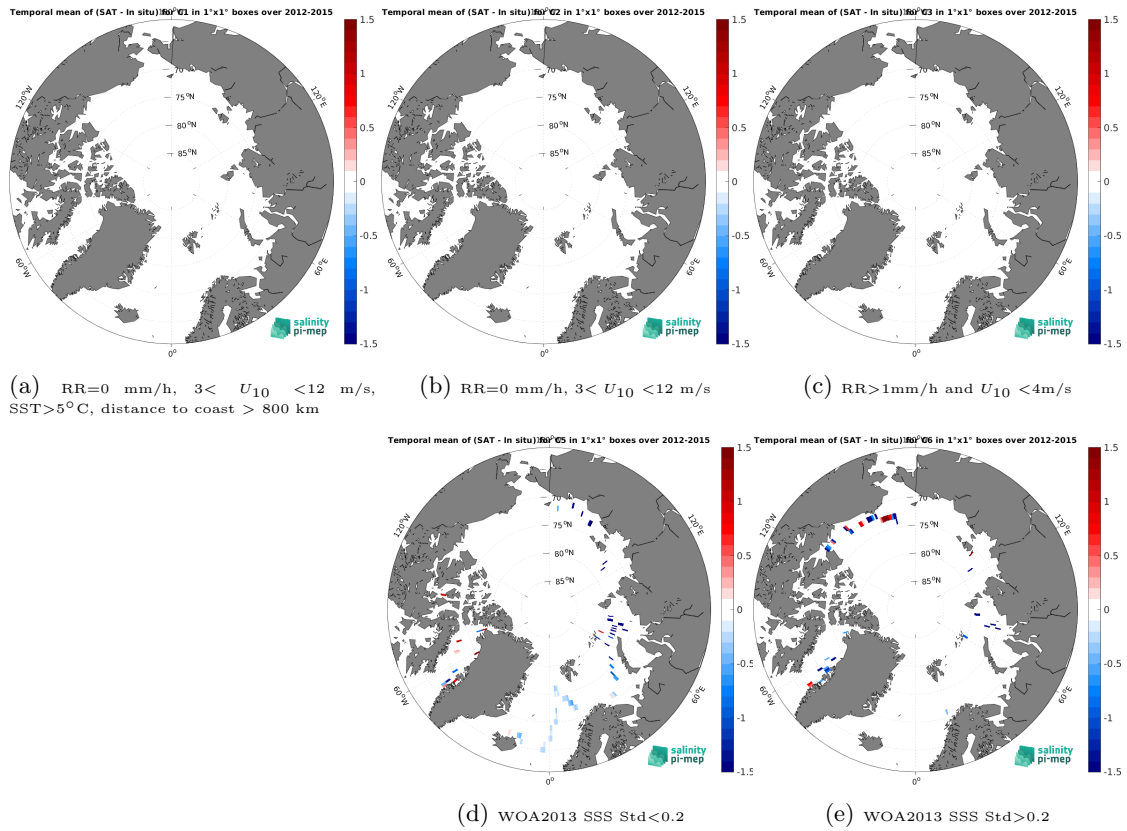
Figure 12: Temporal mean gridded over spatial boxes of size 1^\circ \times 1^\circ of \Delta SSS (SMOS SSS L3 v8 - 18 Days (CATDS-CEC-LOCEAN) - TSG (GOSUD-Sailing-ship)) for 5 different subdatasets corresponding to: RR=0 mm/h, 3 < U_{10} < 12 m/s, SST>5°C, distance to coast > 800 km (a), RR=0 mm/h, 3 < U_{10} < 12 m/s (b), RR>1mm/h and U_{10} < 4 m/s (c), WOA2013 SSS Std<0.2 (d), WOA2013 SSS Std>0.2 (e).
