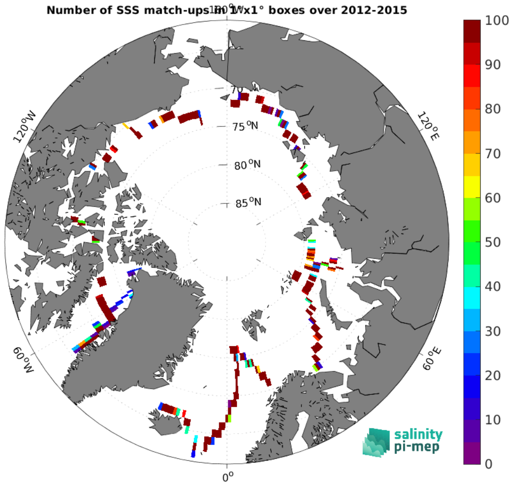
Figure 4: Number of SSS match-ups between TSG (GOSUD-Sailing-ship) SSS and the SMOS SSS L3 v8 - 18 Days (CATDS-CEC-LOCEAN) SSS product for the Arctic Ocean Pi-MEP region over 1^\circ \times 1^\circ boxes and for the full satellite product period.
