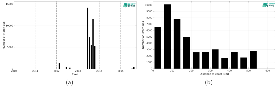
Figure 1: Number of match-ups between TSG (GOSUD-Sailing-ship) and SMOS SSS L3 v8 - 18 Days (CATDS-CEC-LOCEAN) SSS as a function of time (a) and as function of the distance to coast (b) over the Arctic Ocean Pi-MEP region and for the full satellite product period.
