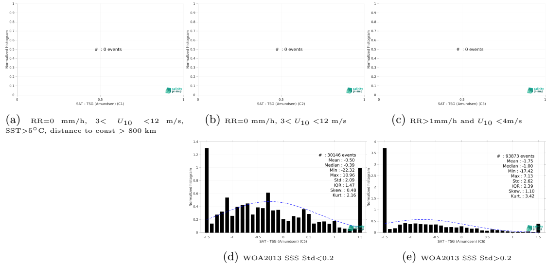
Figure 13: Normalized histogram of \Delta SSS (SMOS SSS L3 v8 - 18 Days (CATDS-CEC-LOCEAN) - TSG (Amundsen)) for 5 different subdatasets corresponding to: RR=0 mm/h, 3 < U_{10} < 12 m/s, SST > 5°C, distance to coast > 800 km (a), RR=0 mm/h, 3 < U_{10} < 12 m/s (b), RR > 1mm/h and U_{10} < 4 m/s (c), WOA2013 SSS Std < 0.2 (d), WOA2013 SSS Std > 0.2 (e).
