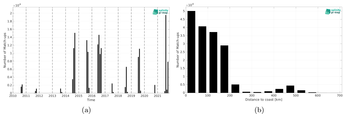
Figure 1: Number of match-ups between TSG (Amundsen) and SMOS SSS L3 v8 - 18 Days (CATDS-CEC-LOCEAN) SSS as a function of time (a) and as function of the distance to coast (b) over the Arctic Ocean Pi-MEP region and for the full satellite product period.
