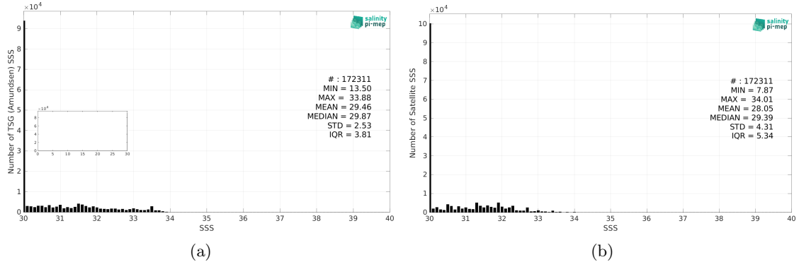
Figure 2: Histograms of SSS from TSG (Amundsen) (a) and SMOS SSS L3 v8 - 18 Days (CATDS-CEC-LOCEAN) (b) considering all match-up pairs per bins of 0.1 over the Arctic Ocean Pi-MEP region and for the full satellite product period.
