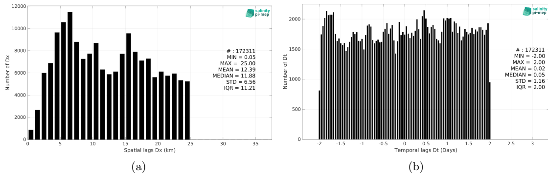
Figure 5: Histograms of the spatial (a) and temporal (b) lags between the location/time of the TSG (Amundsen) measurement and the date of the corresponding SMOS SSS L3 v8 - 18 Days (CATDS-CEC-LOCEAN) SSS pixel.
