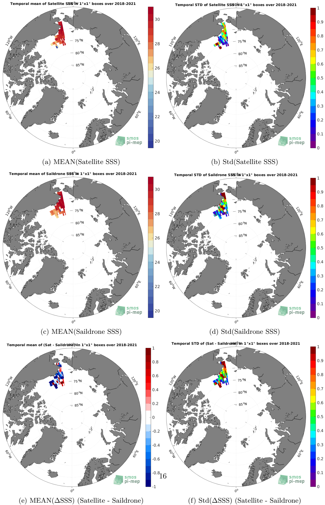
Figure 6: Temporal mean (left) and Std (right) of SSS from SMOS SSS L3 v8 - 18 Days (CATDS-CECOS-LOCEAN) (top), Saildrone (middle), and of \Delta SSS (Satellite - Saildrone). Only match-pairs are used to generate these maps.
