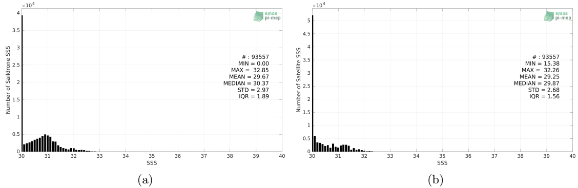
Figure 2: Histograms of SSS from Saildrone (a) and SMOS SSS L3 v8 - 18 Days (CATDS-CECOS-LOCEAN) (b) considering all match-up pairs per bins of 0.1 over the Arctic Ocean Pi-MEP region and for the full satellite product period.
