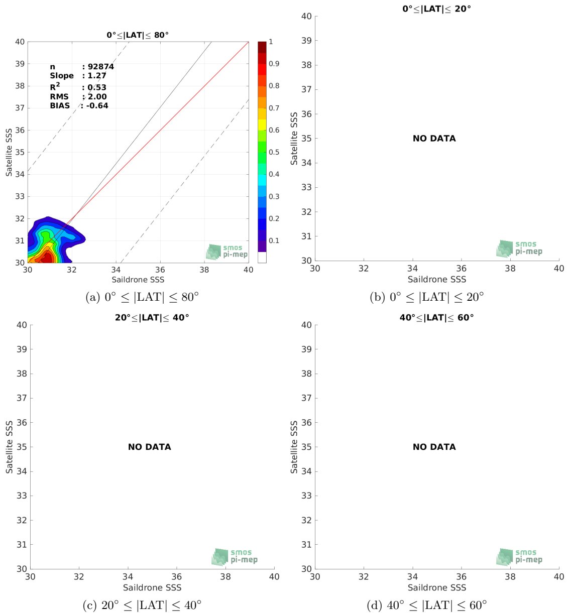
Figure 9: Contour maps of the concentration of SMOS SSS L3 v8 - 18 Days (CATDS-CECOS-LOCEAN) SSS (y-axis) versus Saildrone SSS (x-axis) at match-up pairs for different latitude bands. For each plot, the red line shows x=y . The black thin and dashed lines indicate a linear fit through the data cloud and the \pm 95\% confidence levels, respectively. The number match-up pairs n , the slope and R^2 coefficient of the linear fit, the root mean square (RMS) and the mean bias between satellite and in situ data are indicated for each latitude band in each plots.
