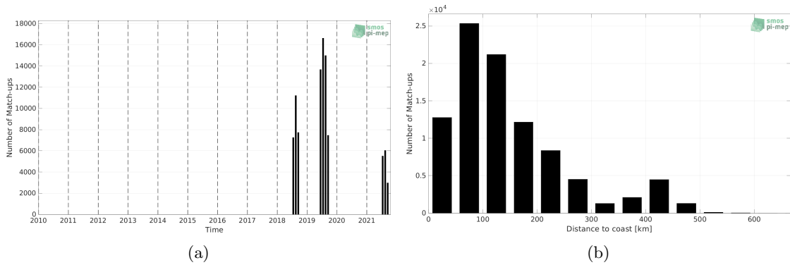
Figure 1: Number of match-ups between Saildrone and SMOS SSS L3 v8 - 18 Days (CATDS-CECOS-LOCEAN) SSS as a function of time (a) and as function of the distance to coast (b) over the Arctic Ocean Pi-MEP region and for the full satellite product period.
