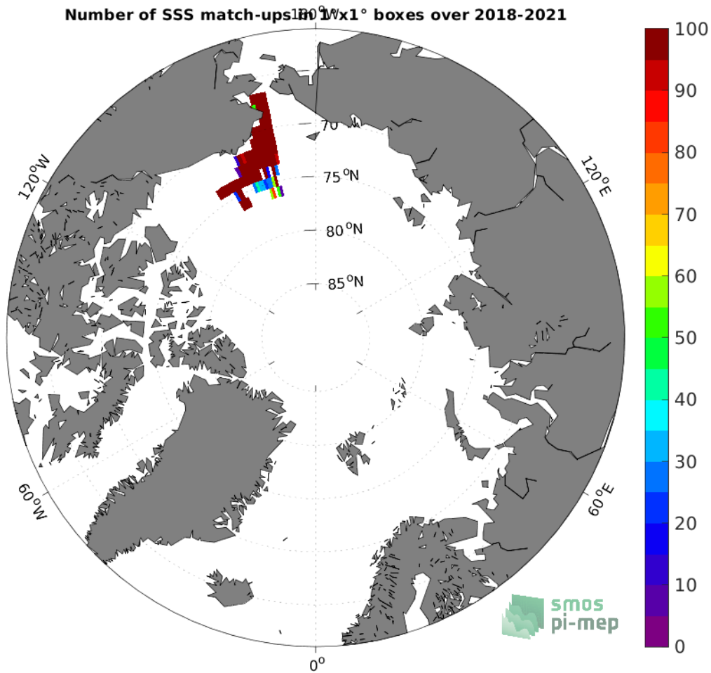
Figure 4: Number of SSS match-ups between Sairdrone SSS and the SMOS SSS L3 v8 - 18 Days (CATDS-CECOS-LOCEAN) SSS product for the Arctic Ocean Pi-MEP region over 1^\circ \times 1^\circ boxes and for the full satellite product period.
