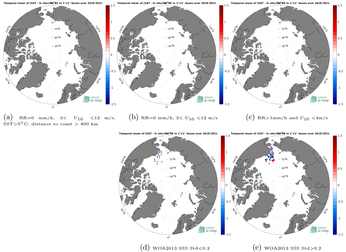
Figure 12: Temporal mean gridded over spatial boxes of size 1^{\circ}\times 1^{\circ} of \Delta\text{SSS} (SMOS SSS L3 v8 - 18 Days (CATDS-CECOS-LOCEAN) - Saildrone) for 5 different subdatasets corresponding to: RR=0 mm/h, 3 < U_{10} < 12 m/s, SST > 5^{\circ}\text{C} , distance to coast > 800 km (a), RR=0 mm/h, 3 < U_{10} < 12 m/s (b), RR > 1 mm/h and U_{10} < 4 m/s (c), WOA2013 SSS Std < 0.2 (d), WOA2013 SSS Std > 0.2 (e).
