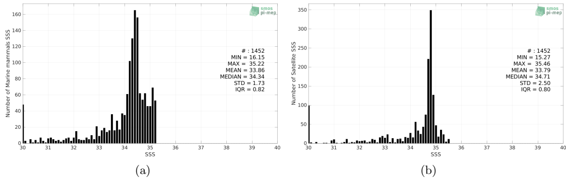
Figure 2: Histograms of SSS from Marine mammals (a) and SMOS SSS L3 v8 - 18 Days (CATDS-CECOS-LOCEAN) (b) considering all match-up pairs per bins of 0.1 over the Arctic Ocean Pi-MEP region and for the full satellite product period.
