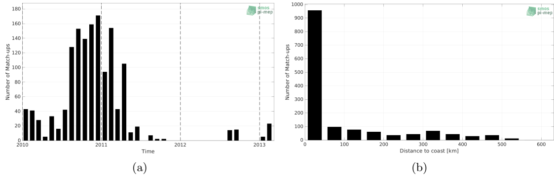
Figure 1: Number of match-ups between Marine mammals and SMOS SSS L3 v8 - 18 Days (CATDS-CECOS-LOCEAN) SSS as a function of time (a) and as function of the distance to coast (b) over the Arctic Ocean Pi-MEP region and for the full satellite product period.
