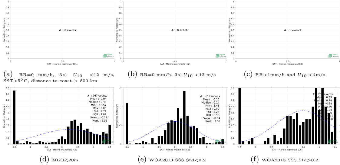
Figure 13: Normalized histogram of \Delta\text{SSS} (SMOS SSS L3 v8 - 18 Days (CATDS-CECOS-LOCEAN) - Marine mammals) for 6 different subdatasets corresponding to: RR=0 mm/h, 3 < U_{10} < 12 m/s, SST > 5^\circ\text{C} , distance to coast > 800 km (a), RR=0 mm/h, 3 < U_{10} < 12 m/s (b), RR > 1\text{mm/h} and U_{10} < 4\text{m/s} (c), MLD < 20\text{m} (d), WOA2013 SSS Std < 0.2 (e), WOA2013 SSS Std > 0.2 (f).
