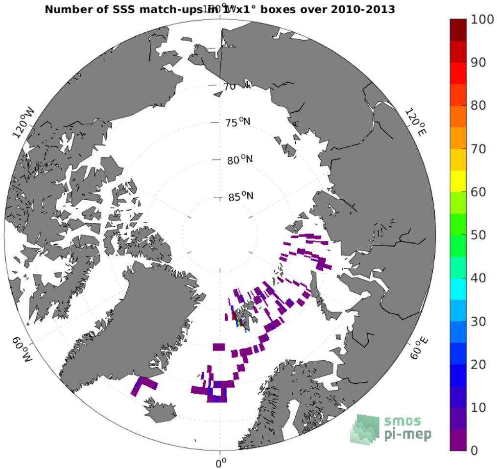
Figure 4: Number of SSS match-ups between Marine mammals SSS and the SMOS SSS L3 v8 - 18 Days (CATDS-CECOS-LOCEAN) SSS product for the Arctic Ocean Pi-MEP region over 1^\circ \times 1^\circ boxes and for the full satellite product period.
