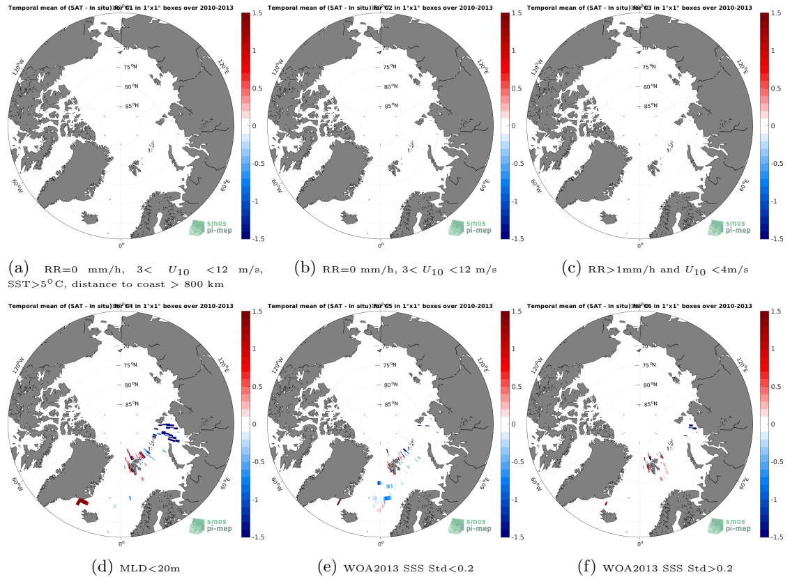
Figure 12: Temporal mean gridded over spatial boxes of size 1^{\circ}\times 1^{\circ} of \Delta\text{SSS} (SMOS SSS L3 v8 - 18 Days (CATDS-CECOS-LOCEAN) - Marine mammals) for 6 different subdatasets corresponding to:RR=0 mm/h, 3 < U_{10} < 12 m/s, SST > 5^{\circ}\text{C} , distance to coast > 800 km (a), RR=0 mm/h, 3 < U_{10} < 12 m/s (b), RR > 1 mm/h and U_{10} < 4 m/s (c),MLD < 20\text{m} (d),WOA2013 SSS Std < 0.2 (e),WOA2013 SSS Std > 0.2 (f).
